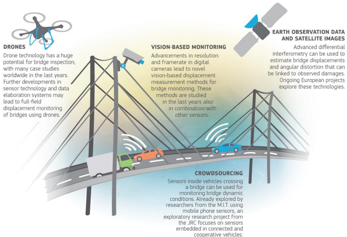
Figure 6. Promising bridge SHM methods
