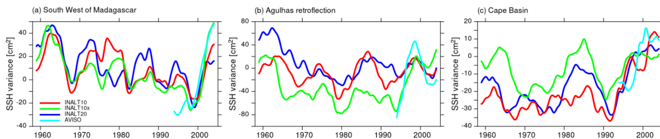
Figure 5. Timeseries of SSH variance anomalies to the 1995-2005 mean [in cm^2 ] computed in a 5 years running window based on 5-daily averages for the three different regions indicated in Fig. 3(f) from the nested configurations INALT20 (blue) INALT10 (red), INALT10x (green) and from AVISO-satellite altimetry (light blue). The curves are interannually filtered. For mean values and correlations see Tables 4 and 5, respectively.
