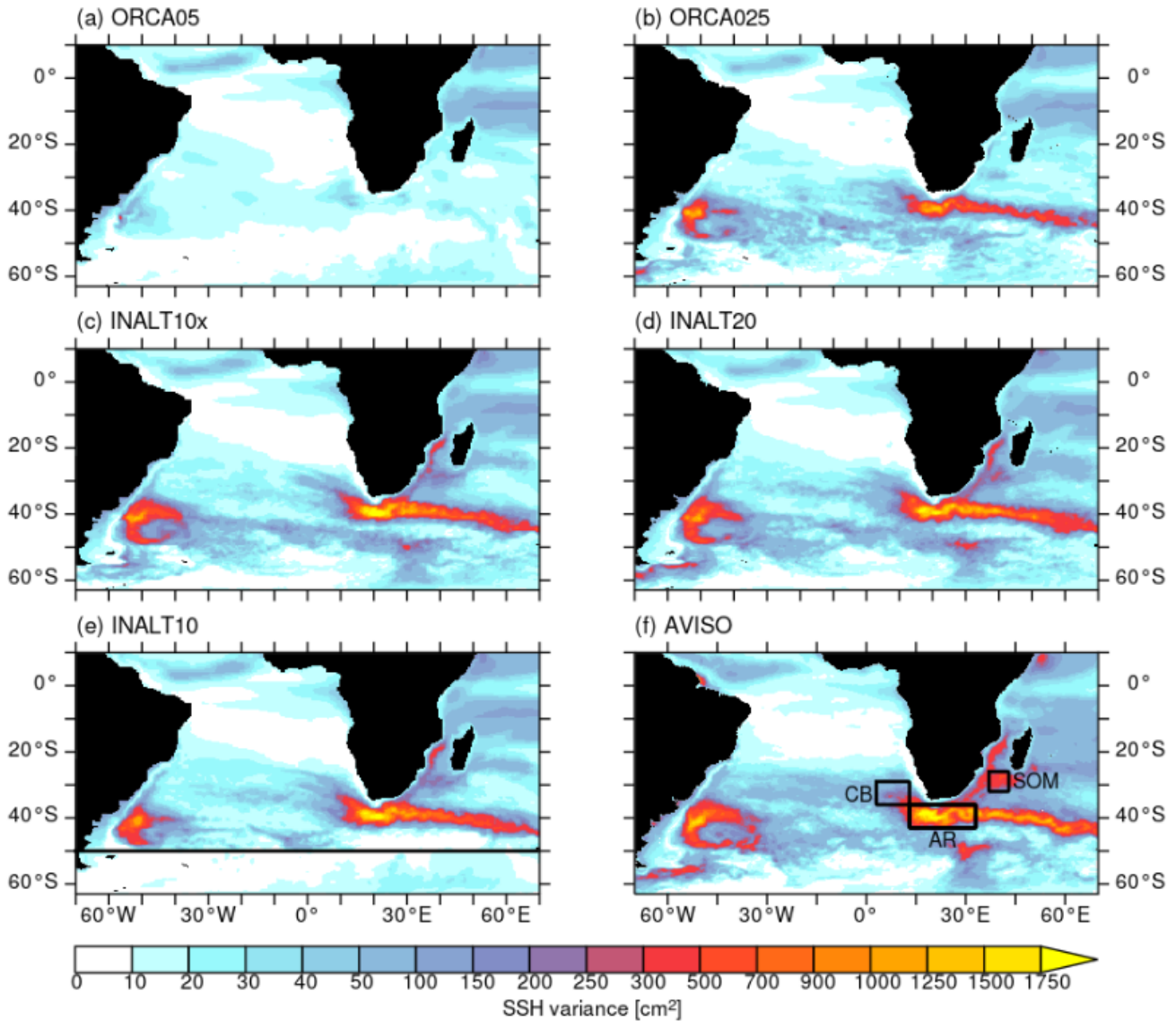
Figure 3. SSH variance [in cm^2 ] for the period 2000-2009 based on 5-day averages from (f) satellite altimetry data (AVISO) compared to the hindcast experiments in the different configurations (a) ORCA05, (b) ORCA025 (based on monthly averages), (c) INALT10x, (d) INALT20 and (e) INALT10. The horizontal line in (e) at 50° S indicates the southern boundary of the nested region in INALT10; the boxes in (f) mark the areas used for time series analyses (see Fig. 5). Note: the discrepancy in the temporal resolution for ORCA025 does not alter the findings (not shown).
