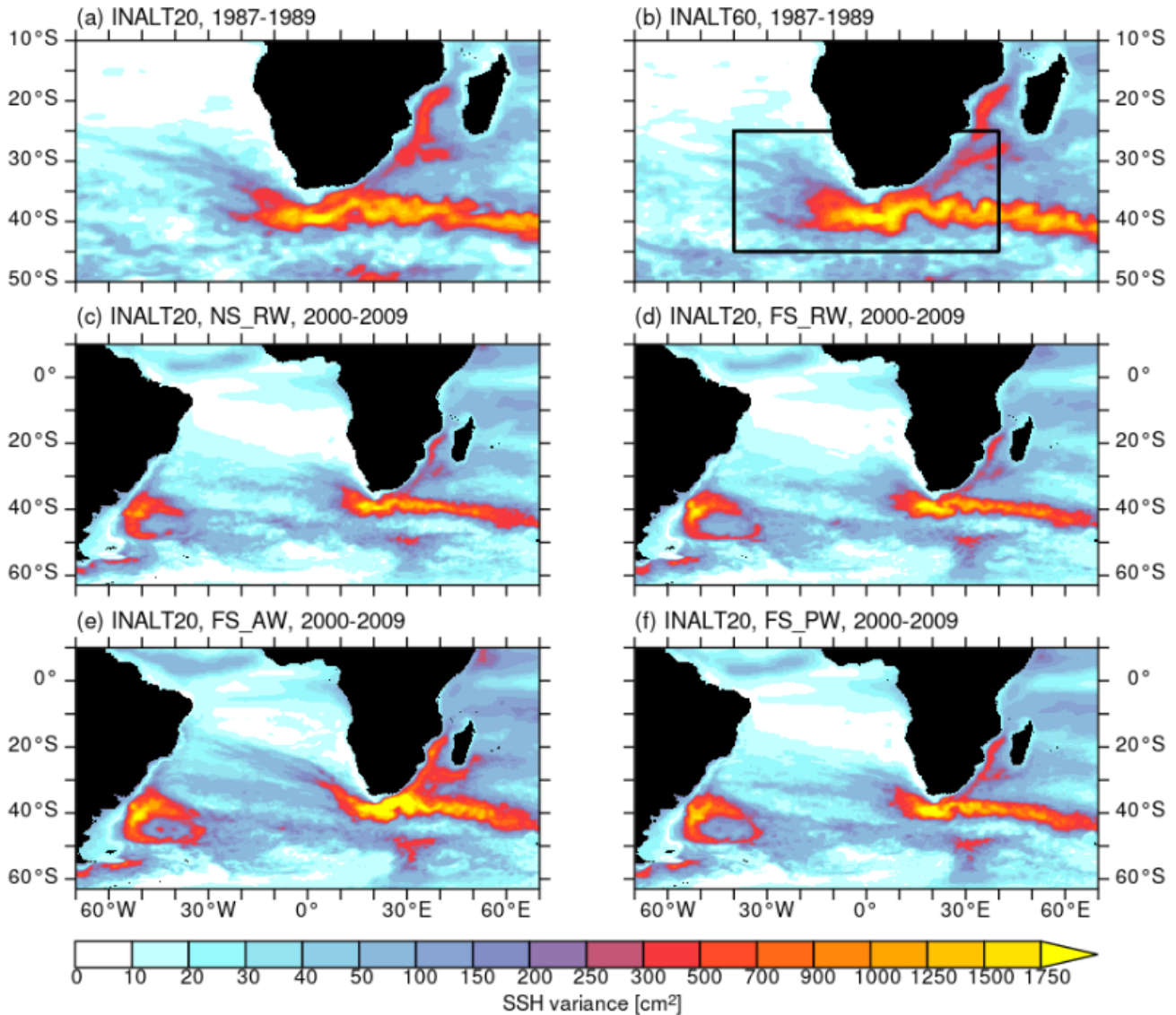
Figure 4. SSH variance [in cm^2 ] for the period 1987 to 1989 from the spin-up experiments in (a) INALT20 and (b) INALT60 based on 5-day averages; The black box in (b) marks the region of the secondary 1/60° nest in INALT60. (c to f) give the SSH variance [in cm^2 ] for the period 2000-2009 based on 5-day averages from the different sensitivity experiments in INALT20: (c) no slip, relative winds, (d) free slip, relative winds, (e) free slip, absolute winds, (f) free slip, partial winds.
