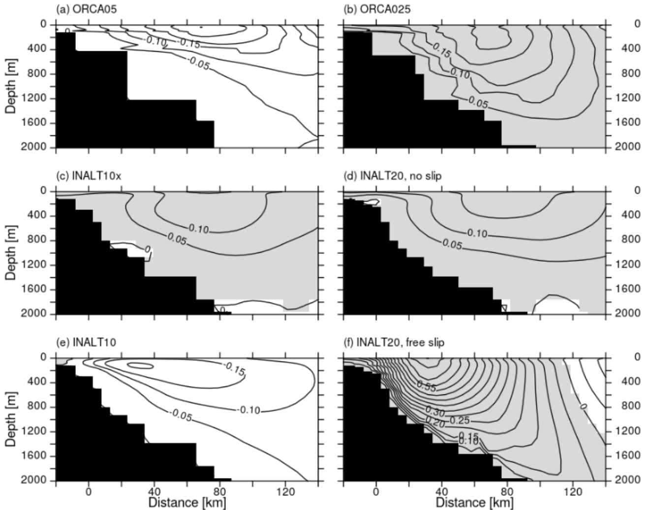
Figure 9. Mean (2000-2009) MC structure at 41^\circ S from ORCA05 (a), ORCA025 (b), INALT10x (c), INALT20 NS_RW (d), INALT10 (e) and INALT20 FS_RW (f). Note that southwestward/negative velocities are shaded in white, northeastward/positive in grey, contoured are intervals of 5 \text{ cm s}^{-1}
