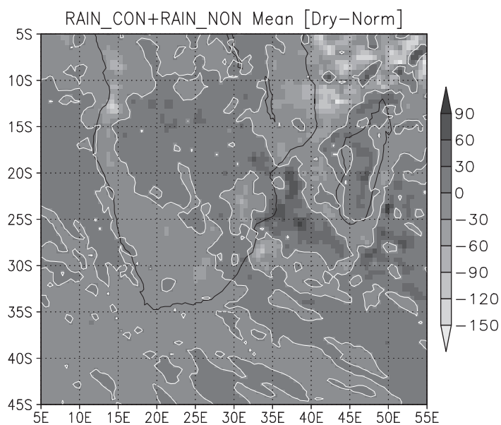
Fig. 3: Nov-Feb rainfall anomalies forced by a dry soil.
