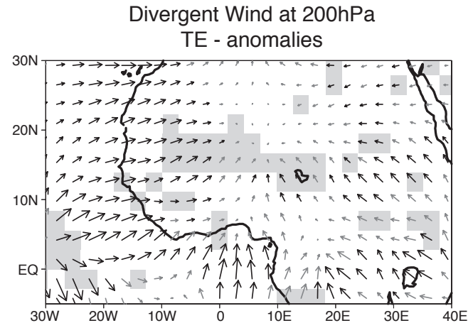
Fig. 4: Simulated monthly mean anomalies (August) for horizontal divergent component of the atmospheric circulation at 200hPa for TE-. Shadings for the vertical velocity anomalies significant at p=0.05 according to the Student's t -test, bold vectors for horizontal components significance.
