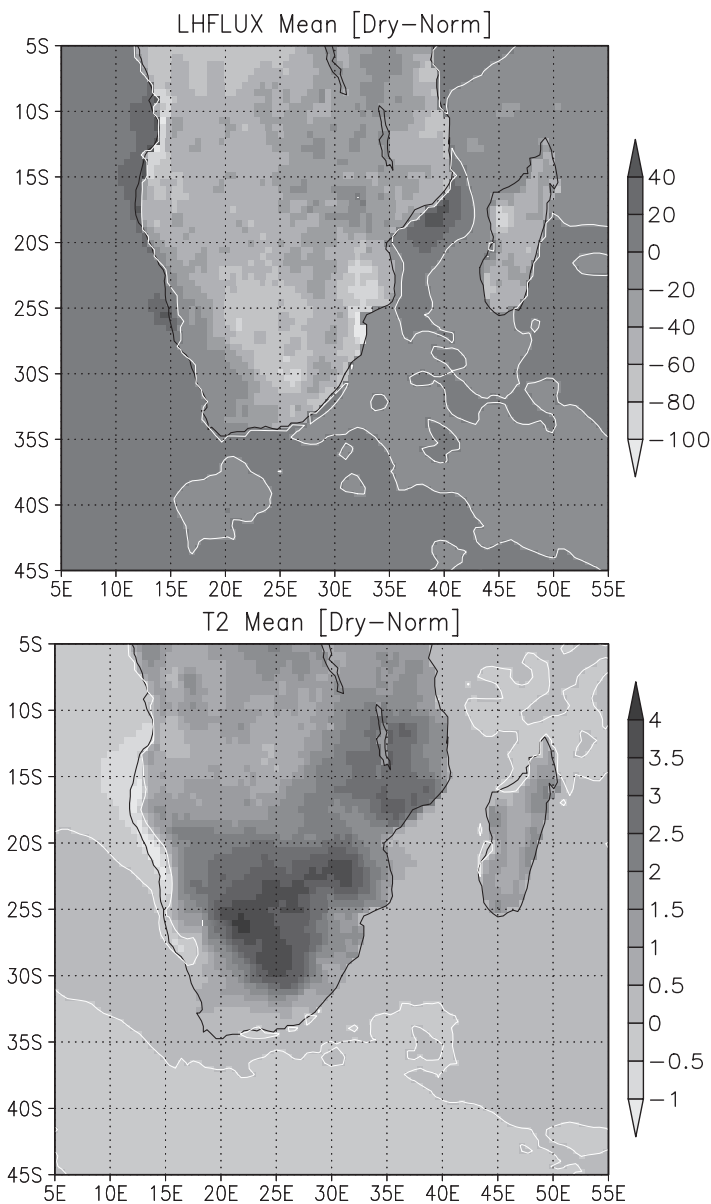
Fig. 1: Nov-Feb mean latent heat flux (upper panel) and surface temperature anomalies(lower panel) forced by a “dry” soil (anomalies relative to the “normal” run).
