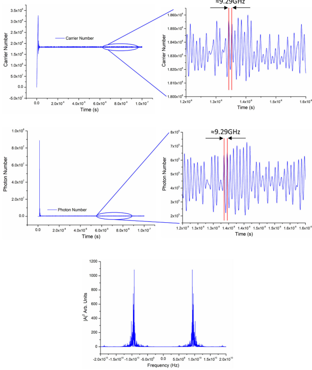
Fig. 10 Carrier (top panel), photon (middle panel) and FFT (bottom panel) outputs with \kappa_c = 5.0 \text{ ns}^{-1} and \Delta\nu = -4 \text{ GHz} [1]
