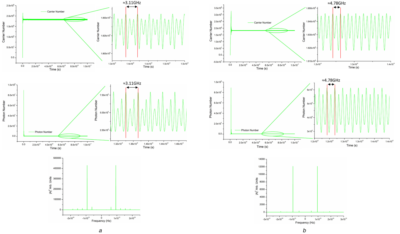
Fig. 9 Typical behaviour observed for complex periodic oscillations (a) Carrier (top panel), photon (middle panel) and FFT (bottom panel) outputs with \kappa_c = 5.0 \text{ ns}^{-1} and \Delta\nu = 0 \text{ Hz} [1], (b) Carrier (top panel), photon (middle panel) and FFT (bottom panel) outputs with \kappa_c = 3.0 \text{ ns}^{-1} and \Delta\nu = -4.6 \text{ GHz} [1]
