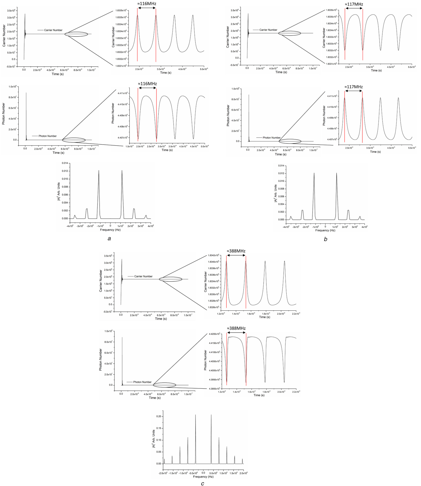
Fig. 8 Typical behaviour observed for single periodic oscillations
