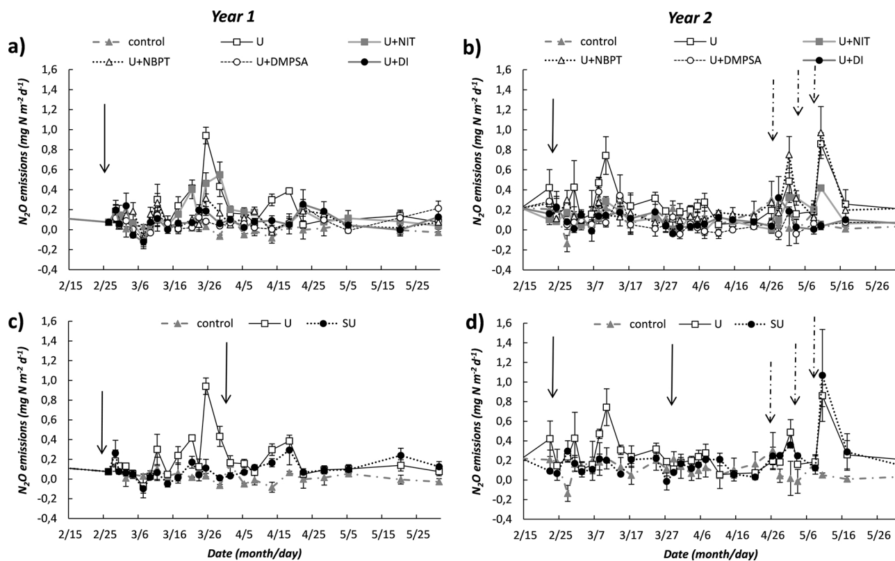
Fig. 4. N_2O emissions in the February–May period in year 1 (a, c) and 2 (b, d) in the different treatments: U (Urea), U + NIT (Urea + Nitrapyrin), U + NBPT (Urea + NBPT), U + DMPSA (Urea + DMPSA), U + DI (Urea + DMPSA + NBPT), split urea (SU) and control. Data are provided separately for inhibitor-based treatments (a, b) and split urea (SU, c, d); and for year 1 (a, c) and 2 (b, d). The plain and dotted arrows indicate N fertilization and irrigation events, respectively. Vertical bars indicate standard errors ( n = 3 ). Outside of the represented period, emissions of N_2O were generally negligible ( -0.1 to 0.1 \text{ mg N m}^{-2} \text{ d}^{-1} ), and fluxes are not shown to improve readability of the figures.
