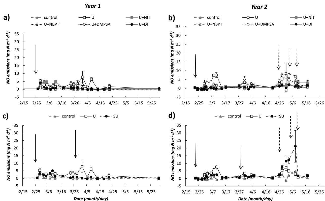
Fig. 5. NO emissions during the experimental period in the February–May period in year 1 (a, c) and 2 (b, d) in the different treatments: U (Urea), U + NIT (Urea + Nitrapyrin), U + NBPT (Urea + NBPT), U + DMPSA (Urea + DMPSA), U + DI (Urea + DMPSA + NBPT), split urea (SU) and control. Data are provided separately for inhibitor-based treatments (a, b) and split urea (SU, c, d); and for year 1 (a, c) and 2 (b, d). The plain and dotted arrows indicate N fertilization and irrigation events, respectively. Vertical bars indicate standard errors ( n = 3 ). Outside of the represented period, emissions of NO were negligible ( < 1 \text{ mg N m}^{-2} \text{ d}^{-1} ), and fluxes are not shown to improve readability of the figures.
