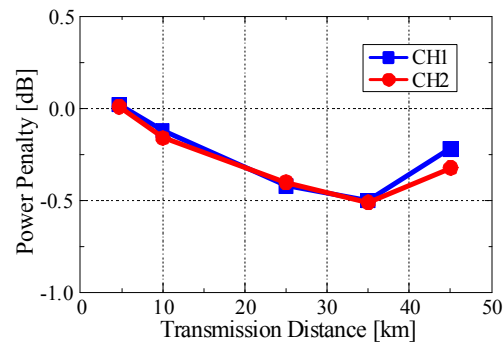
Fig. 6. Power penalty versus transmission distance for CH1 and CH2.
