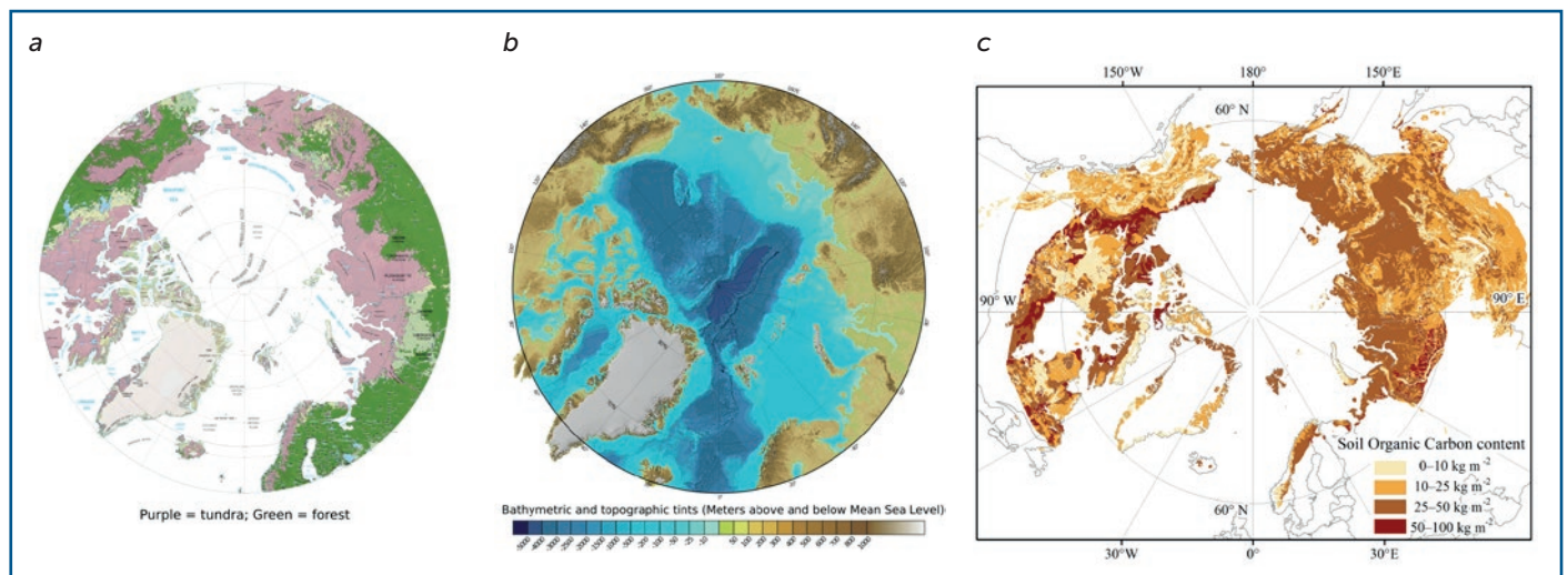
Fig. 1: a: Land cover of the Arctic and Subarctic (polar projection). Key: Dark green = forest; light green = forest-tundra (transitional); pink = tundra. b: Topographic and bathymetric map of the Arctic and Subarctic (polar projection) Pinterest URL: https://www.pinterest.co.uk/pin/298363544038348263/ . c: The Northern Circumpolar Soil Organic Carbon Database version 2. Bolin Centre for Climate Research, Stockholm University. URL: http://bolin.su.se/data/nscsd/
