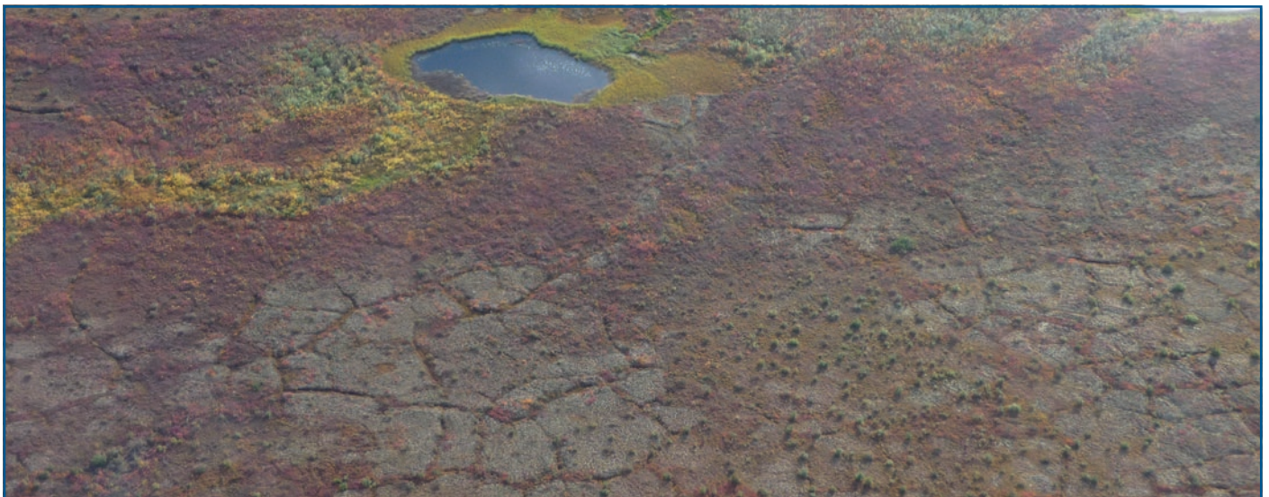
Fig. 5: Areas with ice wedge polygons may become drier with climate change as ice melts and channels between hummocks drain; in this photograph, from the Mackenzie Uplands between Inuvik and Tuktoyaktuk (Northwest Territories, Canada) drainage and drying of polygons is evident, as well as shrub encroachment, especially on polygon margins (photo credit: Philip Wookey)
