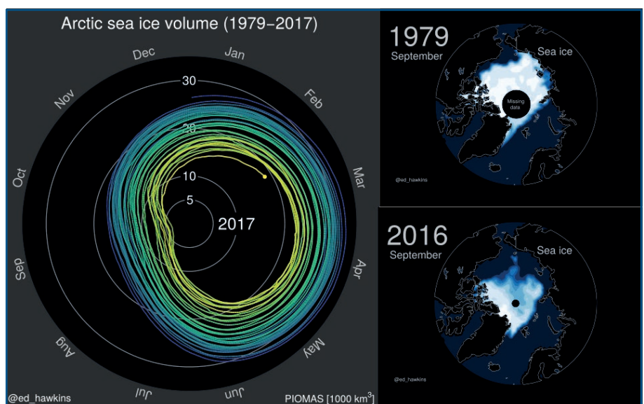
Fig. 3: Sea-ice decline from the 1970s to recent years. The line traces ice volume through time (greatest Mar–May; least Aug–Oct). The most recent years (yellow) show diminishing values compared with the 1980s URL: https://www.climate-lab-book.ac.uk/spirals/
