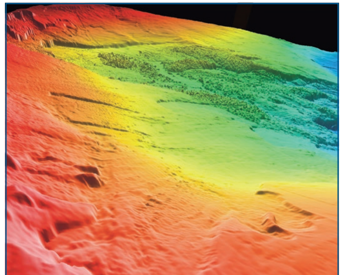
Fig. 10: Sea-floor view (looking south) of the Storegga Slide area (blue/green colours). The slide affected several hundred km of the Norwegian continental shelf about 8000 years ago. Image: Christian Berndt, GEOMAR. URL: http://www.geomar.de/en/news/article/meeresboden-in-bewegung-gefaehrdete-kuesten/
