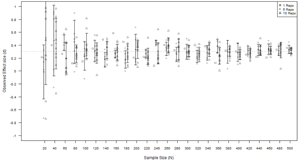
True Effect Size = 0.3
