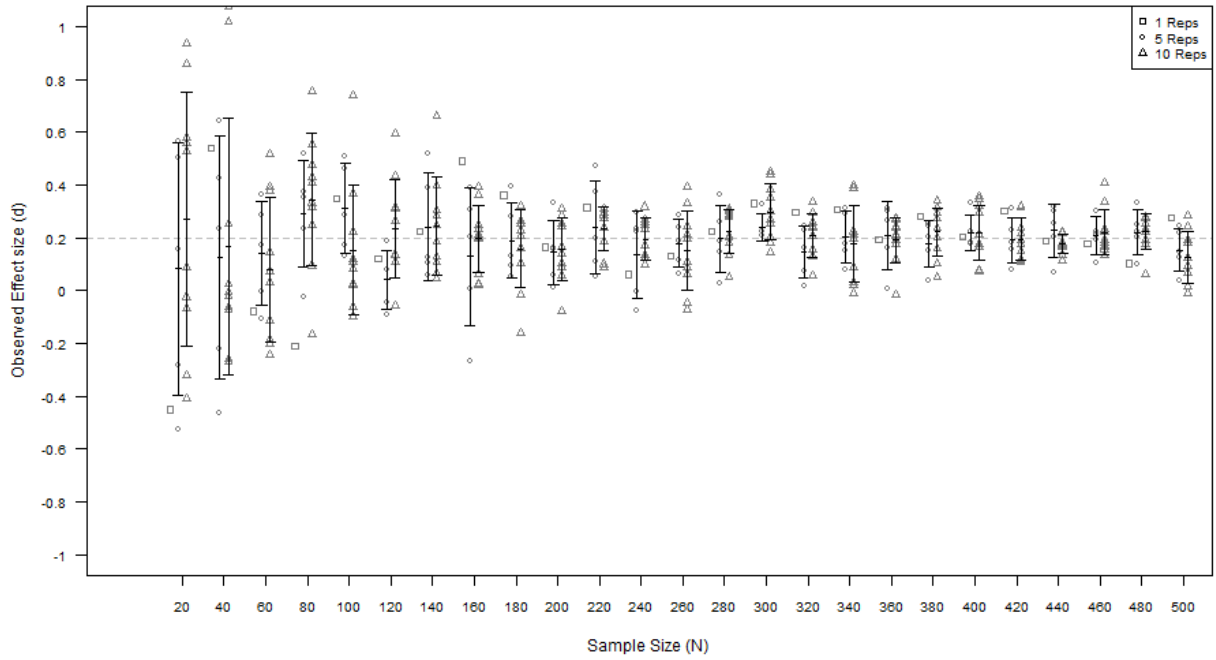
True Effect Size = 0.2
