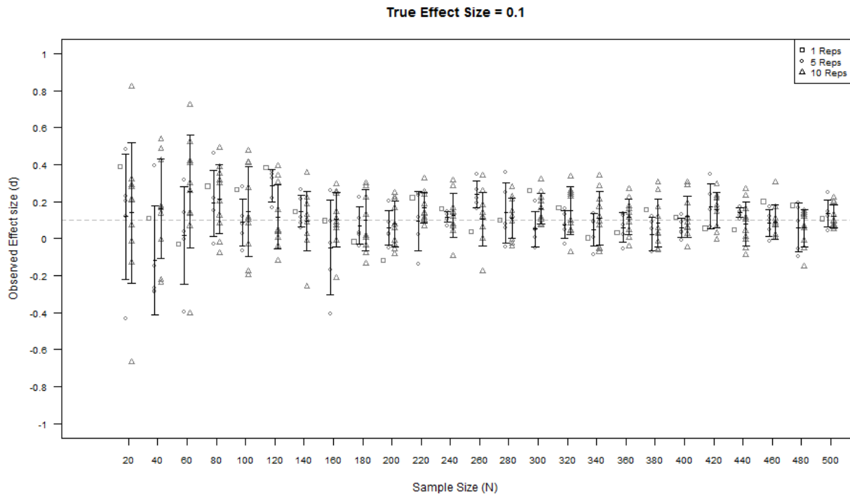
Figures 2-6 are graphs of observed effect sizes of designated effect sizes of .10, .20, .30, .40, and .50 for 1, 5, and 10 replications at sample sizes depicted on the X axis.
