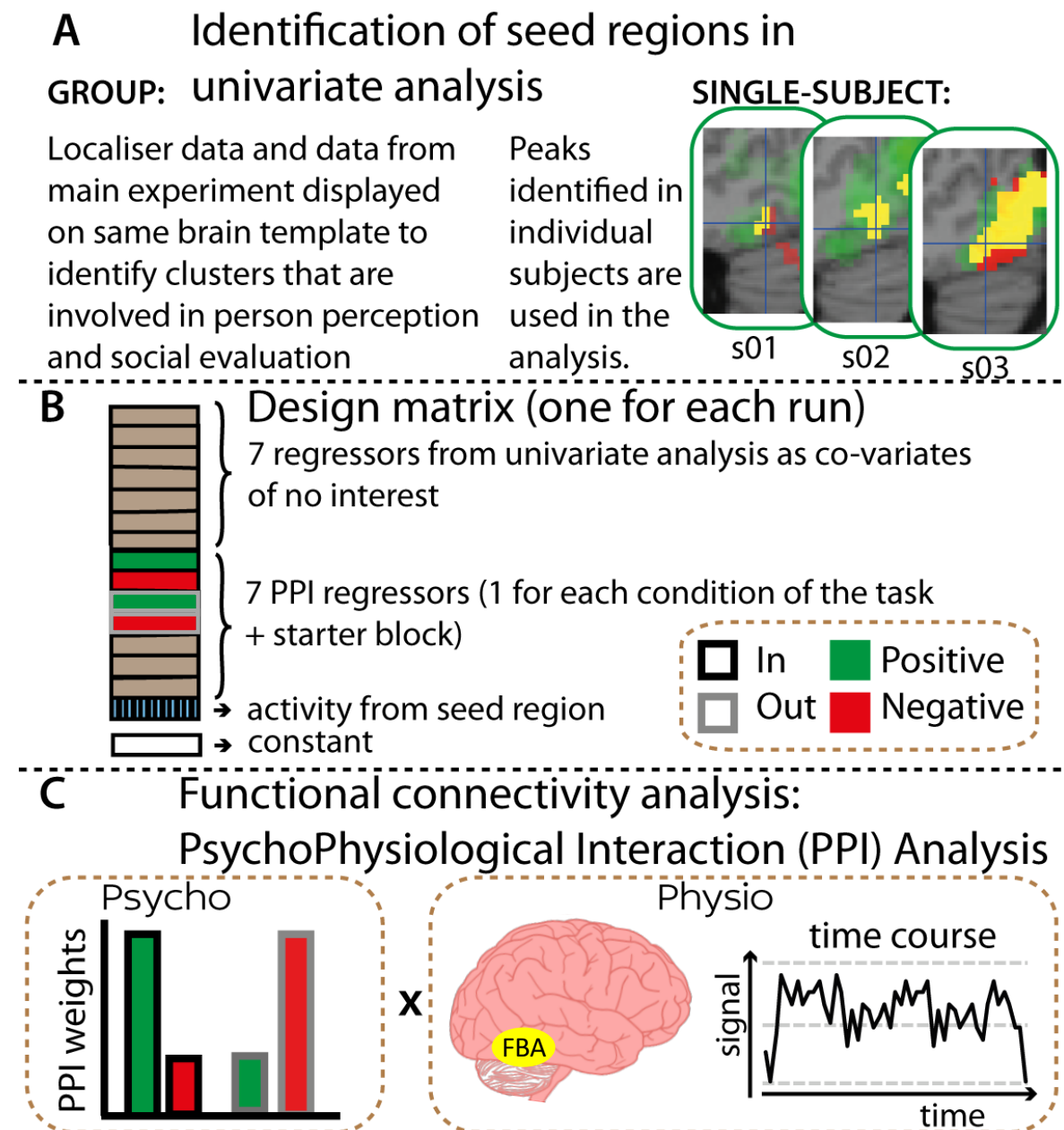
Figure 3. Flow chart illustrating the steps to define seed regions and run PsychoPhysiological Interactions (PPI) analyses. A) Identification of seed regions in the univariate analysis was done at group and single-subject level to allow for inter-individual differences in peak responses. B) An illustration of the design matrix (this was the same for each run), that was created for each participant. C) The “psychological” (task) and “physiological” (time course from seed region) inputs for the PPI analysis.
