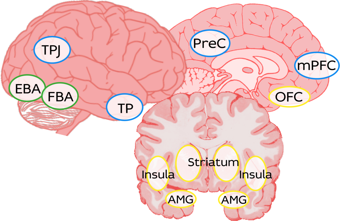
Figure 1. Neural networks involved in body perception (green), Theory of Mind (blue), and affective processing (yellow). Abbreviations: Extrastriate Body Area (EBA), Fusiform Body Area (FBA), TemporoParietal Junction (TPJ), Temporal Pole (TP), Precuneus (PreC), medial PreFrontal Cortex (mPFC), Amygdala (AMG), OrbitoFrontal Cortex (OFC).
