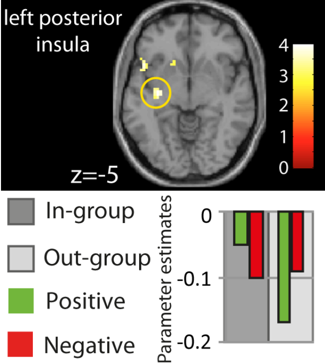
Figure 5. Results from the univariate analysis. The Valence by Group [(PosIn > PosOut) > (NegIn > NegOut)] contrast revealed one cluster within the affective network in left posterior insula. The parameter estimates are extracted from a 4 mm sphere around the peak coordinate.
