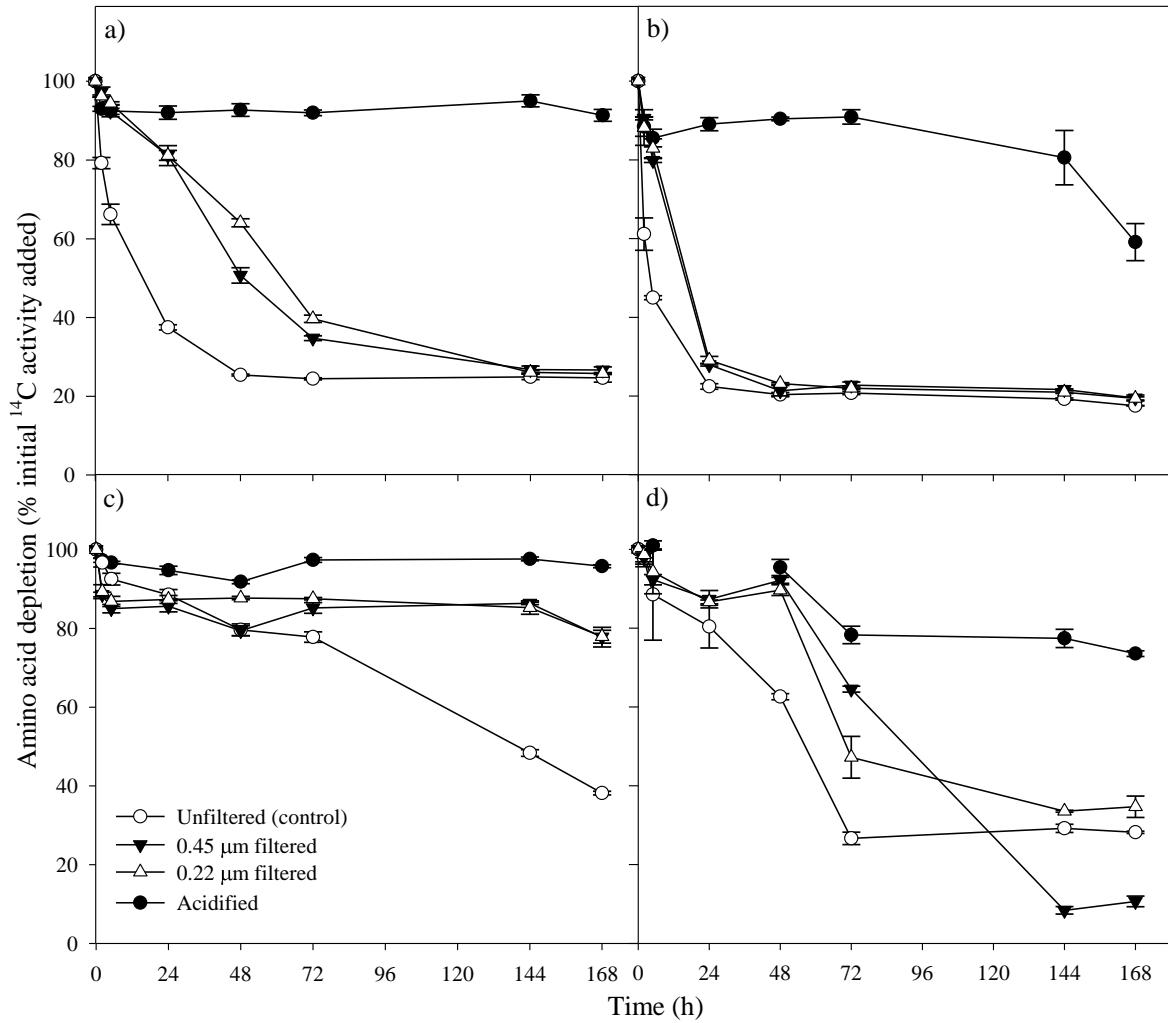
Fig. 3 Effect of filtering (0.45 or 0.2 µm) and acidification on the loss of 14 C-labelled amino acids for: a) Hiraethlyn sub-catchment 5 °C, b) Hiraethlyn sub-catchment 25 °C, c) Migneint sub-catchment 5 °C, d) Migneint sub-catchment 25 °C. Values represent means ± SEM ( n = 3). The legend is the same for all panels.
