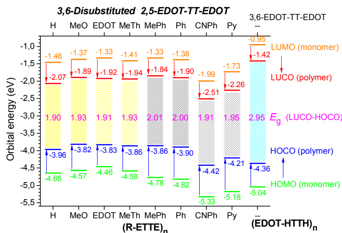
Fig. 5 Evolution of the frontier orbital energy levels from monomers (HOMO, LUMO) to polymers (HOCO, LUCO) and the band gaps of different polymers at B3LYP/6-31G(d) optimized geometries (by PBC for polymers).
