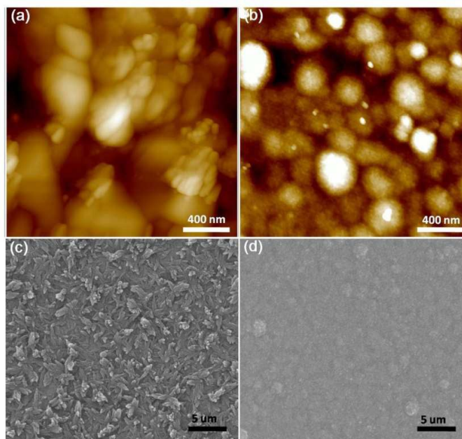
Fig. 10 AFM (a,b) and SEM (c,d; magnification of 25000 \times ) topography images of polymer-coated ITO films: (a,c) P(CNPh-ETTE) ; (b,d) P(Py-ETTE) .
