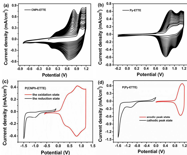
Fig. 6 Potentiodynamic electrochemical polymerization of 0.6 mM monomers: (a) CNPh-ETTE (DCM/THF, 60/40, v/v) and (b) Py-ETTE ( \text{CHCl}_3/\text{ACN} , 75/25, v/v) with \text{TBAPF}_6 (0.1 M) on Pt disk electrode at 100 mV/s (20 cycles are shown). Cyclic voltammograms of electrodeposited polymer films on Pt disk electrode in a monomer-free \text{ACN}/\text{TBAPF}_6 (0.1 M) solution at 100 mV/s under nitrogen atmosphere: (c) P(CNPh-ETTE) and (d) P(Py-ETTE) . Potentials are vs Ag wire.
