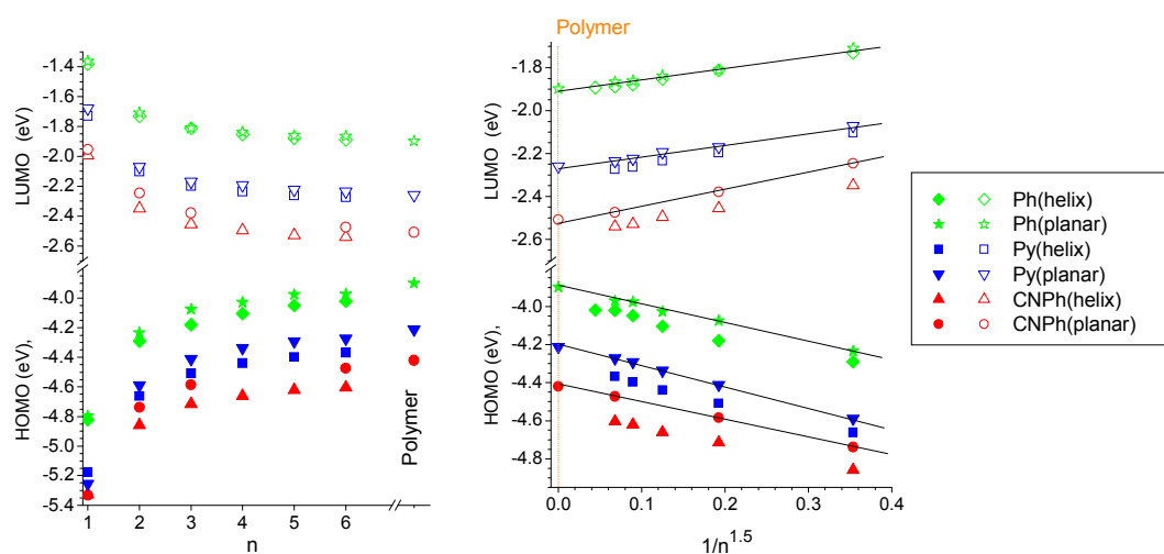
Fig. 3 Chain length dependences of HOMO and LUMO energies for B3LYP/6-31G(d) optimized geometries of helix and planar conformations of (\mathbf{R}\text{-ETTE})_n oligomers ( R = \text{Ph} , CNPh, Py) for corresponding polymers \mathbf{P}(\mathbf{R}\text{-ETTE}) (by PBC). The lines correspond to linear fitting of energies vs 1/n^{1.5} .
