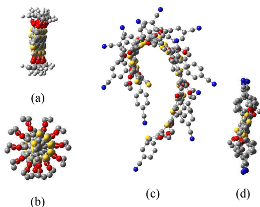
Fig. 1 B3LYP/6-31G(d) optimized geometries of hexamers: (a) (H-ETTE) 6 , (b) helix conformation of (EDOT-HTTH) 6 , (c,d) helix and planar conformations of (CNPh-ETTE) 6 . Views along the oligomers chains are shown; hydrogen atoms in (b-d) are omitted for clarity.
