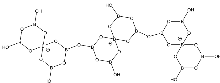
Figure 15. Pentadecaborate(3-) anion as found in (\text{NH}_4)_3[\text{B}_{15}\text{O}_{20}(\text{OH})_8] \cdot 4\text{H}_2\text{O} [105].
