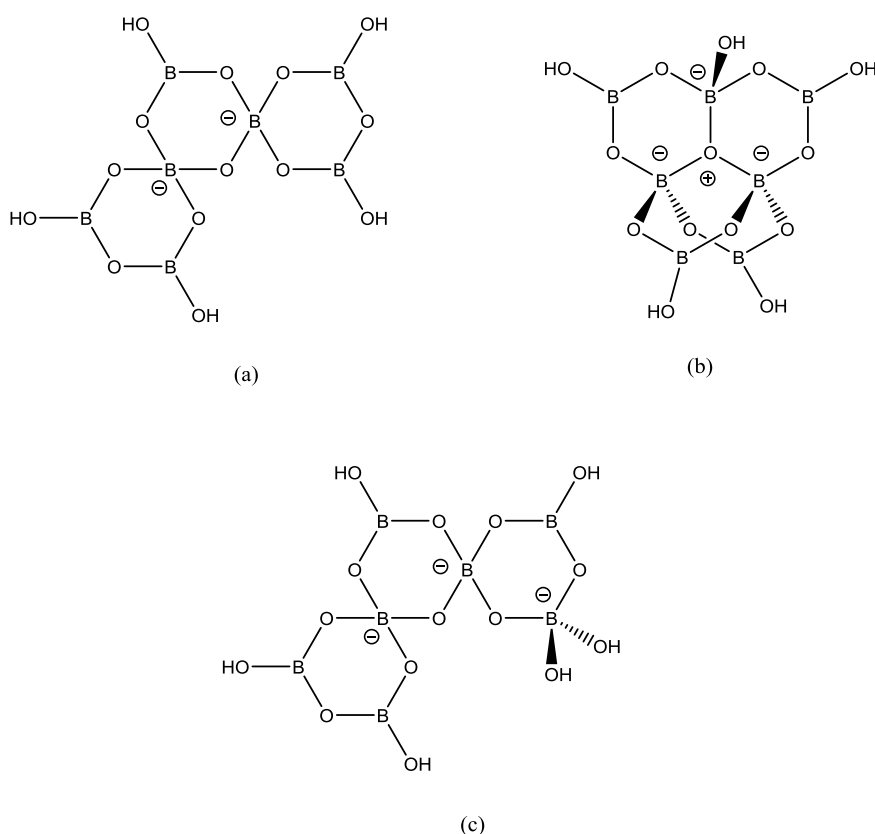
Figure 9. Isolated heptaborate anions as found in (a) [H 2 dab][B 7 O 9 (OH) 5 ]·H 2 O [92], (b) [H 3 N(CH 2 ) 7 NH 3 ][B 7 O 9 (OH) 5 ]·H 2 O [94] and (c) [Co(dien) 2 ][B 7 O 9 (OH) 6 ]·9H 2 O [96].
