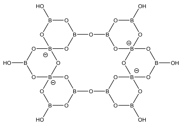
Figure 14. Tetradecaborate(4-) anion as found in [H_3N(CH_2)_2NH_3]_2[B_{14}O_{20}(OH)_6] [34,102].
