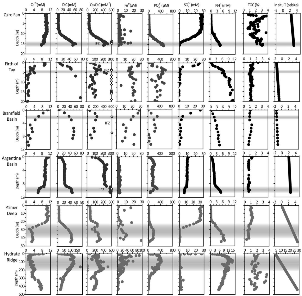
Figure 2. Downcore profiles of compiled parameters at all study sites. The depths for ikaite recovery are marked by diamonds in \text{Ca}^{2+} \times dissolved inorganic carbon (DIC) profiles. The ikaite-formation zones (IFZs) are defined by \text{Ca}^{2+} \times DIC, except for the Firth of Tay (Lu et al. 2012) and the Bransfield Basin (fig. 3), both defined by \delta^{13}\text{C} values. T = temperature. A color version of this figure is available online.
