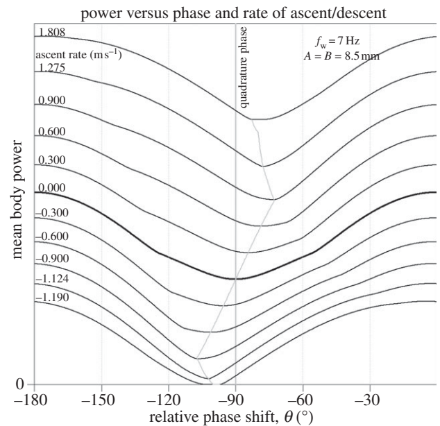
Figure 8. When the bird is ascending or descending, the quadrature phase arrangement is not always optimal. However, the phase \theta for which the power is minimized only deviates significantly from -90^\circ during extreme rates of ascent or descent. The results here simulate a bird with a wingstroke frequency, f_w = 7 \text{ Hz} and equal amplitude oscillations on both forward and vertical axes of amplitude 8.5 \text{ mm} . The locus of points at which the power is minimized at climb rates intermediate between those of the marked traces is also shown.
