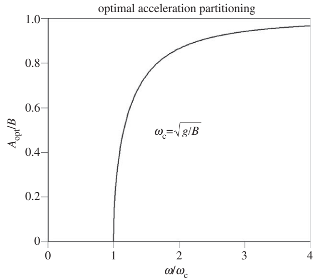
Figure 2. The optimum value of A/B , the ratio of the horizontal and vertical vibration amplitudes, at which body power is minimized and dynamic acceleration on the forward axis attains its smallest acceptable value, see equation (2.24).
