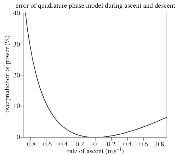
Figure 9. The quadrature phase assumption potentially overpredicts the body power for ascending or descending flight. The error is plotted here for climb rates within the range \pm 0.9 \text{ m s}^{-1} , where the optimum phase appears to deviate linearly from \theta = -90^\circ in figure 8. The model is relatively accurate for sustainable rates of ascent but errors grow rapidly for high rates of descent.
