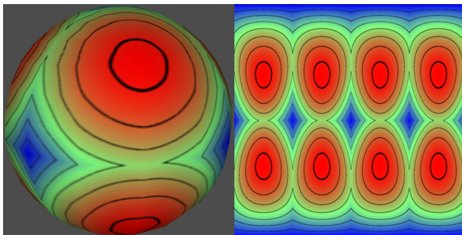
Figure 10. Variation of the error in ODBA with orientation, rising from a minimum of zero (six centres of the square contours) to a maximum of 73.2% (eight centres of the circular contours) with a mean error of 50% (contours at 10% intervals). A single contiguous contour is obtained when ODBA/VeDBA = \sqrt{2} . (Online version in colour.)
