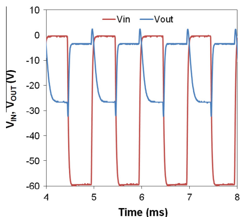
Fig. 9. Response of an inverter stage from the 5-stage ring oscillator ( V_{DD} = -60 V).
