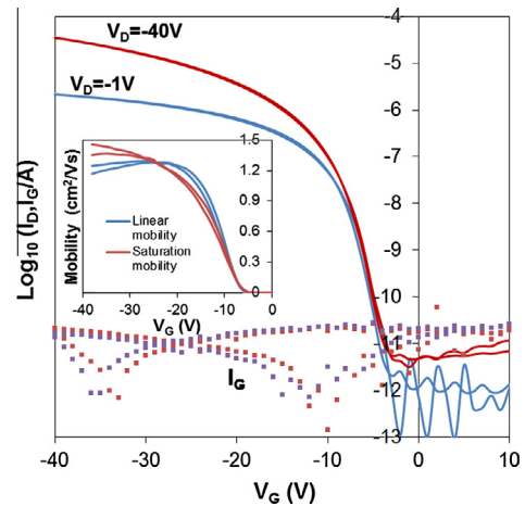
Fig. 3. Transfer characteristics in the linear and saturation regimes for one of the devices from Fig. 2(b) formed on PS-TPGDA. Also shown are the gate leakage current, I_G , (dotted curves) and the gate voltage dependence of mobility in both regimes (inset).
