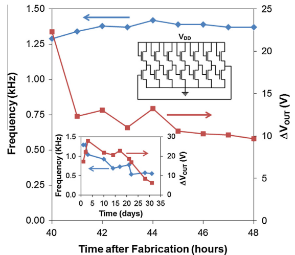
Fig. 8. Performance of a 7-stage ring oscillator during 8 h of continuous operation beginning 40 h after fabrication ( V_{DD} = -60 V). Also shown as an inset, is the performance measured intermittently over 1 month starting 21 h after fabrication.
