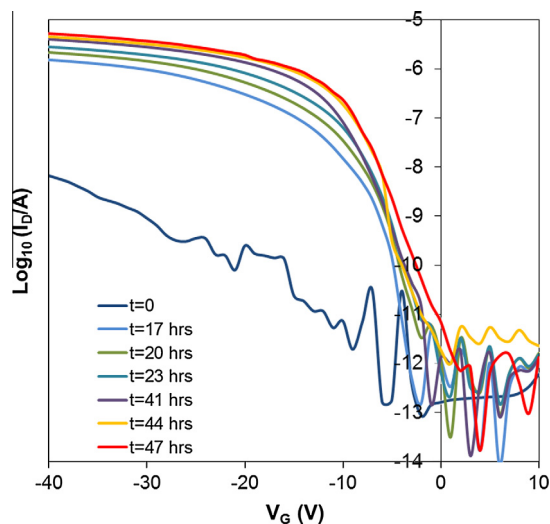
Fig. 1. A series of transfer characteristics obtained at different times after fabrication. On testing immediately after fabrication, the OTFT barely displayed any transistor action but improved significantly over time.
