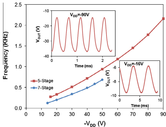
Fig. 7. Output frequency of 5- and 7-stage ring oscillators as a function of the rail voltage V_{DD} . The 7-stage device was tested 21 h after fabrications while the 5-stage device was tested 1 month after fabrication. The insets show the outputs from the 5-stage ring oscillator with V_{DD} = -16 V, the minimum operating voltage, and at -90 V the highest applied voltage.
