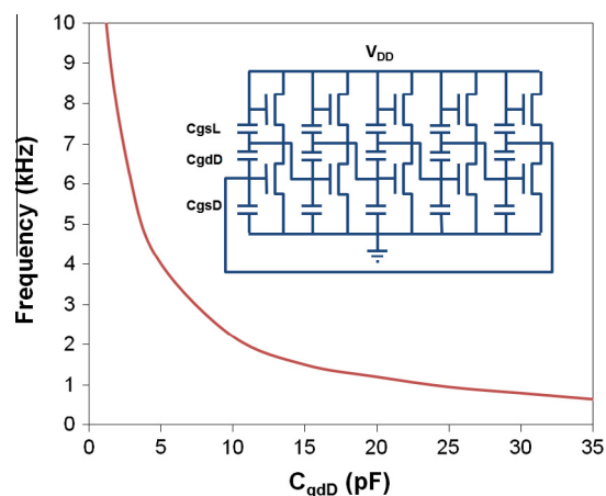
Fig. 10. Effect of parasitic capacitances on the 5-stage ring oscillator frequency deduced from simulations with V_{DD} = -60 V. The inset shows the ring oscillator circuit including parasitic gate–source, C_{gs} , and gate–drain, C_{gd} , capacitances added to the driver (D) and load (L) OTFTs. In the simulation it was assumed that C_{gdD} = C_{gsD} = 5C_{gsL} .
