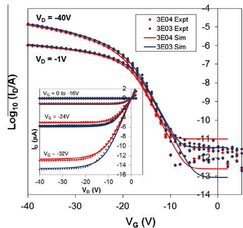
Fig. 5. Transfer and output (inset) characteristics of two adjacent devices (data points) formed on the second batch of PS-TPGDA. The solid lines are simulations obtained using the Silvaco UOTFT software. The main fitting parameters are given in Table 1.
