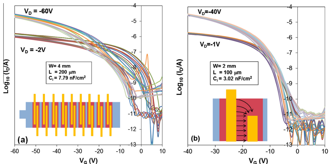
Fig. 2. Transfer characteristics in the linear and saturation regimes for blocks of 9 \times DNTT TFTs fabricated on (a) TPGDA (1 device failed) and (b) PS-TPGDA gate insulators. The inset in (a) shows a schematic plan view of one of the 10 blocks of 9 TFTs with common gate on each substrate while that in (b) illustrates the current flow lines between source and drain near the tip of one electrode.
