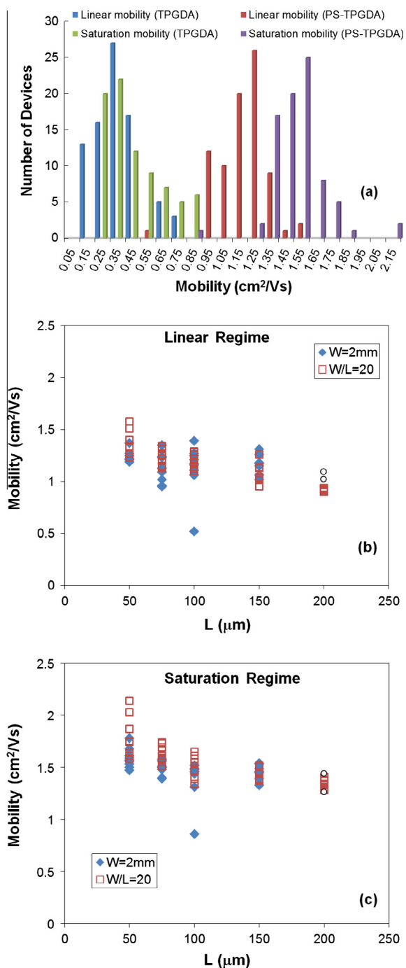
Fig. 4. (a) Histogram showing the number of devices with mobility in the range \pm 0.05 cm ^2 /Vs of the values indicated on the horizontal axis. The improvement achieved by buffering the TPGDA surface with polystyrene is clear. Maximum mobilities extracted in (b) linear and (c) saturation regimes of all the functioning devices on the PS-TPGDA substrate. Also provided for comparison (two open circles) are the mobilities extracted from two devices ( W = 2 mm, L = 200 \mu m) from another substrate.
