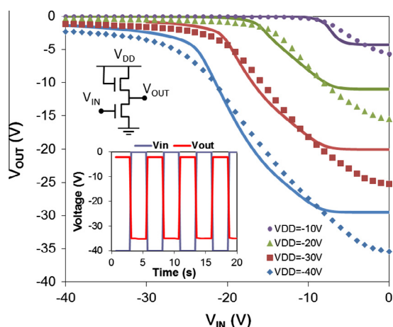
Fig. 6. Experimentally-measured inverter voltage transfer characteristics (points) for different supply voltages, V_{DD} . Also shown (lines) are simulations based on the model card for transistor 3E03 (see Table 1). The insets show the saturated load inverter circuit and the inverter response to a square wave input signal with V_{DD} = -40 V.
