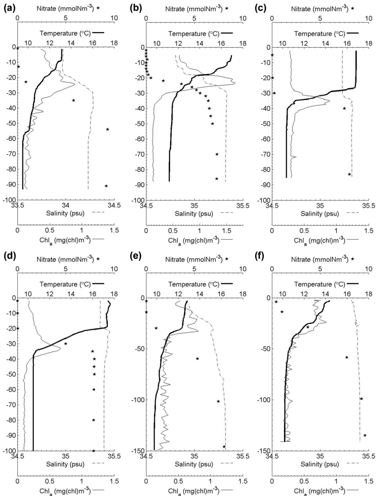
Figure 2. Individual profiles of water column structure for a series of contrasting locations within the seasonally stratified Northwest European shelf seas (locations are shown in Figure 1). Each represents a single CTD profile with temperature, salinity fluorescence, calibrated to show chlorophyll-a, and nitrate concentrations from water samples. (a) S1—Western Irish Sea on 26th June 2002, (b) CS3—Celtic Sea on 5th August 2003, (c) CS1—Celtic Sea on 31st July 2003, (d) OB—Celtic Sea on 2005, (e) S140E—Malin shelf on the 15th July 1996, and (f) S140—Malin shelf on the 14th July 1996.
