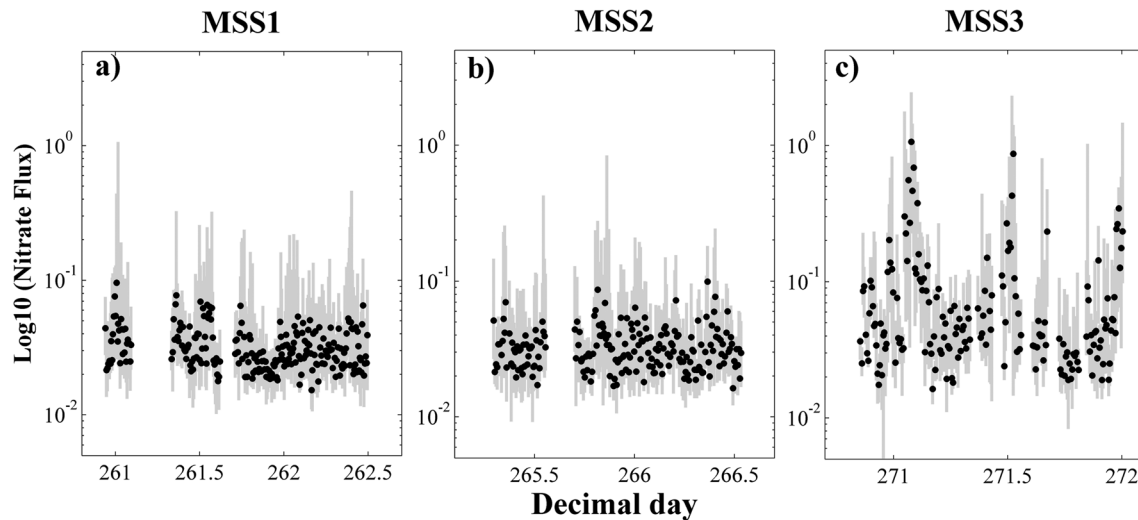
Figure 6. Vertical nitrate flux (y axis is in log scale; units are \text{mmol N m}^{-2} \text{d}^{-1} ) through the pycnocline estimated from the three series of turbulence measurements: (a) MSS1, (b) MSS2, and (c) MSS3. The grey lines represent the interquartile range for each profile, and the black dots indicate the median values.
