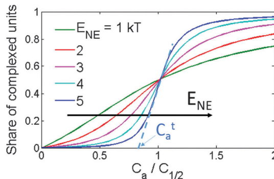
Fig. 7 Share of the complexed repeat units versus acceptor concentration for various E_{NE} according to the NE model. The acceptor concentration is normalized to the concentration at which half of the monomer units of the polymer are complexed, C_{1/2} . C_a^t shows the threshold acceptor concentration for the curve with E_{NE} = 5 \text{ kT} .
