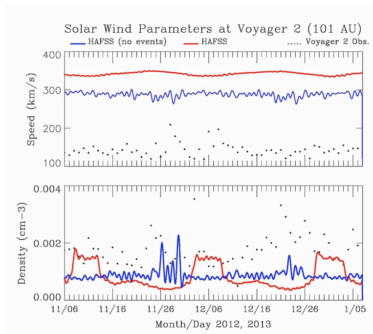
Figure 8. Same as Figure 1 for HAFSS simulations at V2 (at 101 AU) from November 6, 2012 to January 6, 2013.
