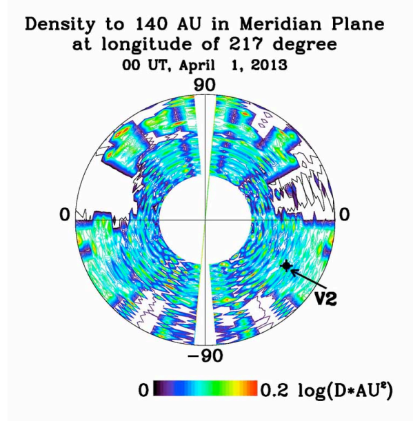
Figure 7. HAFSS plasma density simulations from the Sun to 140 AU in the V2 meridian plane at 217 degrees longitude.
