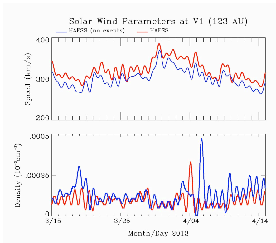
Figure 11. Same as Figure 1 for HAFSS simulations at V1 (at 123 AU) from March 15 to April 15, 2013.
