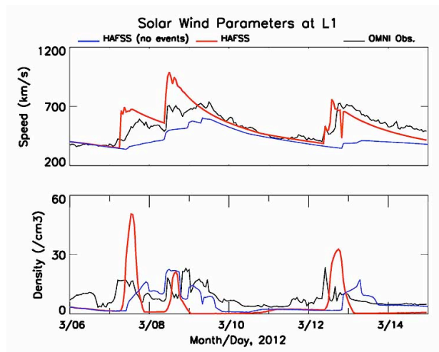
Figure 1. Comparison of HAFSS 3D time-dependent simulation time series results with L1 OMNI observations near Earth (see text). The red line indicates the HAFSS simulation using as inputs the background solar wind and the solar wind from the impulsive solar events (Table 1). The blue line shows the HAFSS results at Earth using only the background (ambient) solar wind inputs. The OMNI data are shown by the black line.
