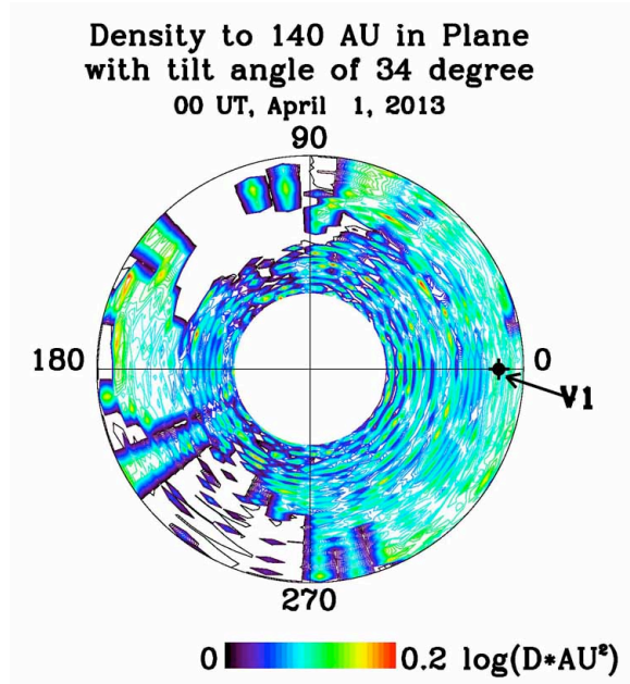
Figure 9. HAFSS plasma density simulations from the Sun to 140 AU in the V1 plane tilted at +34 degrees.
