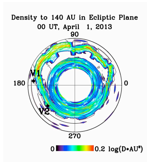
Figure 5. HAFSS ecliptic plane simulation plot of the plasma density from the Sun to 140 AU on April 1, 2013.
