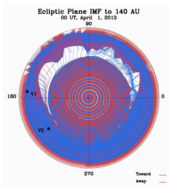
Figure 3. HAFSS ecliptic plane plot of the magnetic field from the Sun to 140 AU. The black dots indicate the locations of V1 at 174 degrees and 123 AU and of V2 at 217 degrees and 101 AU.
