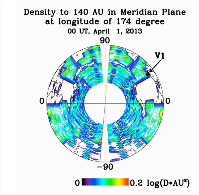
Figure 10. HAFSS plasma density simulations from the Sun to 140 AU in the V1 meridian plane at 174 degrees longitude
