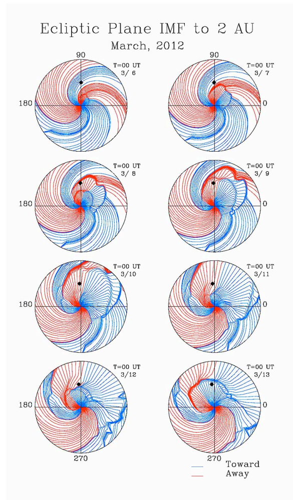
Figure 2. HAFSS ecliptic plane simulation plots of the IMF from the Sun to 2 AU.
