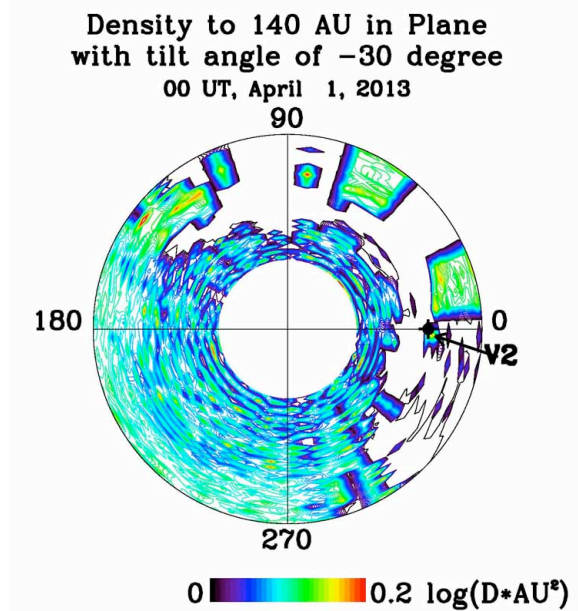
Figure 6. HAFSS plasma density simulations from the Sun to 140 AU in the V2 plane tilted at -30 degrees.
