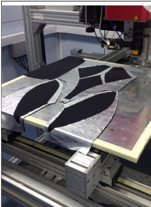
Figure 15. Preparation of flat panels for laser treatment at TWI Author's own 2015
