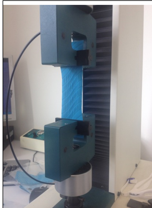
Figure 20. Mechanical testing of laser treated fabric sample: sample under tension Author's own 2014
