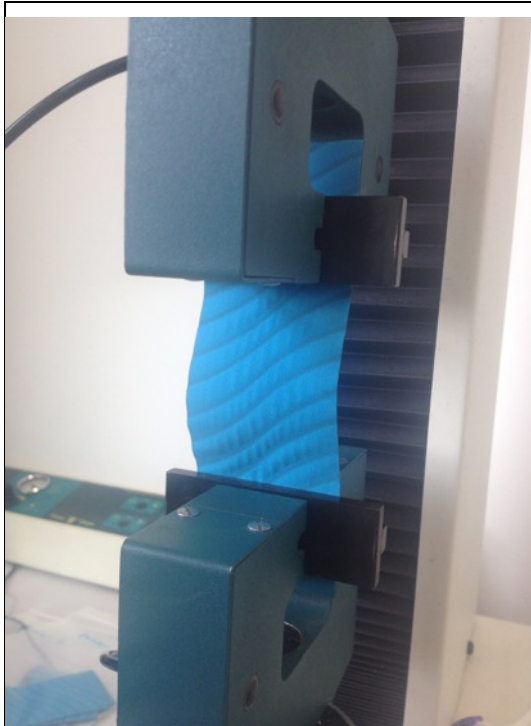
Figure 19. Mechanical testing of laser treated fabric sample: sample relaxed without tension Author's own 2014
