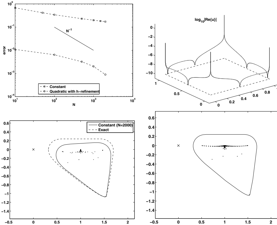
FIG. 5.2. Upper left: Rate of convergence of \gamma^{(h)} on the unit square. Upper right: A function associated with a point of the numerical range close to 0.5. Lower left: Approximate numerical range using piecewise constant basis functions (solid line) against exact numerical range (dotted line). The dots show the eigenvalues of the Galerkin projection A^{(h)} . Lower right: Approximation to exact numerical range and the spectrum of A on the square obtained by using piecewise quadratic basis functions and h -refinement towards corners of the square.
