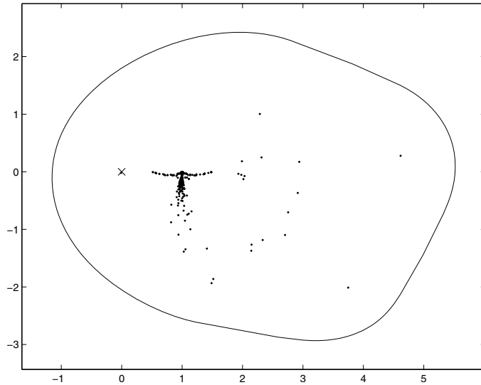
FIG. 5.13. Plot of the numerical range of A_{k,k} for the trapping domain, where k = 5.7 - 0.29i is the approximate value of the first resonance.
