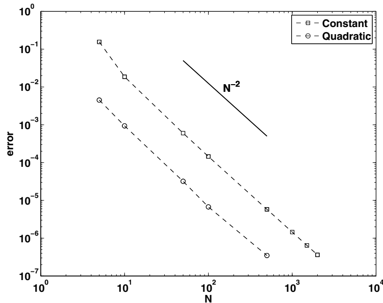
FIG. 5.1. Convergence of the coercivity constant for a growing number of elements per wavelength on the unit circle for k = 1 with constant and quadratic basis functions.
