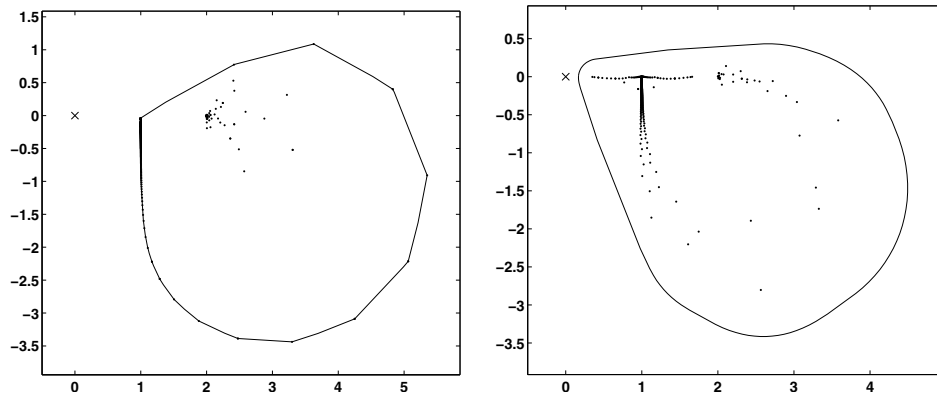
FIG. 3.1. Eigenvalues and boundary of the numerical range of the boundary integral operator A on the unit circle (left plot) and on the equilateral triangle with side length 1 (right plot) for k = 50 .
