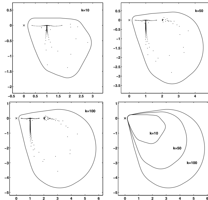
FIG. 5.6. The numerical range of A on the unit square for k = 10, 50, 100 . The black dots are approximations to the spectral values of A . The lower right plot shows a comparison of the numerical ranges for the three different wavenumbers.
