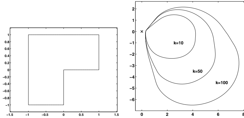
FIG. 5.8. The numerical range for k = 10, 50, 100 of A for the L -shaped domain.
