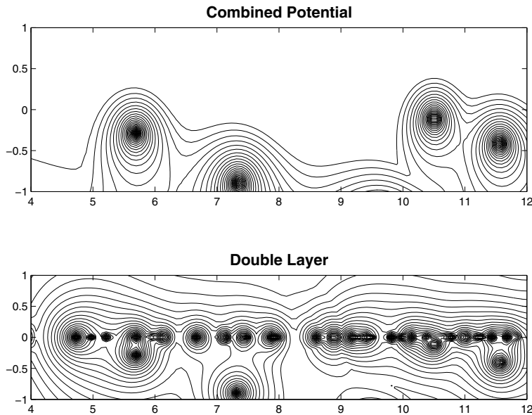
FIG. 5.12. Top: Contour plot of \log_{10}(\|A_{k,k}^{-1}\|) over a part of the complex plane. Bottom: Contour plot of \log_{10} \|(I + K_k)^{-1}\| . In this second plot the singularities in the negative half of the complex plane are resonances, and the singularities on the real axis correspond to eigenfrequencies of the interior Neumann eigenvalue problem.
