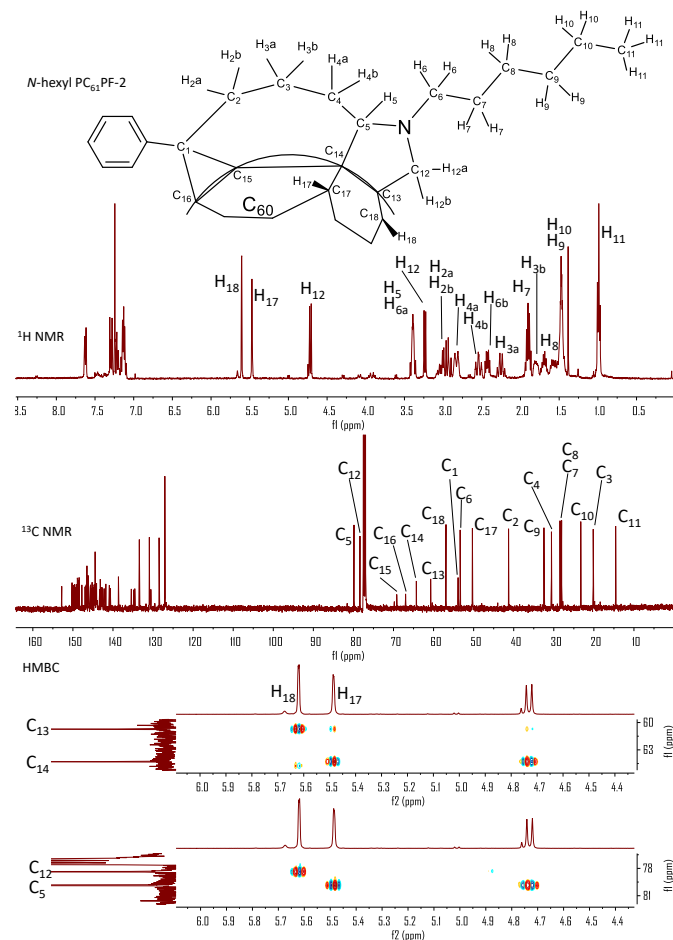
Figure 4. ^1\text{H} , ^{13}\text{C} and HMBC NMR spectrum of N -hexyl \text{PC}_{61}\text{PF-2} with resonances assigned for the key atoms in discussion.
