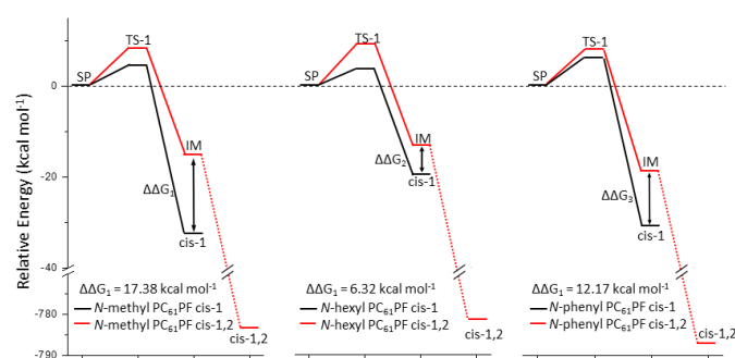
Figure 10. Relative energy of starting point, transition states, intermediates and products of PC 61 PF compounds with cis -1 and cis -1,2 configuration from DFT calculations.
