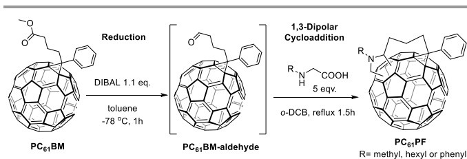
Figure 2. One-pot two-step synthesis of PC 61 PF derivatives.
