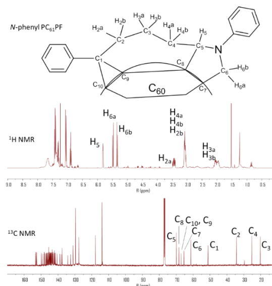
Figure 6. ^1\text{H} and ^{13}\text{C} spectrum of N -phenyl \text{PC}_{61}\text{PF} with resonances assigned for the key atoms in discussion.
