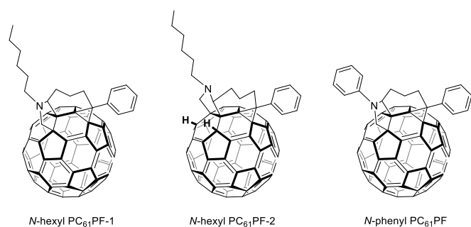
Figure 8. Chemical structures of N -hexyl PC 61 PF-1, N -hexyl PC 61 PF-2 and N -phenyl PC 61 PF.
