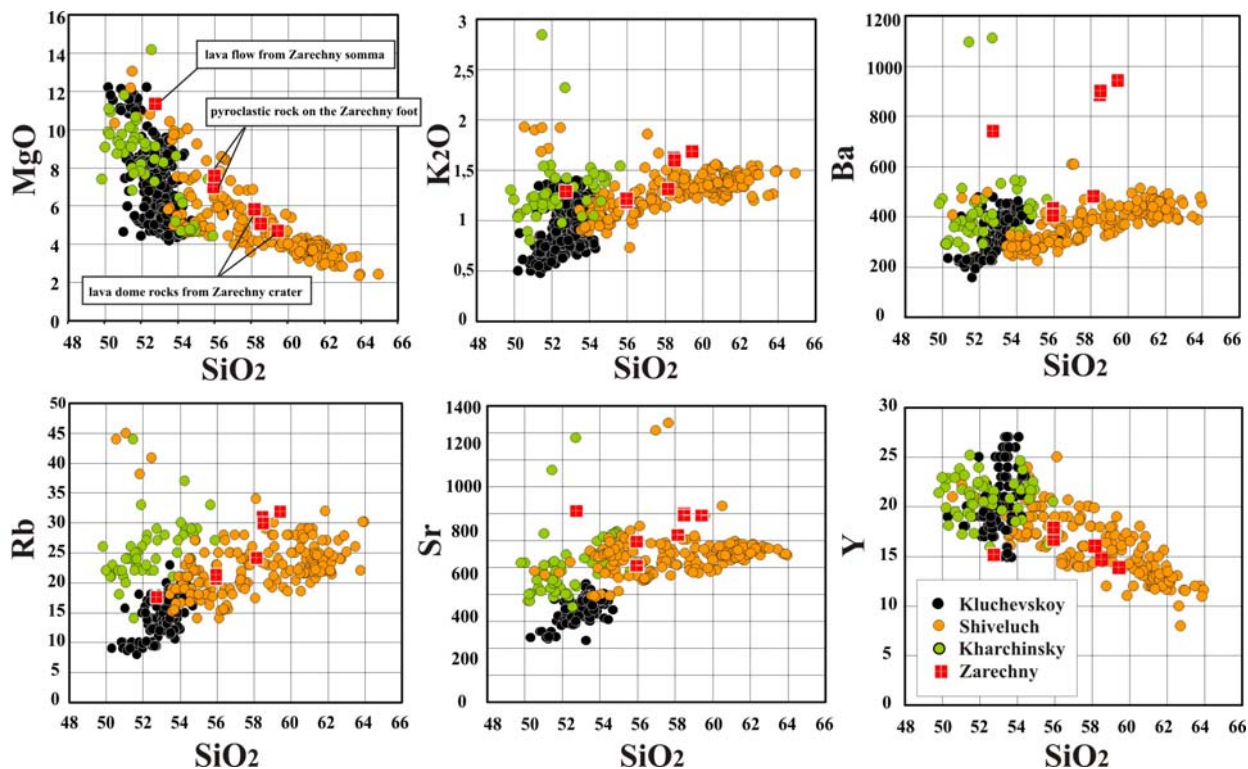
Fig. 2. Selected major (Mg, K) and trace (Ba, Rb, Sr, Y) elements composition of Zarechny volcano rocks compared with the neighboring CKD volcanoes. The composition of Kluchevskoy rocks from Portnyagin et al. (2007); Shiveluch – from Gorbach and Portnyagin (2011) and Gorbach et al. (2013), and Kharchinsky volcano from our unpublished data.
