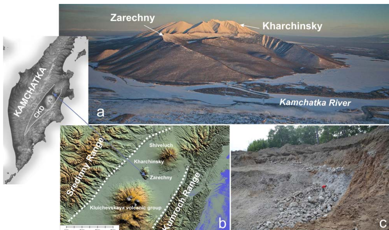
Fig. 1. Zarechny volcano (a) with its regional position (b) and deposits (c). Photo by Yuri Demyanchuk (a) and Anastasiya Plechova (c).
