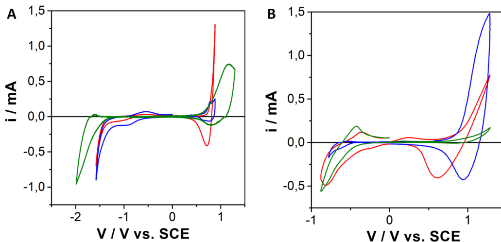
Figure 2. Second cyclic voltammograms in the solid state at 0.1 \text{ V s}^{-1} of PT2Shex(2) (green line), PT2Sbr1 (red line) and PT2Sbr2 (blue line) (A) and their corresponding blends (B).
