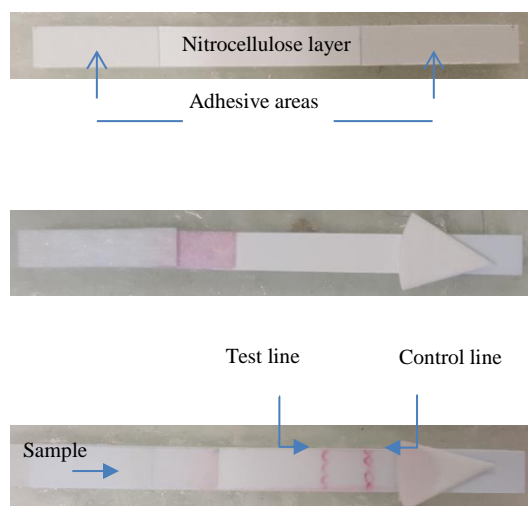
Fig. 1. Blank nitrocellulose membrane (top), assembled lateral flow strip (middle) and strip after the assay (bottom). The positions of the test line and the control remain the same for all the results exhibited later in the paper
