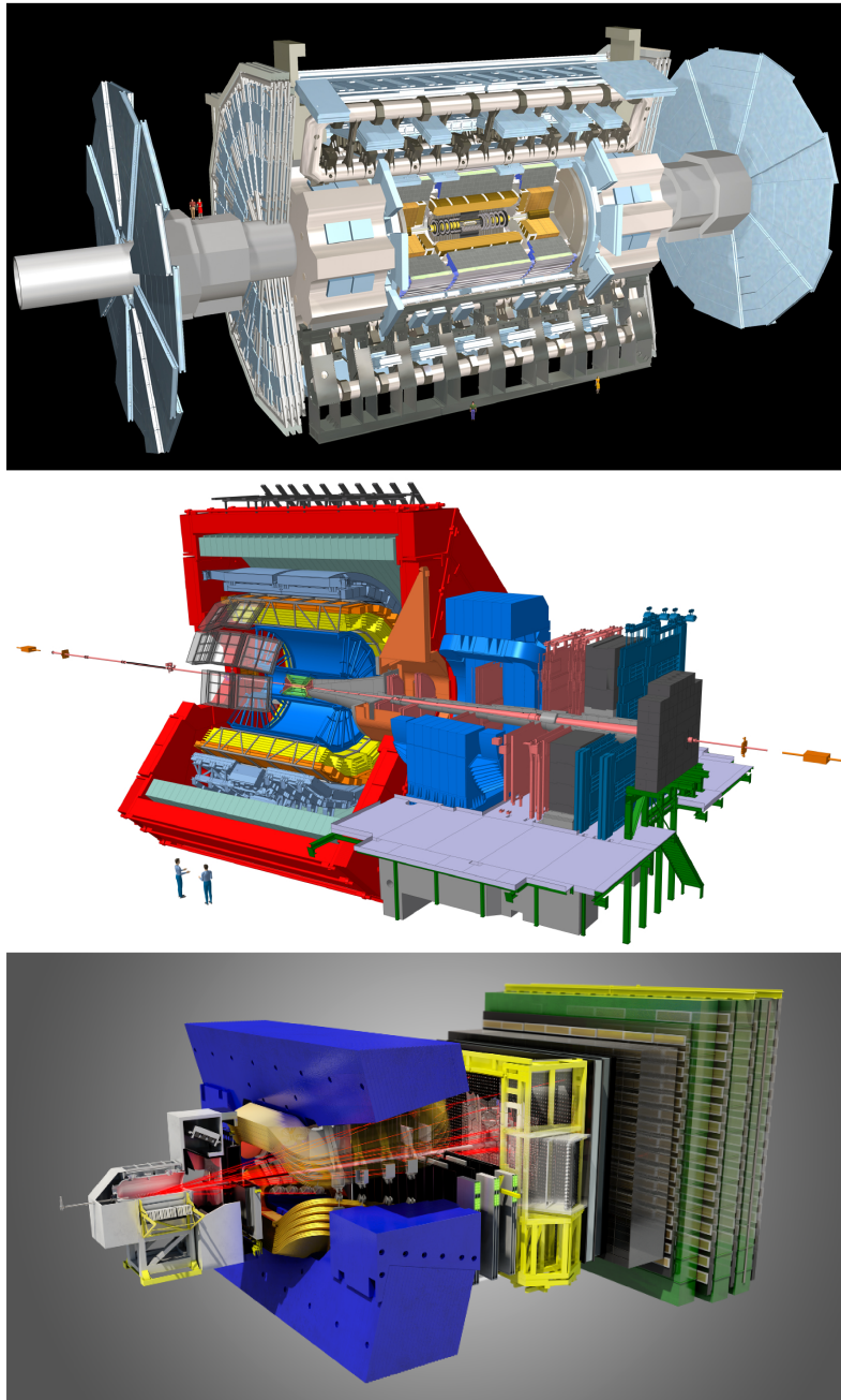
Figure 3.21: Top: the ATLAS experiment. [88] Center: the ALICE experiment. [89] Bottom: the LHCb experiment. [90]
