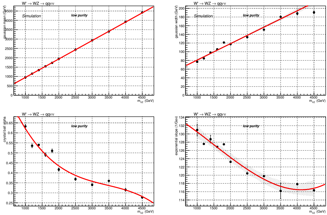
Figure 4.53: Interpolation of the fitted parameters as a function of the resonance mass, for a spin-1 ( W' ) signal hypothesis, low-purity category.
