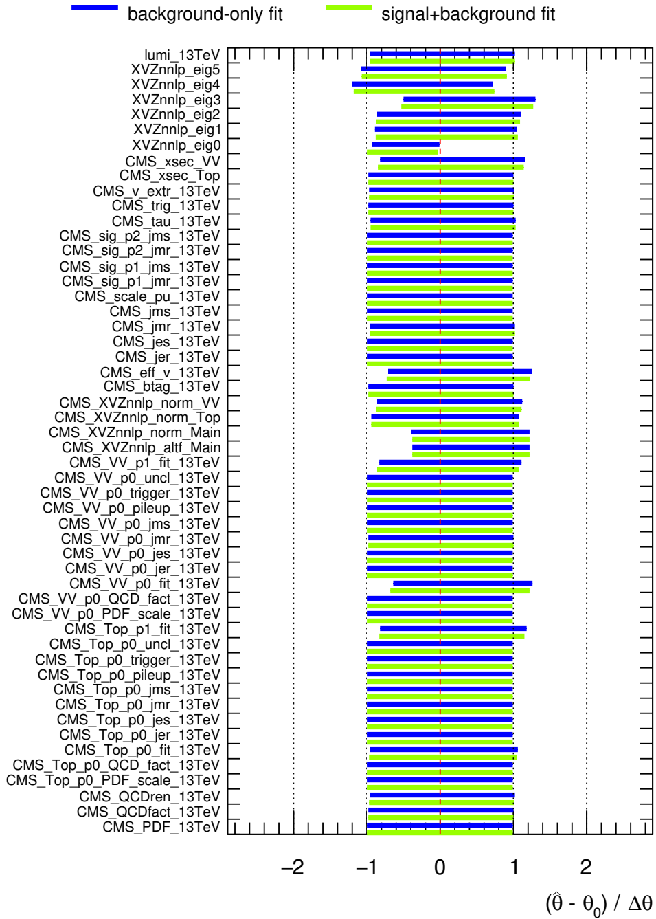
Figure 4.63: Nuisance pulls for the low-purity category, calculated under both the background-only (blue bars) and signal plus background hypotheses (green bars). A signal hypothesis of a spin-2 bulk graviton of mass 3 TeV is considered.
