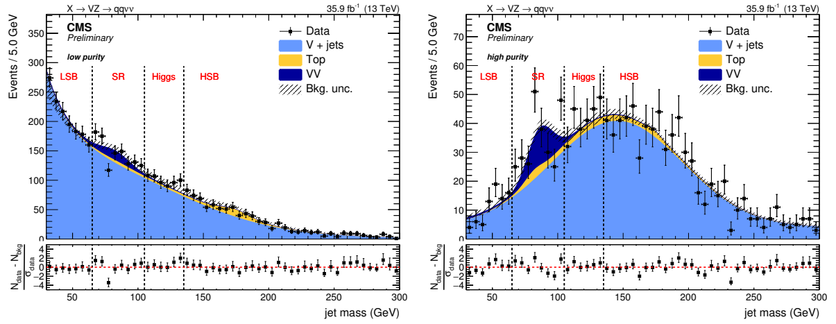
Figure 4.38: Background yield prediction in the signal region, after the fit to data sidebands, in the low- (left) and high-purity category (right). Data and predictions are in agreement.
