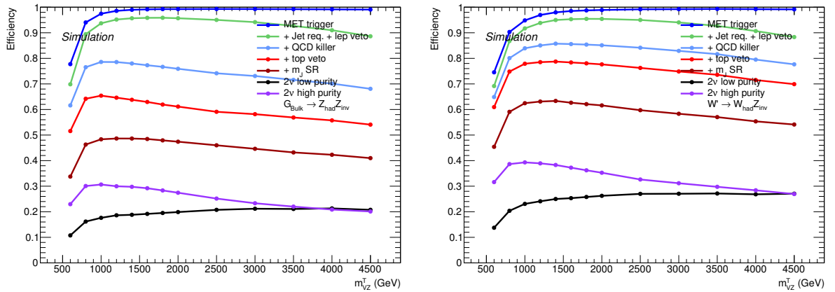
Figure 4.25: Signal efficiency for a spin-2 bulk graviton decaying into a pair of Z bosons (left), and for a spin-1 W' decaying into a W and a Z bosons (right), as a function of the mass of the heavy particle. The efficiencies are separated by purity category after the signal region selections.
