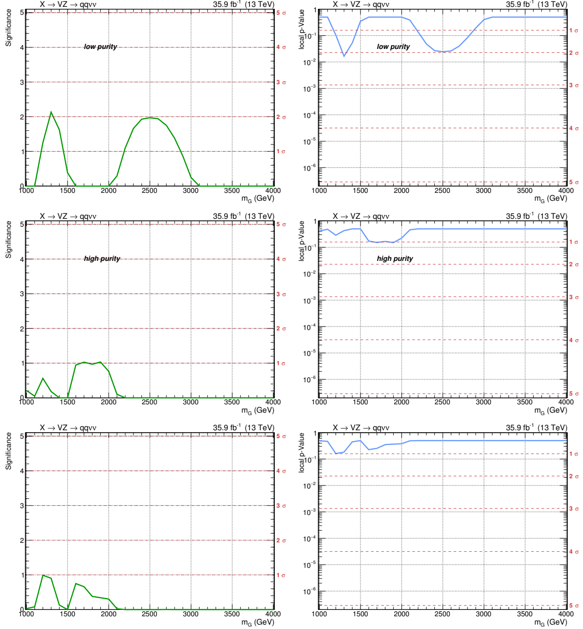
Figure 4.68: Local significances (left plots) and local p-values (right plots) as a function of the resonance mass, for a spin-2 bulk graviton hypothesis, in the low- (top), high-purity categories (center), and in the combination of the categories (bottom).
