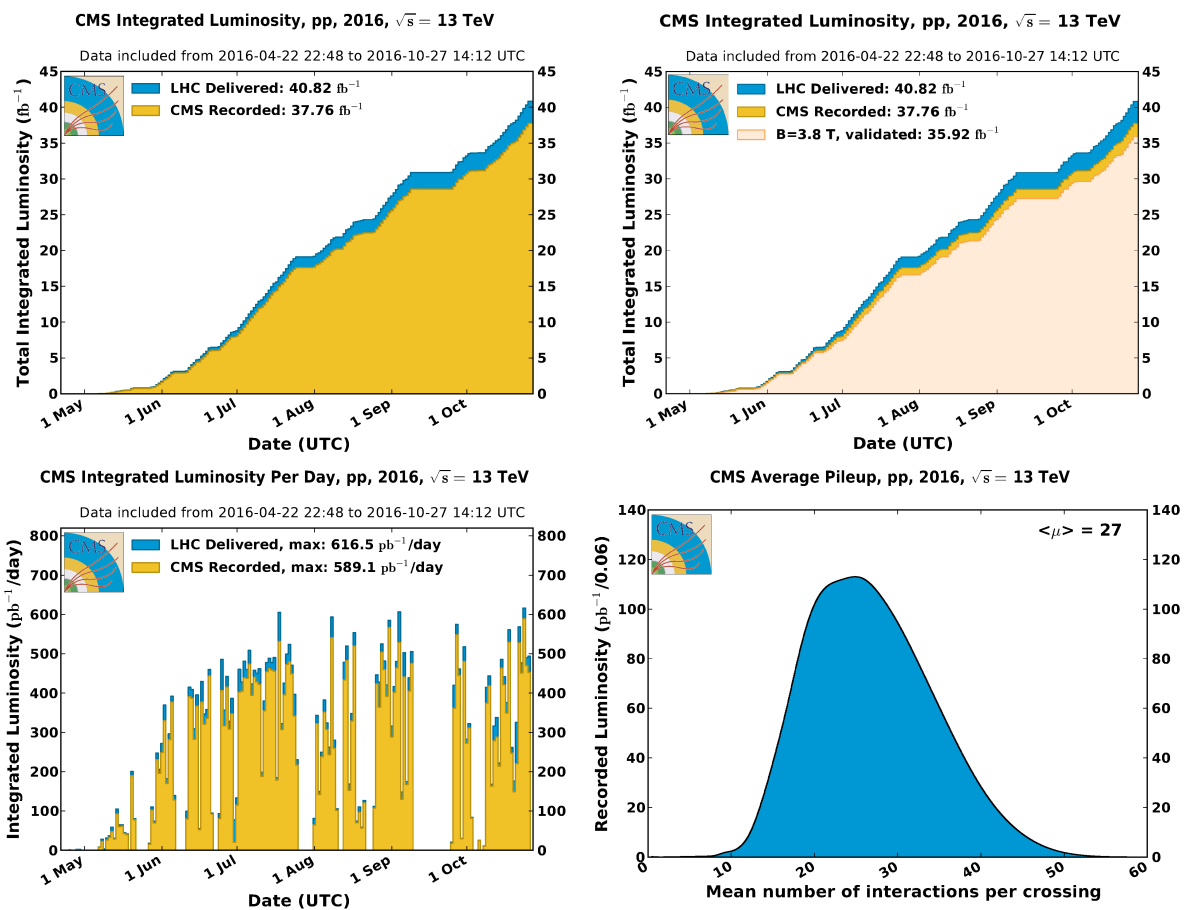
Figure 3.3: Luminosity in 2016 LHC data. Top-left plot: the cumulative integrated luminosity delivered by the LHC (in blue) and recorded by the CMS detector (in orange), as a function of the data-taking period. Top-right plot: data recorded by CMS and declared as optimal for the physics analyses (in light orange), corresponding to a total integrated luminosity of 35.9\ \text{fb}^{-1} . Bottom-left plot: maximum integrated luminosity per day. Bottom-right plot: number of proton interactions per bunch crossing (pile-up). [53]
