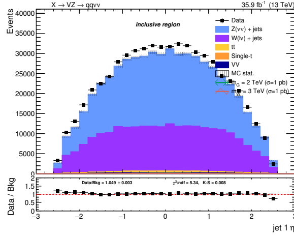
Figure 4.16: Leading AK8 jet \eta spectra after inclusive selections.
