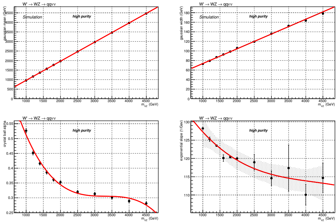
Figure 4.54: Interpolation of the fitted parameters as a function of the resonance mass, for a spin-1 ( W' ) signal hypothesis, high-purity category.
