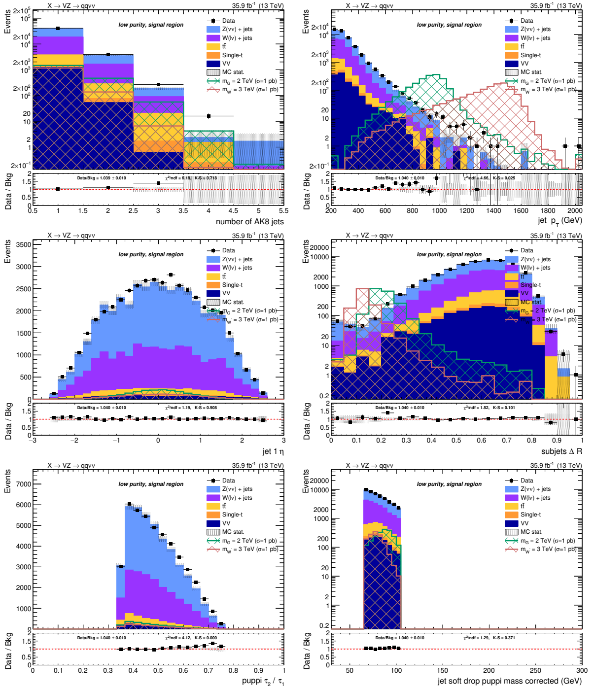
Figure 4.32: Top: number of AK8 jets in the event (left) and V jet candidate p_T (right). Center: V jet candidate \eta (left) and angular separation \Delta R between the constituents leading subjets (right). Bottom: V jet candidate \tau_{21} subjeetiness after PUPPI correction (left) and V jet candidate soft drop PUPPI mass (right). Events are selected with the low-purity, signal region selection, and simulated backgrounds are normalized to luminosity.
