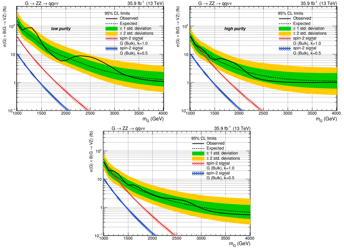
Figure 4.66: Top: observed and expected (with \pm 1(2)\sigma band) 95% C.L. upper limit on \sigma \mathcal{B}(G \rightarrow Z_{\text{had}}Z_{\text{inv}}) for a spin-2 (bulk graviton) signal, for low-purity (left) and high-purity (right) categories, including all statistical and systematics uncertainties. Background predictions are extracted with the \alpha method. Bottom: observed and expected (with \pm 1(2)\sigma band) 95% C.L. upper limit on \sigma \mathcal{B}(G \rightarrow Z_{\text{had}}Z_{\text{inv}}) for a spin-2 (bulk graviton) signal, combining the two purity categories.
