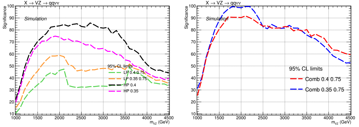
Figure 4.21: Analysis sensitivity to bulk graviton signals, computed by applying different \tau_{21} categorizations, considering the categories separately (left) and combining them together (right), as a function of the resonance mass.
