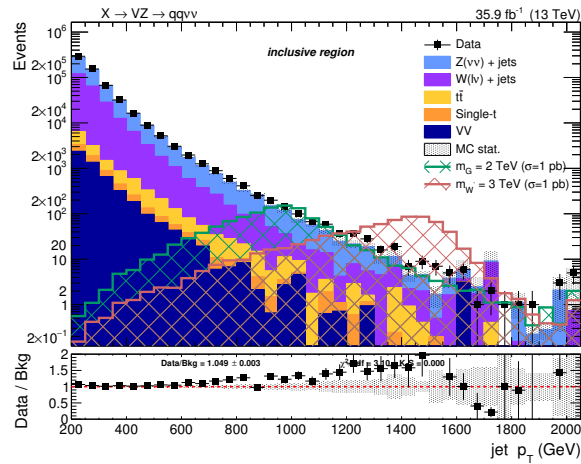
Figure 4.15: Leading AK8 jet p_T spectrum after inclusive selections.
