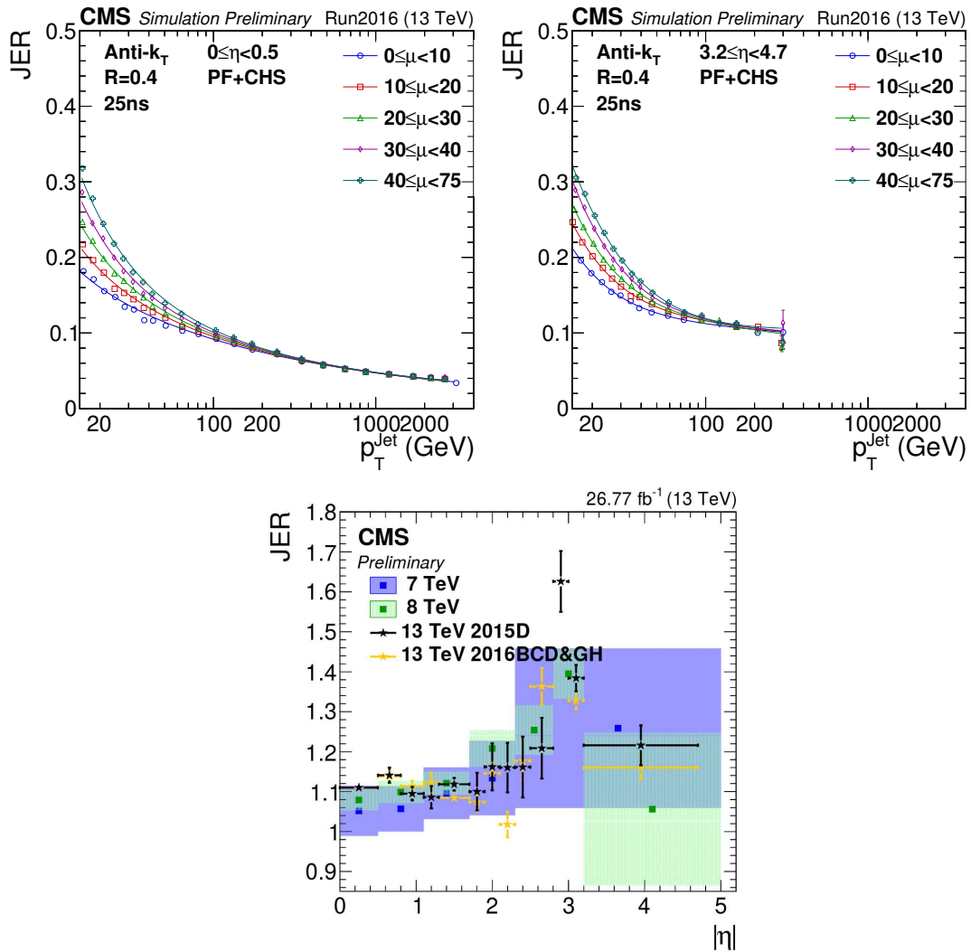
Figure 3.16: Top: jet energy resolution in MC simulations, as a function of the jet p_T . Different curves represent a different average number of primary vertices per event ( \mu ). Bottom: data-MC scale factors, as a function of the jet \eta , measured in 2016 data (yellow dots). [81]
