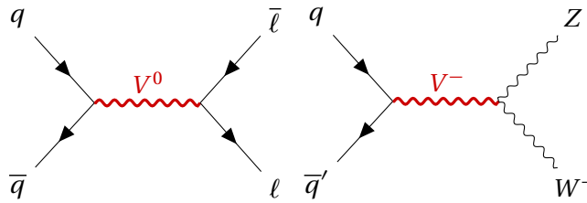
Figure 2.3: Examples of Drell-Yan production mechanism of a heavy V HVT boson: q - \bar{q} quark scattering producing a neutral V^0 that decays leptonically (left); q - \bar{q}' scattering producing a charged V^- that decays into a W and Z bosons (right).
