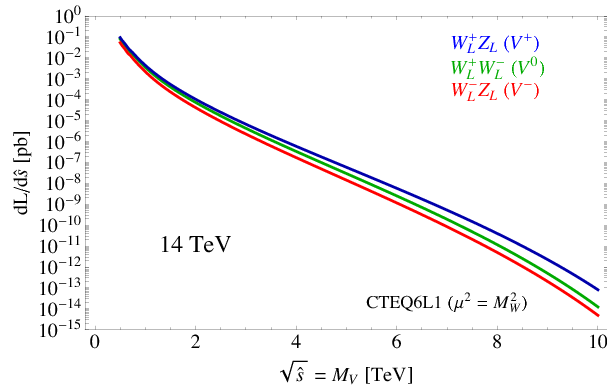
Figure 2.6: Parton luminosities for VBF production process of a heavy V HVT boson, as a result of the scattering between longitudinally polarized vector bosons, as a function of the parton center-of-mass energy, for the LHC proton-proton collisions performed at 14 TeV. [14]
