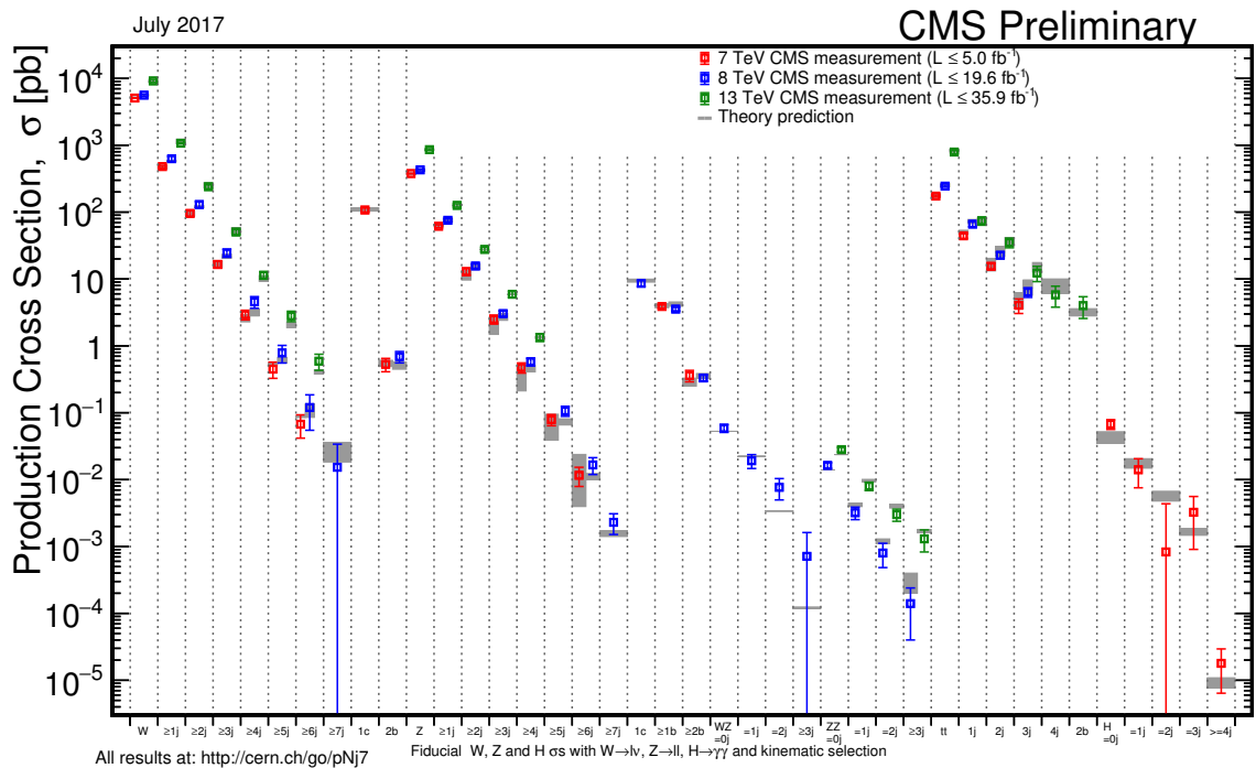
Figure 4.9: Production cross-sections of the standard model processes involving a vector boson in association with jets, as measured by CMS, and theoretical predictions. These phenomena represent the main background sources for the analysis. [97]
