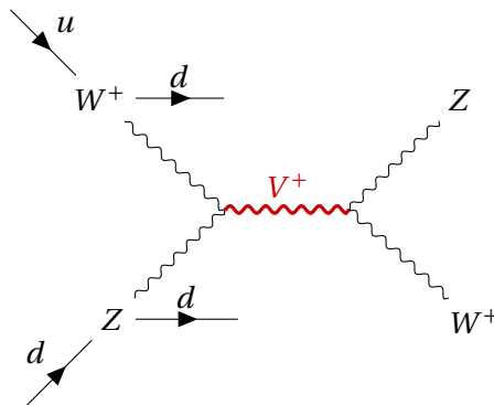
Figure 2.4: Example of VBF production mechanism of a heavy V HVT boson: a charged V^+ boson is produced by a couple of W and Z bosons, as a result of electroweak interactions of initial state u and d quarks. V^+ decays into a Z boson and a W^+ boson. The final state signature includes the presence of a pair of quarks, due to the primary interactions.
