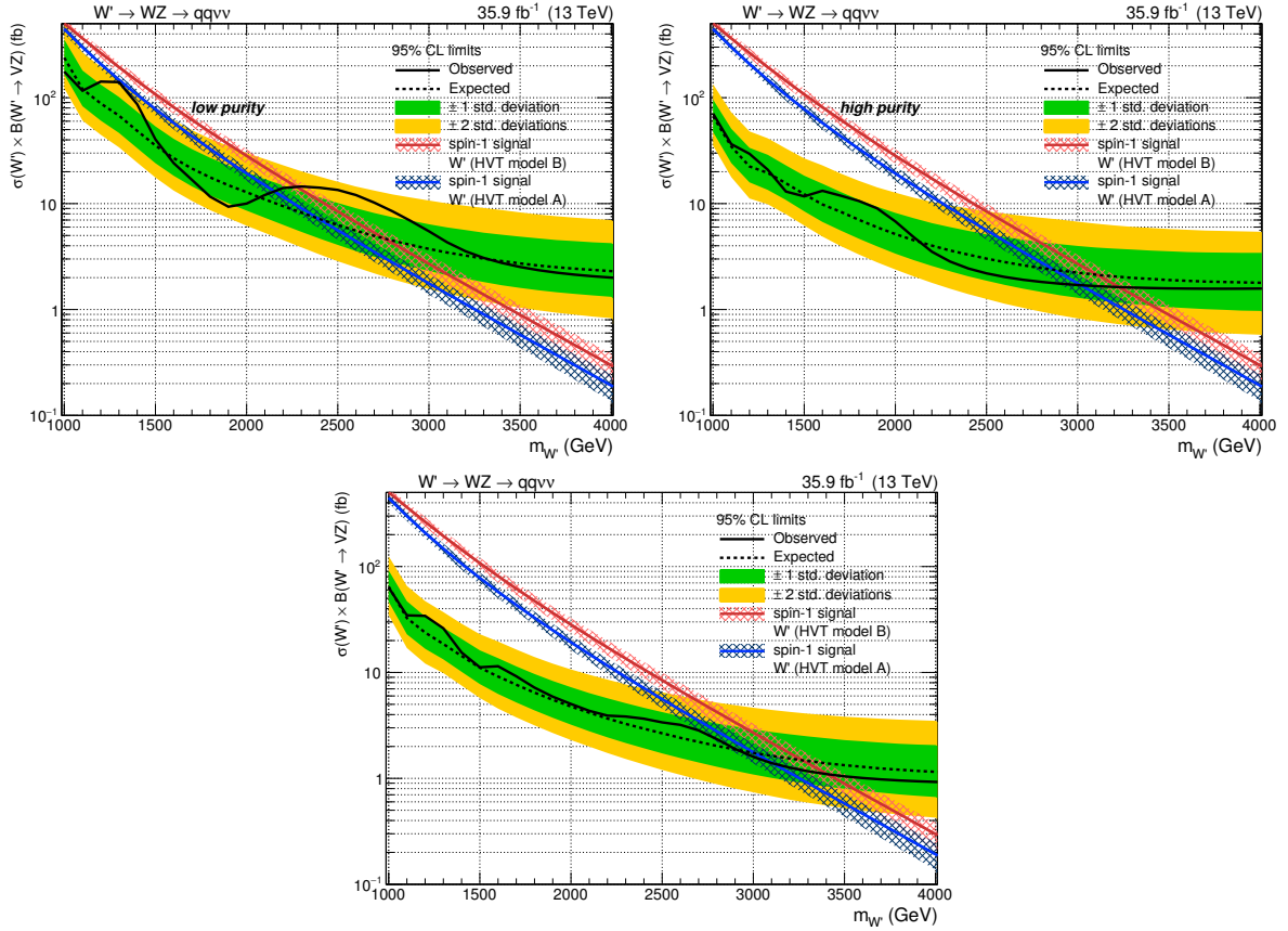
Figure 4.67: Top: observed and expected (with \pm 1(2)\sigma band) 95% C.L. upper limit on \sigma \mathcal{B}(W' \rightarrow W_{\text{had}} Z_{\text{inv}}) for a spin-1 (HVT) signal, for low-purity (left) and high-purity (right) categories, including all statistical and systematic uncertainties. Background predictions are extracted with the \alpha method. Bottom: observed and expected (with \pm 1(2)\sigma band) 95% C.L. upper limit on \sigma \mathcal{B}(W' \rightarrow W_{\text{had}} Z_{\text{inv}}) for a spin-1 (HVT) signal, combining the two purity categories.
