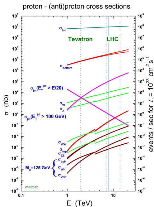
Figure 3.5: Cross-sections and number of expected events in proton-proton collisions, as a function of the center-of-mass energy. Rare phenomena, such as the Higgs boson production, can be observed at the LHC. [55]
