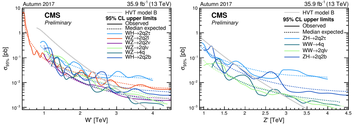
Figure 2.10: The observed and expected limits on the product of the cross-section and branching fraction \sigma\mathcal{B}(W' \rightarrow (WZ, WH)) for a spin-1 W' (left) and \sigma\mathcal{B}(Z' \rightarrow (ZH, WW)) for a spin-1 Z' (right), as a function of the reconstructed mass of the diboson resonance. [33] The gray line shows the theoretical prediction for the HVT model B. The light blue curve corresponds to the HH \rightarrow b\bar{b}\tau^+\tau^- , (WH, ZH) \rightarrow q\bar{q}\tau^+\tau^- analysis [31]; the dark orange curve corresponds to the ZW, ZZ \rightarrow \ell\bar{\ell}q\bar{q} analysis [28]; the light green curve corresponds to the WZ, WW \rightarrow \ell\nu q\bar{q} analysis [30]; the dark green curve corresponds to the (WZ, WW) \rightarrow q\bar{q}q\bar{q} analysis [24, 25]; the dark blue curve corresponds to the (WH, ZH) \rightarrow q\bar{q}b\bar{b} analysis [26, 27]; finally, the violet curve corresponds to the analysis discussed in this thesis [32].
