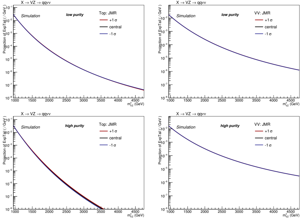
Figure 4.58: Shape variations due to jet mass resolution obtained in the Top (left) and diboson (right) backgrounds, in the low-purity (top) and high-purity (bottom) category.
