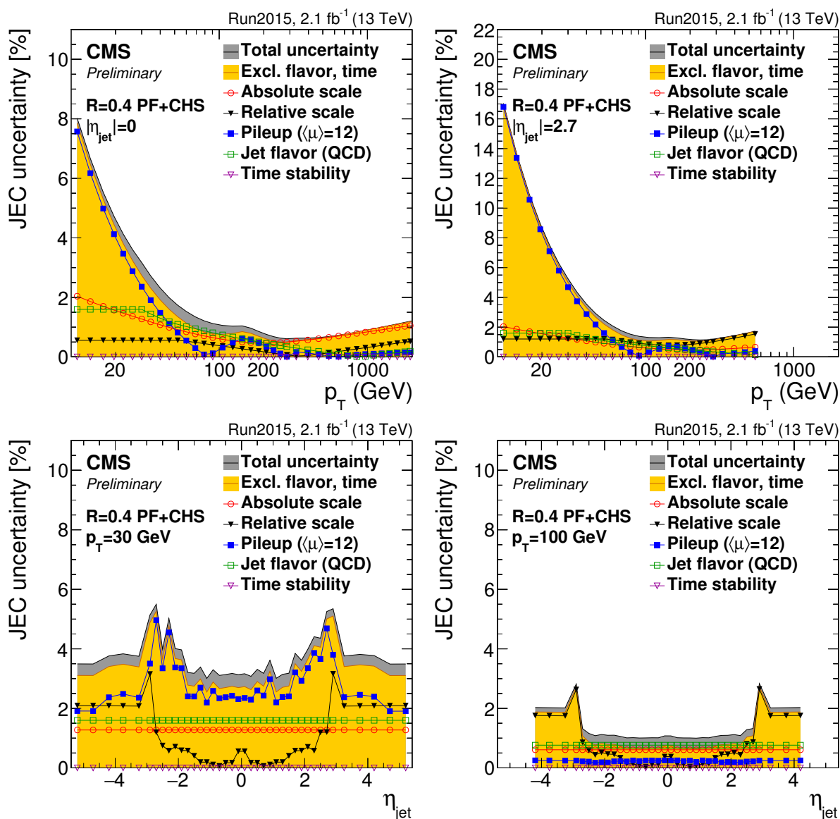
Figure 3.15: Jet energy corrections uncertainties, as a function of jet p_T (top) and \eta (bottom), calculated in 2015 data. The yellow histograms report the convolution of the uncertainties applied in the analysis. [81]
