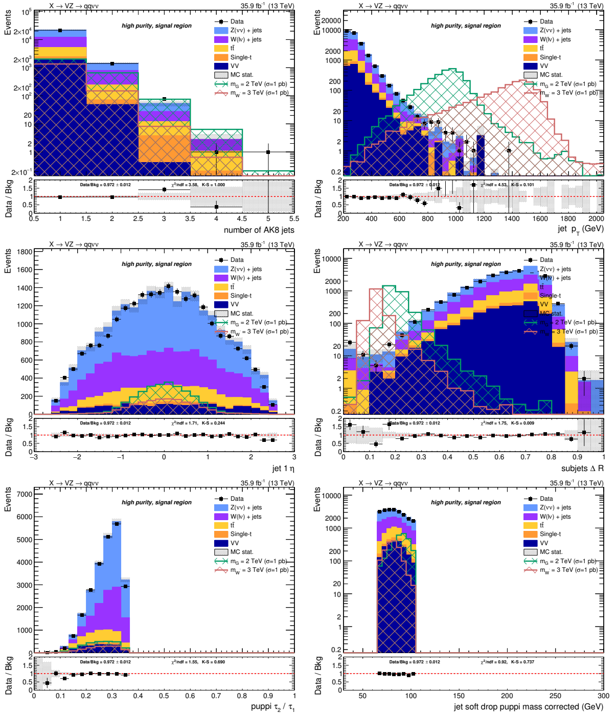
Figure 4.34: Top: number of AK8 jets in the event (left) and V jet candidate p_T (right). Center: V jet candidate \eta (left) and angular separation \Delta R between the constituents leading subjects (right). Bottom: V jet candidate \tau_{21} subjeetiness after PUPPI correction (left) and V jet candidate soft drop PUPPI mass (right). Events are selected with the high-purity signal region selection, and simulated backgrounds are normalized to luminosity.
