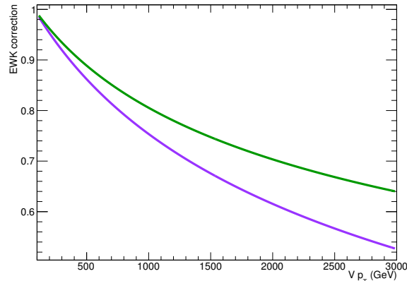
Figure 4.10: Electroweak corrections for the Z (green line) and W boson (purple line) as a function of the transverse momentum of the boson [101].
