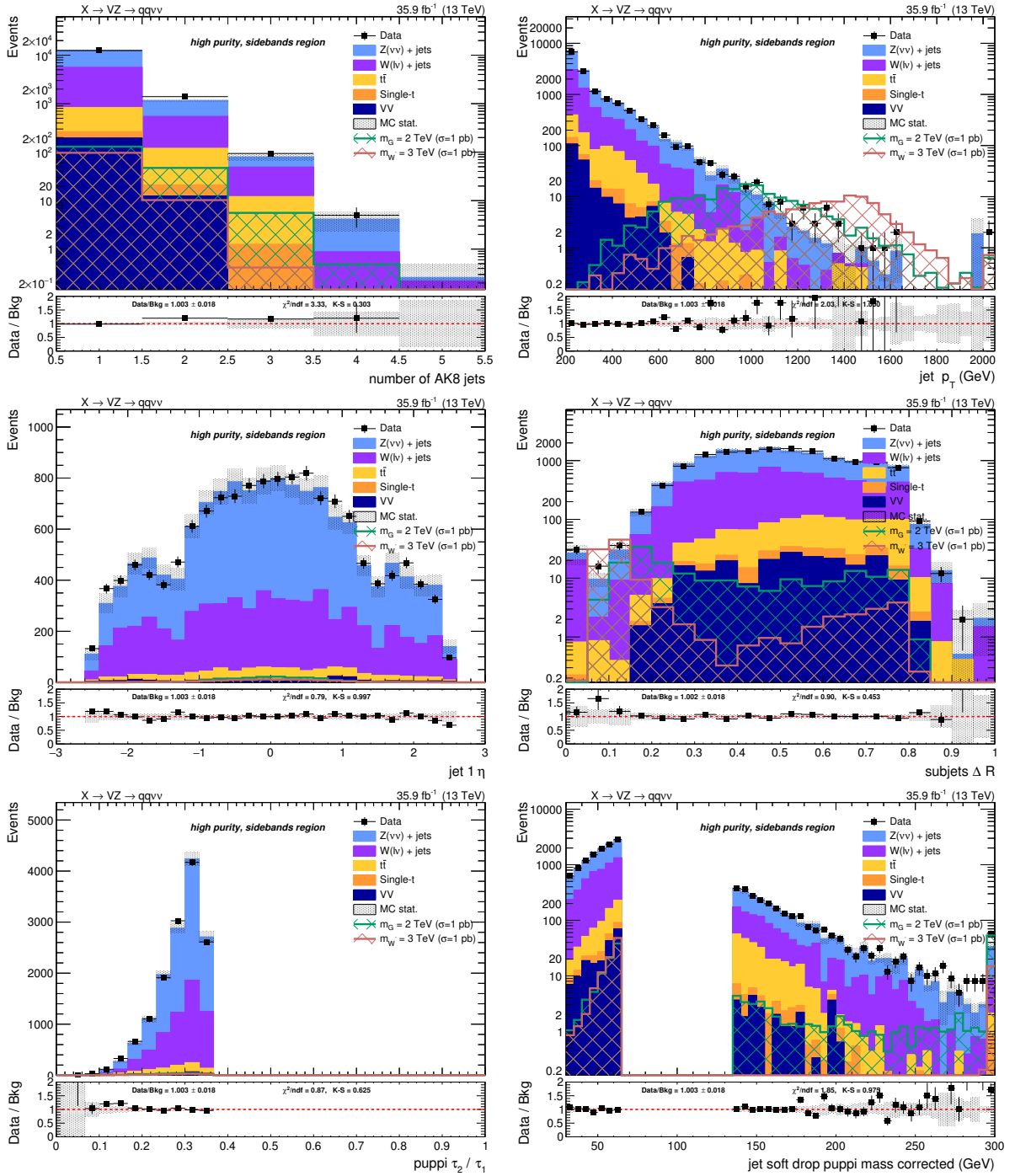
Figure 4.30: Top: number of AK8 jets in the event (left) and V jet candidate p_T (right). Center: V jet candidate \eta (left) and angular separation \Delta R between the constituents leading subjects (right). Bottom: V jet candidate \tau_{21} subjeettiness after PUPPI correction (left) and V jet candidate soft drop PUPPI mass (right). Events are selected with the high-purity sidebands selection, and simulated backgrounds are normalized to luminosity.
