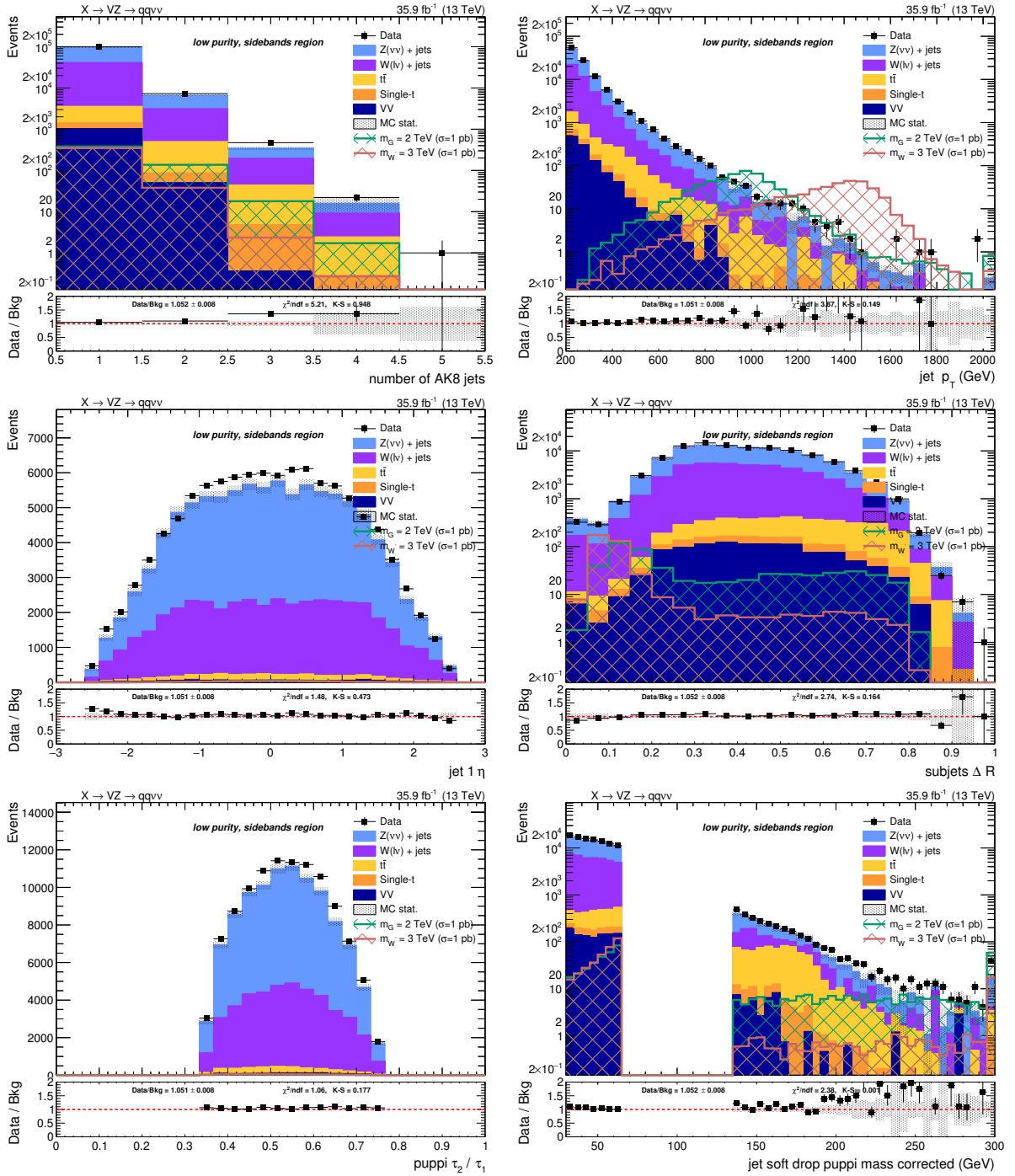
Figure 4.28: Top: number of AK8 jets in the event (left) and V jet candidate p_T (right). Center: V jet candidate \eta (left) and angular separation \Delta R between the constituents leading subjects (right). Bottom: V jet candidate \tau_{21} subjeettiness after PUPPI correction (left) and V jet candidate soft drop PUPPI mass (right). Events are selected with the low-purity sidebands selection, and simulated backgrounds are normalized to luminosity.
