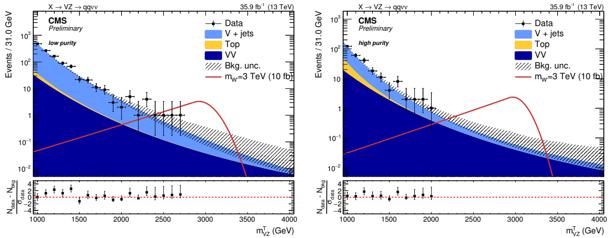
Figure 4.43: Expected background predicted with the \alpha method in the low- (left) and high-purity category (right), compared to observations (black markers) and a signal hypothesis of a spin-1 W' of mass 3 TeV.
