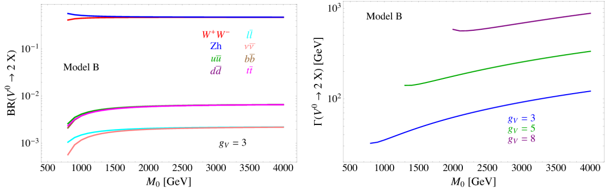
Figure 2.2: HVT model B scenario: branching fractions for fermionic and bosonic decays when g_V = 3 (left) as a function of the mass of the resonance M_0 ; total width of the resonance, as a function of its mass, considering different values of the parameter g_V (right). [14]
