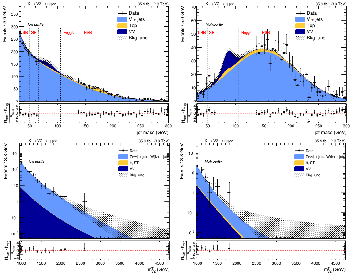
Figure 4.47: Top: results of the fit to the m_V spectrum in data, in the sidebands defined for the \alpha method validation: low-sideband ( 30 < m_V < 50 GeV) and high-sideband ( m_V > 135 GeV) (left: low-purity category, right: high-purity category). Bottom: results of the fits to the m_{VZ}^T spectrum, in the pseudo-signal region ( 50 < m_V < 65 GeV) defined for the \alpha method validation (left: low-purity category, right: high-purity category). Both the true signal region and the Higgs regions are kept blind.
