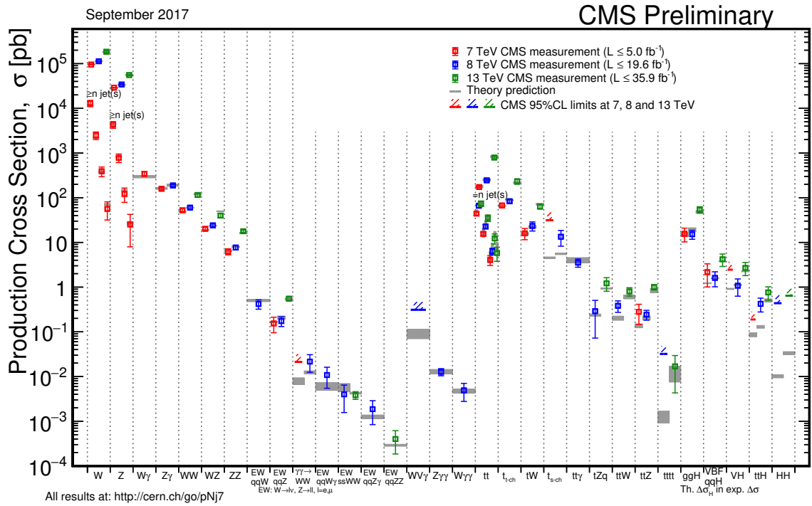
Figure 4.8: Production cross-sections of the main standard model processes, as measured by CMS, and theoretical predictions. [97]
