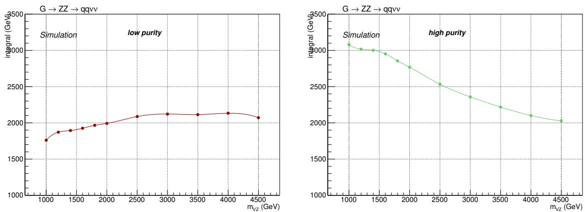
Figure 4.55: Interpolation of the signal normalization as a function of the resonance mass, for a spin-2 (bulk graviton) signal hypothesis. From left to right: low-purity, high-purity.
