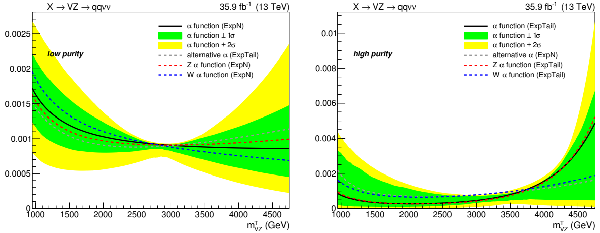
Figure 4.46: Validation of the \alpha method: \alpha functions calculated for Z + \text{jets} background (red dotted line) and for W + \text{jets} background (blue dotted line) separately, and \alpha function for the total V + \text{jets} background (black solid line). Left: low-purity category; right: high-purity category.
