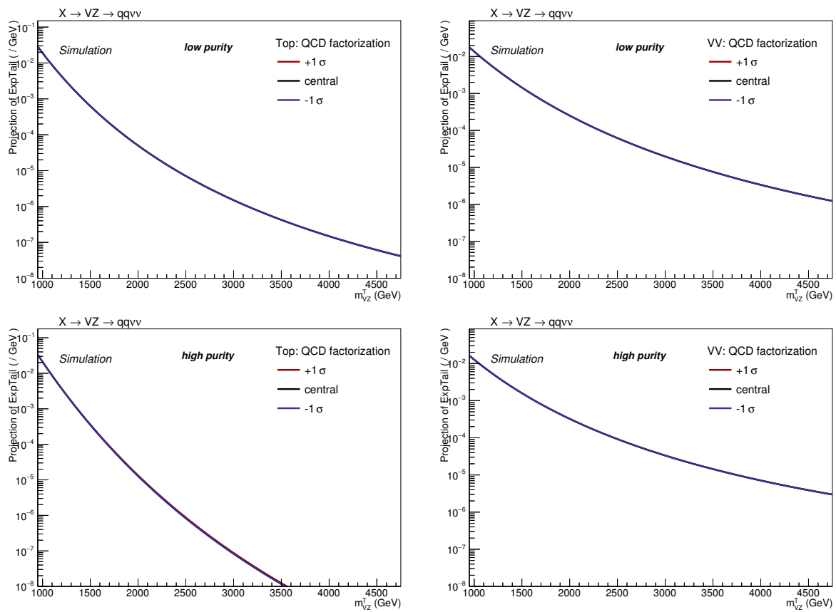
Figure 4.61: Shape variations due to QCD factorization in the Top (left) and diboson (right) backgrounds, in the low-purity (top) and high-purity (bottom) category.
