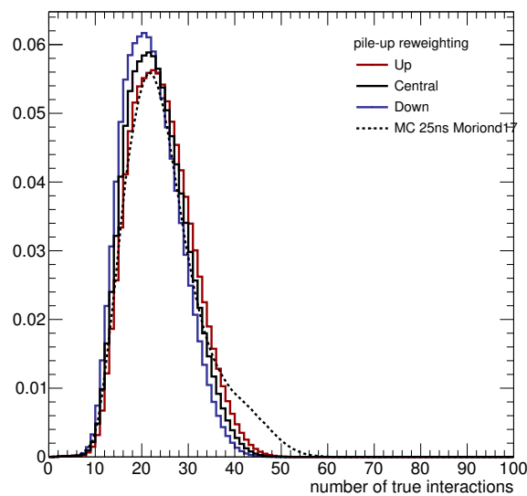
Figure 4.59: Pile-up scenario in 2016 data (black curve), and scenarios obtained by shifting up (red curve) or down (blue curve) the central value of the total inelastic cross-section (69.2 mb), compared to pile-up distribution simulated in Monte Carlo samples (dotted curve).
