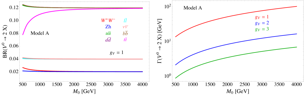
Figure 2.1: HVT model A scenario: branching fractions for fermionic and bosonic decays when g_V = 1 (left) as a function of the mass of the resonance M_0 ; total width of the resonance, as a function of its mass, considering different values of the parameter g_V (right). [14]
