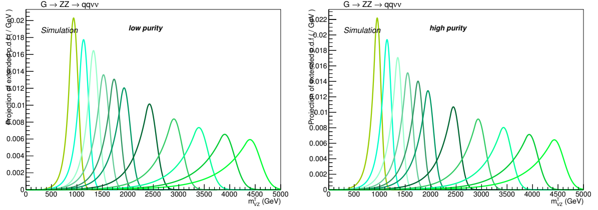
Figure 4.49: Interpolation of the signal as a function of the resonance transverse mass m_{VZ}^T , for a spin-2 (bulk graviton) signal hypothesis with an arbitrary cross section of 1 pb in the low- (left) and high-purity category (right). Signal distributions are normalized to unity.
