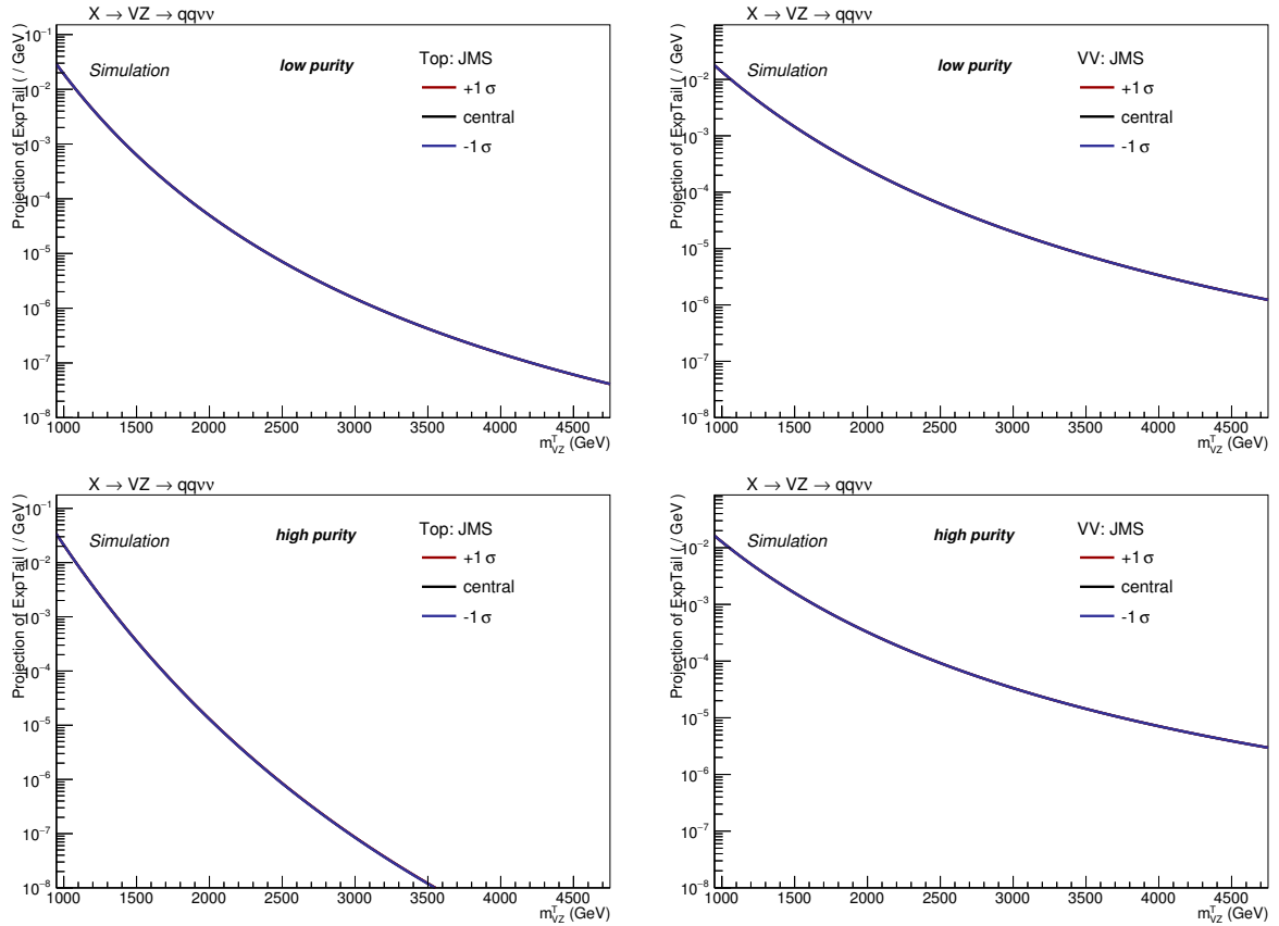
Figure 4.57: Shape variations due to jet mass calibration corrections obtained in the Top (left) and diboson (right) backgrounds, in the low-purity (top) and high-purity (bottom) category.
