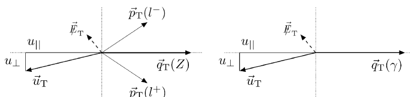
Figure 3.19: Left (Right): kinematics of Z \rightarrow \ell\ell (photon) events in the (r, \varphi) plane; \vec{u}_T is the hadronic recoil, \vec{q}_T is the transverse momentum of the considered boson. [85]
