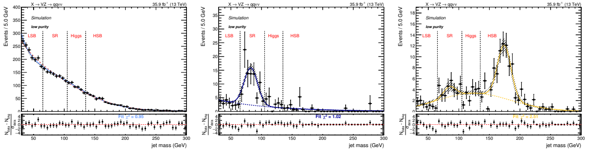
Figure 4.36: Fit to the simulated m_V in the low-purity category for the three backgrounds: V + \text{jets} (left), VV (center), Top (right). For the main background prediction, the alternative function is displayed with a dotted red line, superimposed to the main choice (continuous light blue curve).
