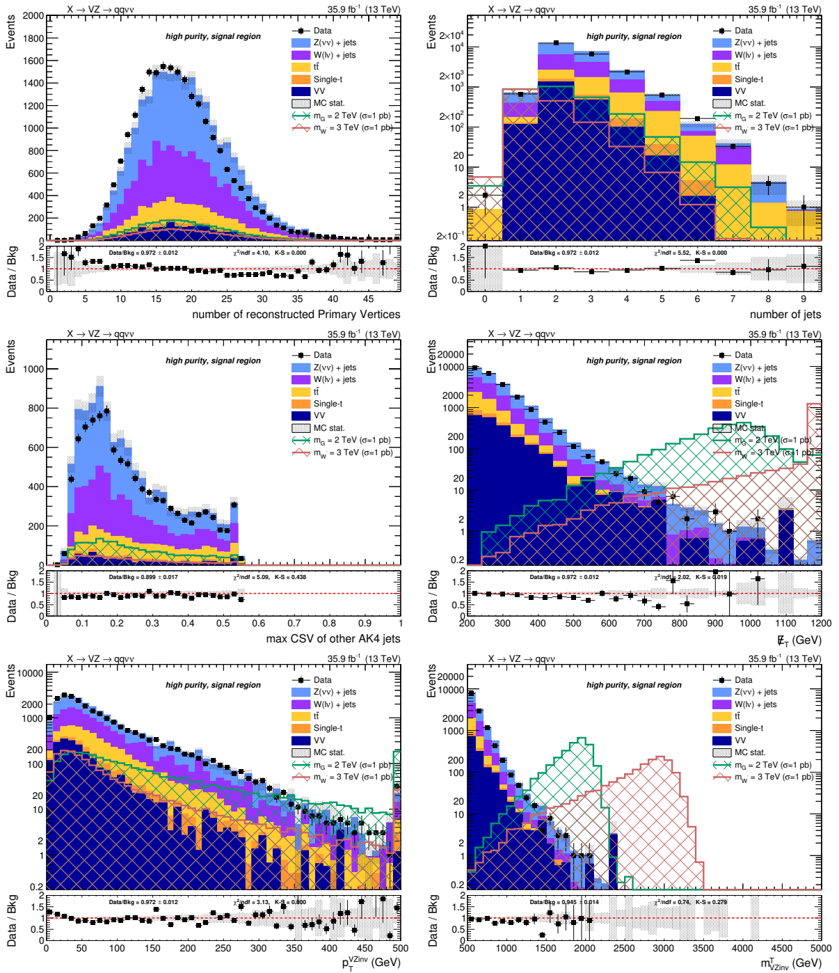
Figure 4.35: Top: number of reconstructed primary vertices (left) and number of AK4 jets in the event (right). Center: distribution of the b-tagging multivariate discriminant for the AK4 jets not included in the V jet cone (left) and E_T^{\text{miss}} distribution (right). Bottom: p_T of the VZ candidate (left) and transverse mass of the VZ candidate (right). Events are selected with the high-purity signal region selection, and simulated backgrounds are normalized to luminosity.
