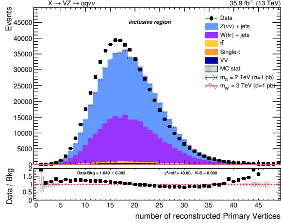
Figure 4.13: Primary vertices multiplicity in data and MC samples, after reweighting.
