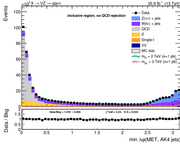
Figure 4.24: Distribution of the minimum azimuthal separation between \vec{p}_T^{\text{miss}} and the momenta of all the AK4 jets present in each event. By imposing \min\Delta\varphi > 0.5 , the QCD background (in gray) is suppressed.
