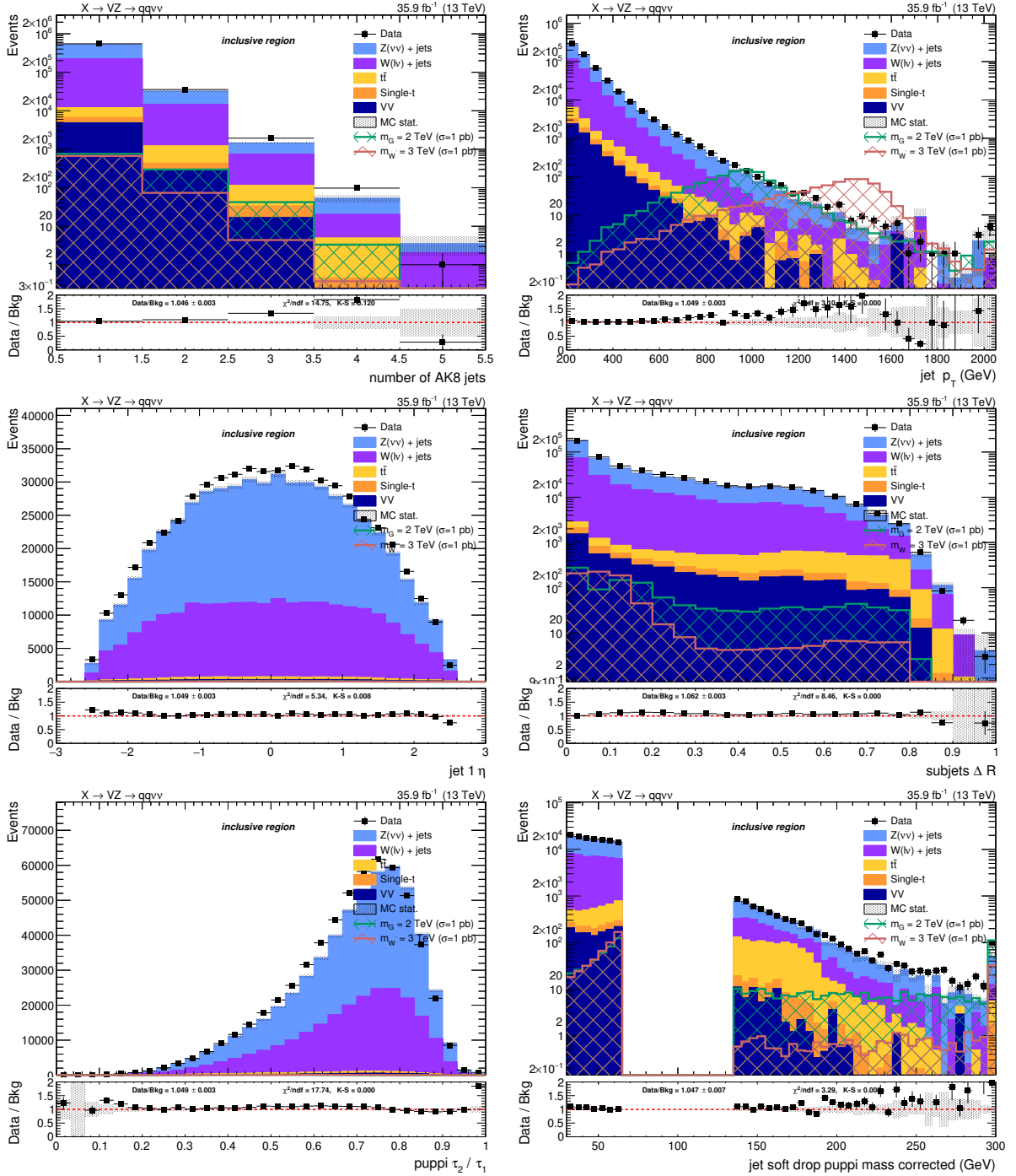
Figure 4.26: Top: number of AK8 jets in the event (left) and V jet candidate p_T (right). Center: V jet candidate \eta (left) and angular separation \Delta R between the constituents leading subjets (right). Bottom: V jet candidate \tau_{21} subjeetiness after PUPPI correction (left) and V jet candidate soft drop PUPPI mass (right). Events are selected with the inclusive selection, and simulated backgrounds are normalized to luminosity.
