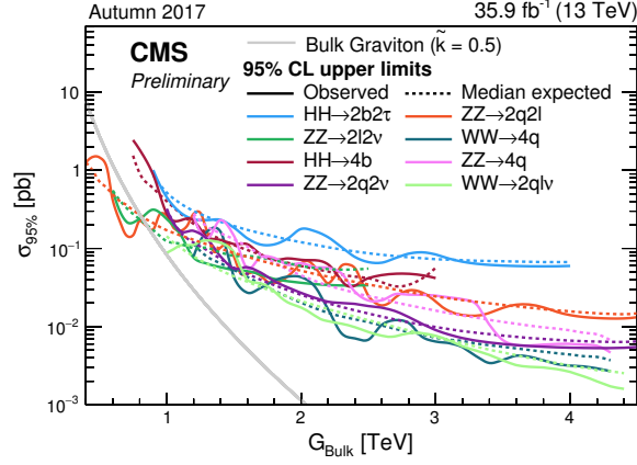
Figure 2.16: The observed and expected limits on the product of the cross-section and branching fraction \sigma \mathcal{B}(G \rightarrow (WW, ZZ)) for a spin-2 bulk graviton, as a function of the reconstructed mass of the diboson resonance. [33] The gray line shows the theoretical prediction for the bulk graviton model, once assumed a curvature parameter \tilde{k} = 0.5 . The light blue curve corresponds to the HH \rightarrow b\bar{b}\tau^+\tau^- , (WH, ZH) \rightarrow q\bar{q}\tau^+\tau^- analysis [31]; the bright green curve corresponds to the ZZ \rightarrow \ell\ell\nu\nu analysis [48]; the dark red curve corresponds to the HH \rightarrow b\bar{b}b\bar{b} analysis [49]; the dark orange curve corresponds to the ZW, ZZ \rightarrow \ell\bar{\ell}q\bar{q} analysis [28]; the dark green curve and the pink curve correspond to two possible final states included in the (WZ, WW) \rightarrow q\bar{q}q\bar{q} analysis [24, 25]; the light green curve corresponds to the WZ, WW \rightarrow \ell\nu q\bar{q} analysis [30]; finally, the violet curve corresponds to the analysis discussed in this thesis [32].
