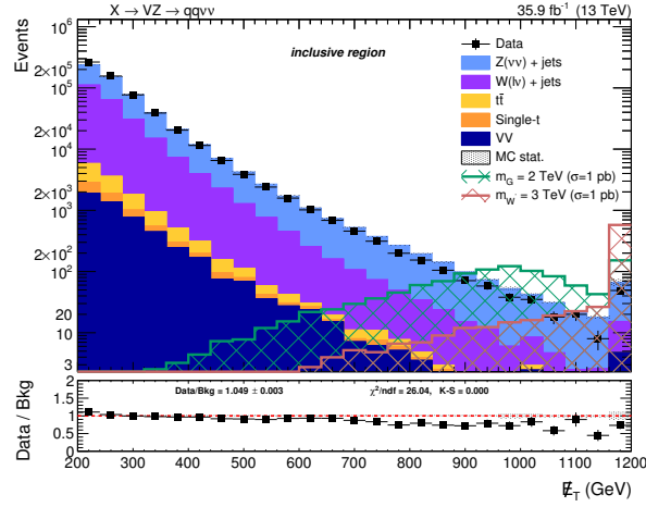
Figure 4.23: Type-1 corrected E_T^{\text{miss}} distribution after inclusive selections.
