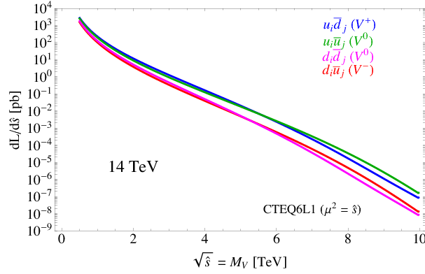
Figure 2.5: Parton luminosities for Drell-Yan production process of a heavy V HVT boson, as a result of the scattering between i and j partons, as a function of the parton center-of-mass energy, for the LHC proton-proton collisions performed at 14 TeV. [14]
