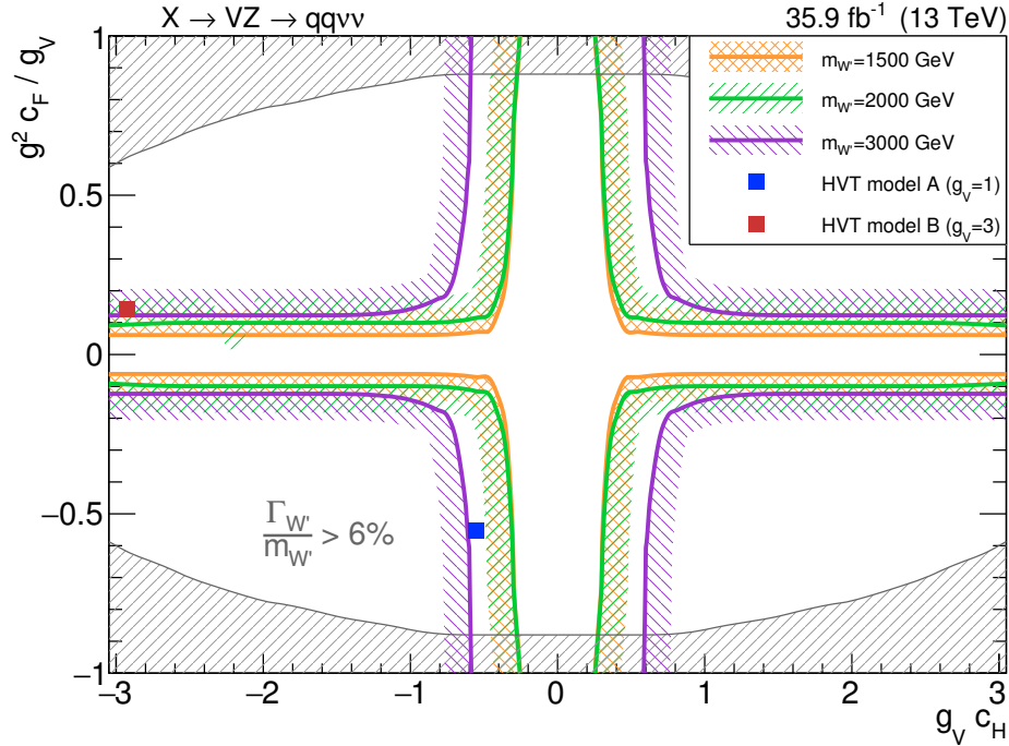
Figure 4.70: Exclusion limits on the parameter space of the HVT model. Coloured curves represent the contours of the parametric region excluded by observations in data, considering a spin-1 W' resonance of mass 1.5 TeV (in orange), 2 TeV (in green), 3 TeV (in violet). Benchmark model A and model B are represented as blue and red markers. The shaded gray area indicates the parameter space where the narrow width approximation fails.
