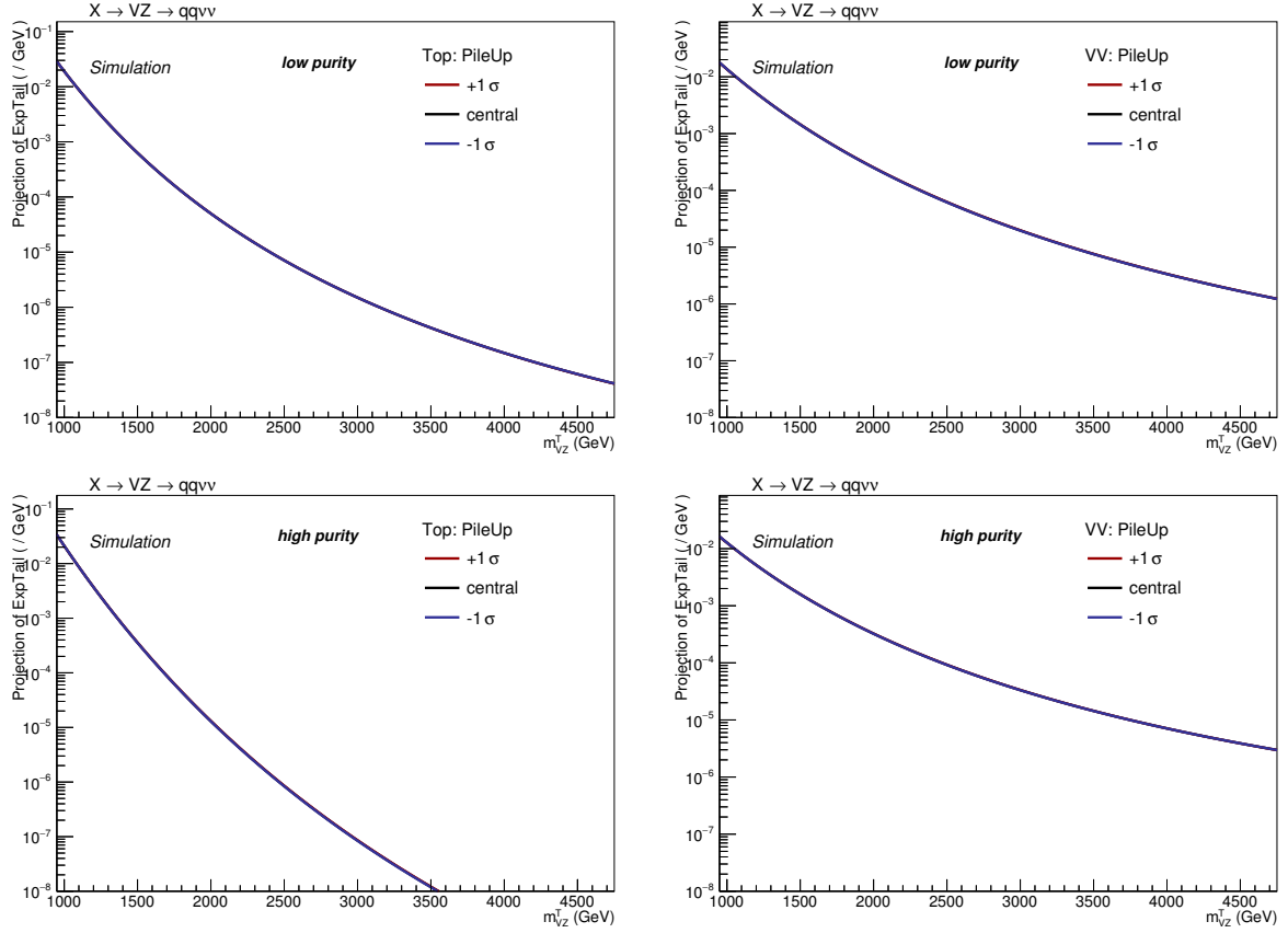
Figure 4.60: Shape variations due to pile-up uncertainty obtained in the Top (left) and diboson (right) backgrounds, in the low-purity (top) and high-purity (bottom) category.
