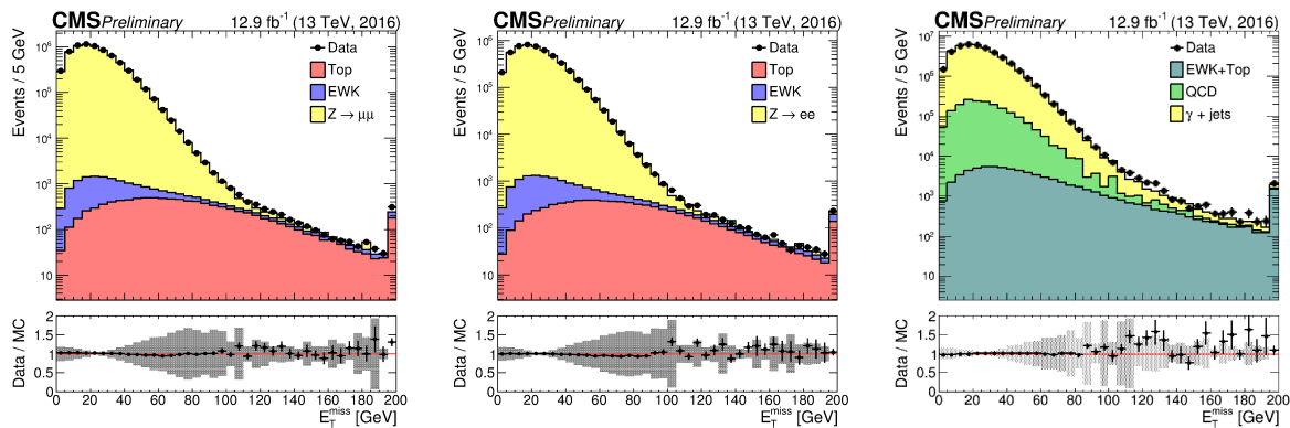
Figure 3.18: Data (black markers) and Monte Carlo (histograms) distributions of E_T^{\text{miss}} variable, in events reconstructing respectively a Z \rightarrow \mu\mu decay (left), a Z \rightarrow ee decay (center), an isolated photon (right). [85]
