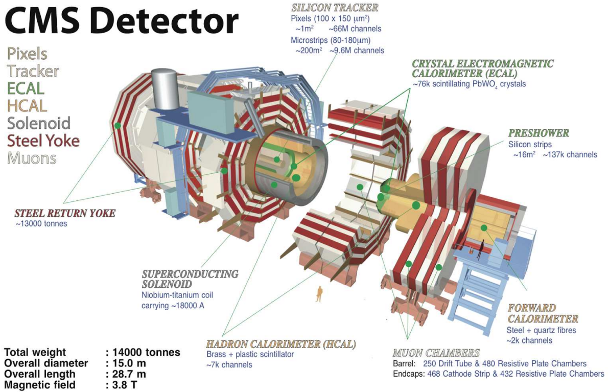
Figure 3.6: The CMS experiment. [56]
