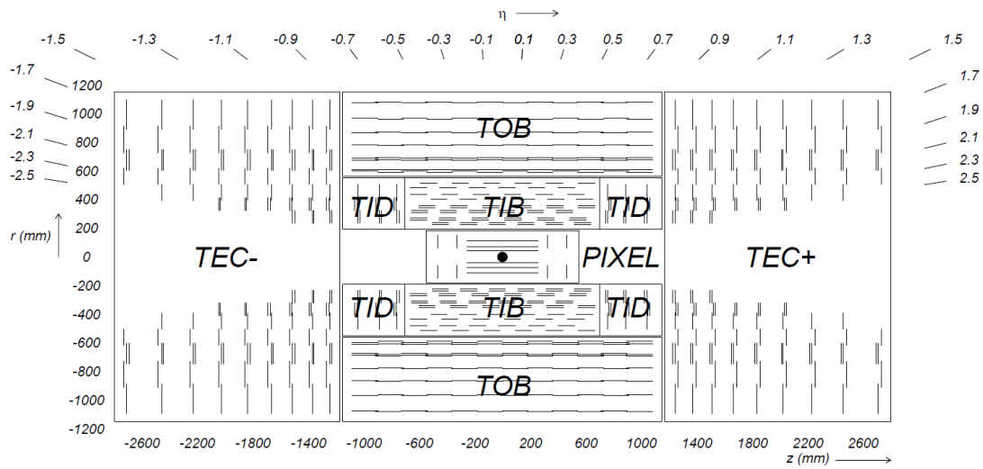
Figure 3.10: The CMS tracking system: the inner pixel detector, close to the interaction point, and the outer strip detector. [56]
