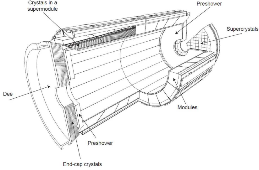
Figure 3.11: The CMS electromagnetic calorimeter. [56]
