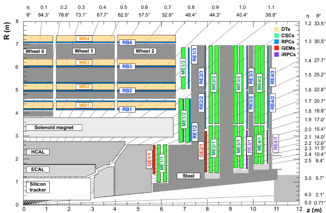
Figure 3.13: Section of CMS detector, in the plane (r, z) , parallel to the beamline, that emphasizes the location of the muon detectors, in particular: Drift Tubes (DT, in yellow); Cathode Strip Chambers (CSC, in green); Resistive Plate Chambers (RPC, in blue). [56]
