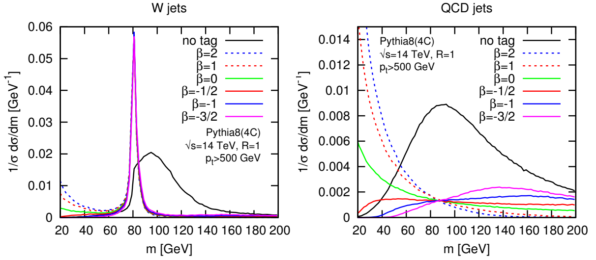
Figure 4.17: Distributions of the jet mass in W + jet signal simulations (left) and multi-jet QCD background (right), before (in black) and after applying soft drop algorithm. Each curve corresponds to a different value of the parameter \beta . [103]
