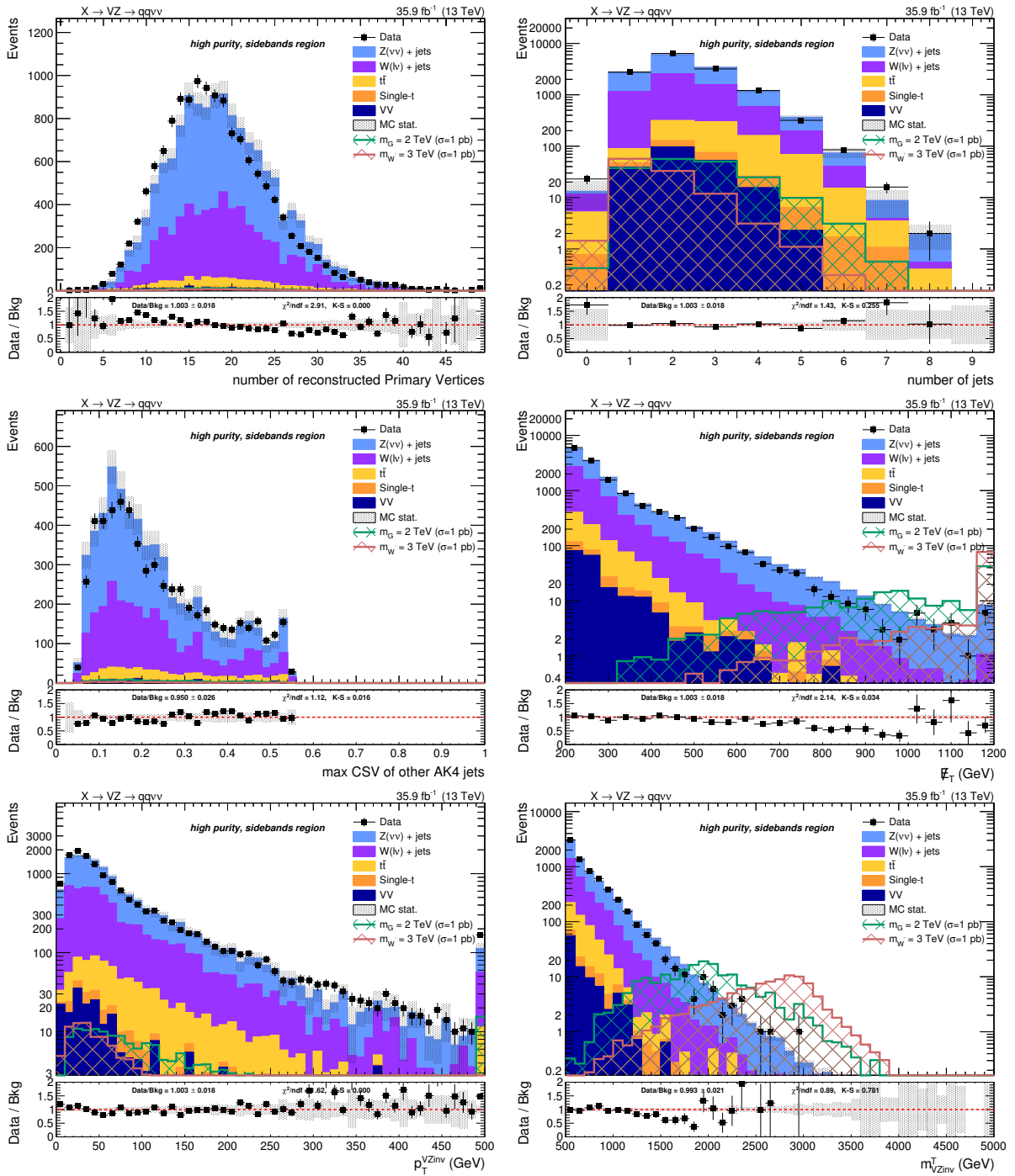
Figure 4.31: Top: number of reconstructed primary vertices (left) and number of AK4 jets in the event (right). Center: distribution of the b-tagging multivariate discriminant for the AK4 jets not included in the V jet cone (left) and E_T^{\text{miss}} distribution (right). Bottom: p_T of the VZ candidate (left) and transverse mass of the VZ candidate (right). Events are selected with the high-purity sidebands selection, and simulated backgrounds are normalized to luminosity.
