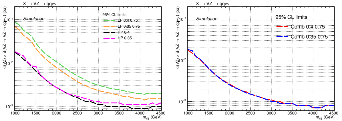
Figure 4.22: Exclusion limit on cross-section time branching fraction at 95% CL of bulk graviton signals, computed by applying different \tau_{21} categorizations, considering the categories separately (left) and combining them together (right), as a function of the resonance mass.
