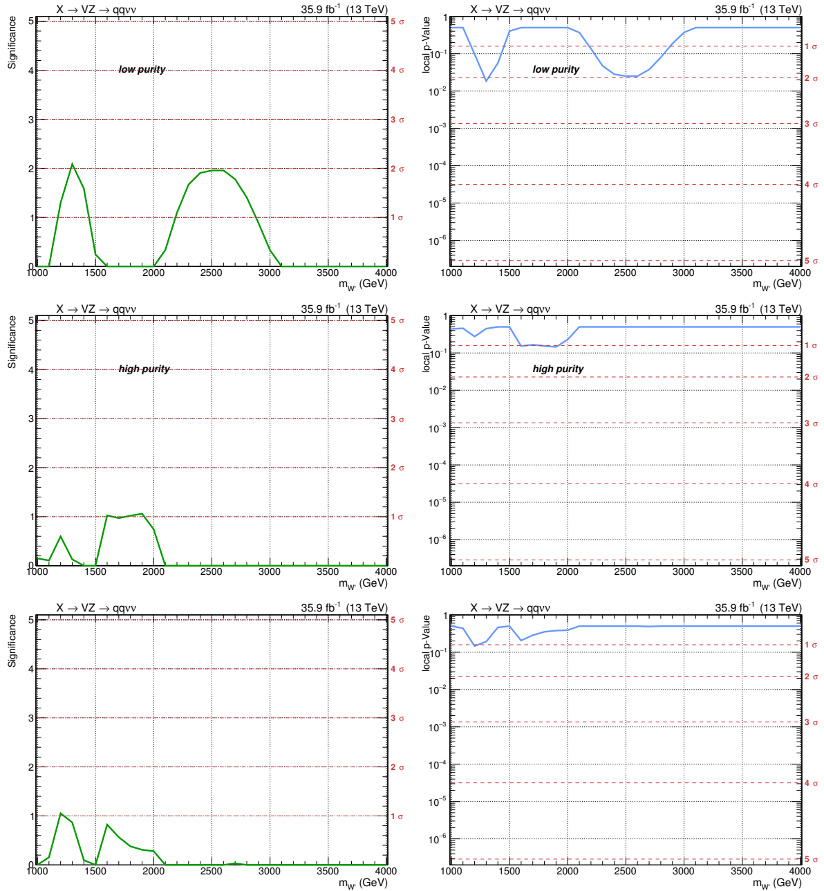
Figure 4.69: Local significances (left plots) and local p-values (right plots) as a function of the resonance mass, for a spin-1 W' hypothesis, in the low- (top), high-purity categories (center), and in the combination of the categories (bottom).
