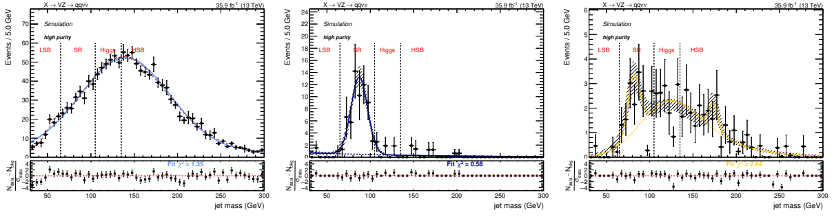
Figure 4.37: Fit to the simulated m_V in the high-purity category for the three backgrounds: V + jets (left), VV (center), Top (right). For the main background prediction, the alternative function is displayed with a dotted red line, superimposed to the main choice (continuous light blue curve).
