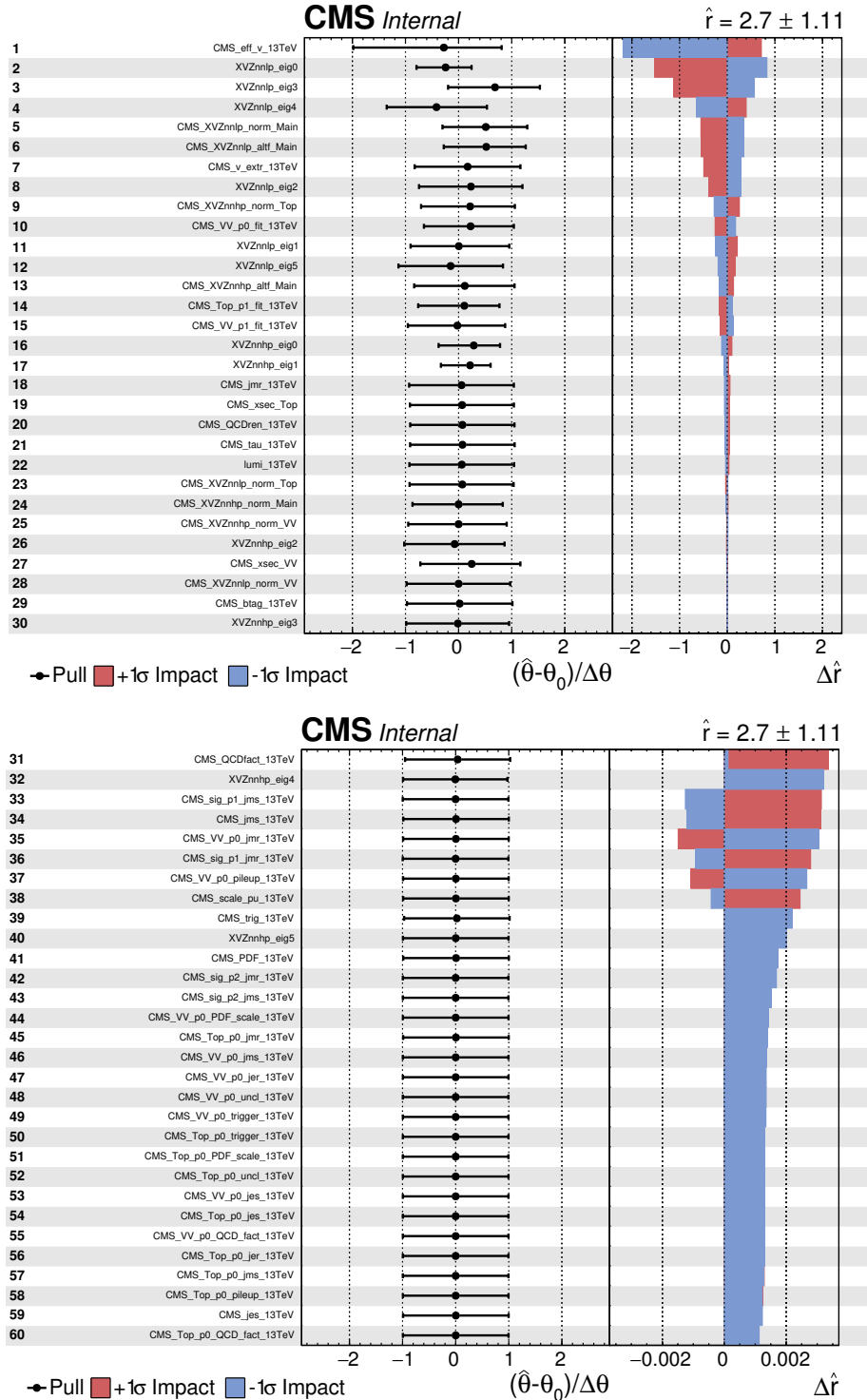
Figure 4.65: Impacts of the nuisance parameters on the signal strength estimation, for the combination of the low- and high-purity categories. A signal hypothesis of a spin-2 bulk graviton of mass 2.5 TeV is considered. \theta_0 is the pre-fit value of the nuisance parameter taken into account; \hat{\theta} is the value of the nuisance parameter after the maximum likelihood fit; \Delta\hat{r} represents the impact, i.e. the shift induced in the parameter of interest (in this case, r , the cross-section times branching fraction, describing the signal strength) as the \theta parameter is fixed and brought to its +1\sigma or -1\sigma post-fit values, with all the other nuisance parameters profiled as log-normal.
