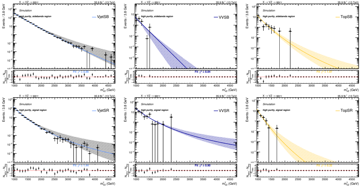
Figure 4.41: High-purity category. Top: fits to the simulated background components V + \text{jets} (left), VV (center), Top (right) in the sidebands (SB). Bottom: fits to the simulated background components V + \text{jets} (left), VV (center), Top (right) in the signal region (SR).
