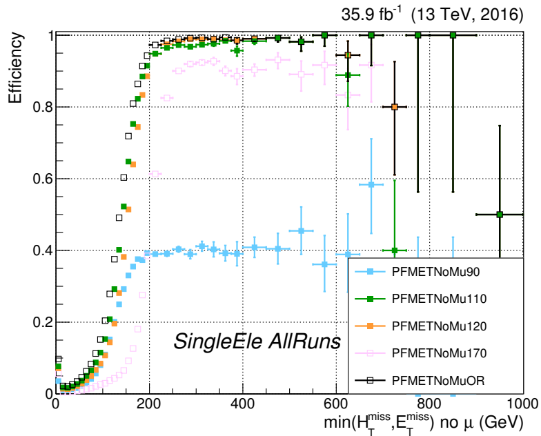
Figure 4.12: \vec{p}_T^{\text{miss}} trigger efficiency for the \vec{p}_T^{\text{miss}} trigger paths used in this analysis, calculated on SingleElectron dataset, as a function of the minimum of the variables E_T^{\text{miss}} (no \mu ) (eq. 4.1) and H_T^{\text{miss}} (eq. 4.2).
