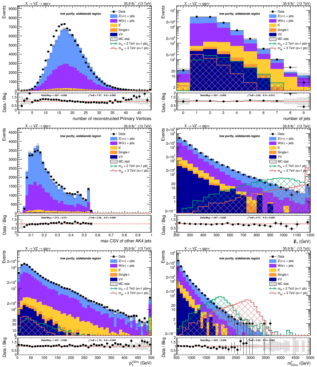
Figure 4.29: Top: number of reconstructed primary vertices (left) and number of AK4 jets in the event (right). Center: distribution of the b-tagging multivariate discriminant for the AK4 jets not included in the V jet cone (left) and E_T^{\text{miss}} distribution (right). Bottom: p_T of the VZ candidate (left) and transverse mass of the VZ candidate (right). Events are selected with the low-purity sidebands selection, and simulated backgrounds are normalized to luminosity.
