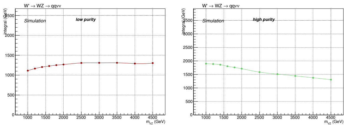
Figure 4.56: Interpolation of the signal normalization as a function of the resonance mass, for a spin-1 ( W' ) signal hypothesis. From left to right: low-purity, high-purity.
