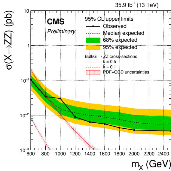
Figure 2.15: The observed and expected limits, with 68% and 95% uncertainty bands, on the product of the cross-section and branching fraction \sigma \mathcal{B}(G \rightarrow ZZ) for a spin-2 bulk graviton, as a function of the reconstructed mass of the diboson resonance. The coloured lines show the theoretical predictions for \tilde{k} = 0.1 and 0.5. [48]
