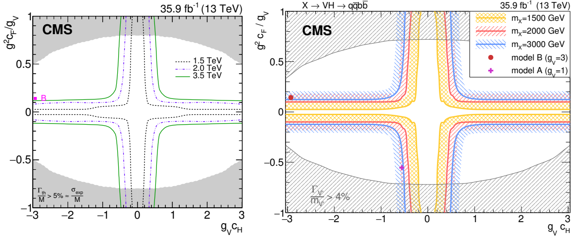
Figure 2.9: Exclusion contours in the coupling parameters plane of the HVT model ( g_V c_H and g_V^2 c_F / g_V ), for [24, 25] analysis (left), and [26, 27] analysis (right).
