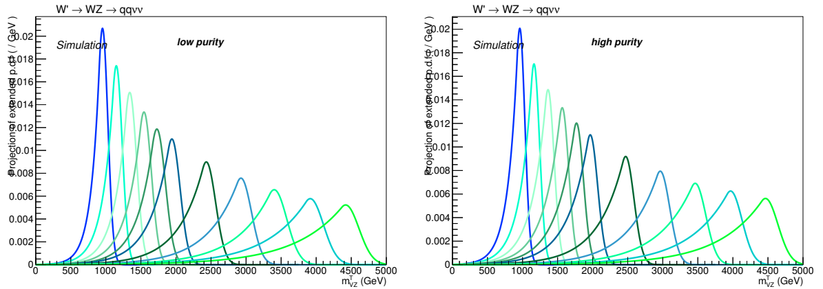
Figure 4.50: Interpolation of the signal as a function of the resonance transverse mass m_{VZ}^T , for a spin-1 ( W' ) signal hypothesis with an arbitrary cross section of 1 pb in the low- (left) and high-purity category (right). Signal distributions are normalized to unity.
