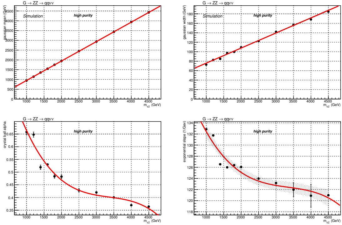
Figure 4.52: Interpolation of the fitted parameters as a function of the resonance mass, for a spin-2 (bulk graviton) signal hypothesis, high-purity category.
