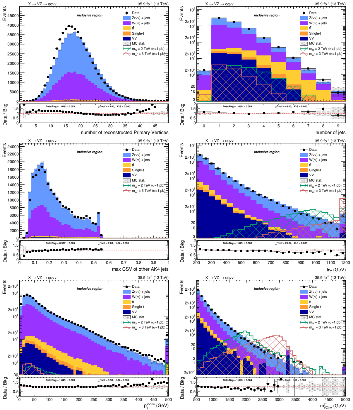
Figure 4.27: Top: number of reconstructed primary vertices (left) and number of AK4 jets in the event (right). Center: distribution of the b-tagging multivariate discriminant for the AK4 jets not included in the V jet cone (left) and E_T^{\text{miss}} distribution (right). Bottom: p_T of the VZ candidate (left) and transverse mass of the VZ candidate (right). Events are selected with the inclusive selection, and simulated backgrounds are normalized to luminosity.
