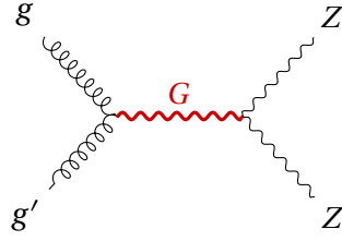
Figure 2.14: Gluon fusion production mechanism for a KK graviton that decays into a couple of Z bosons.
