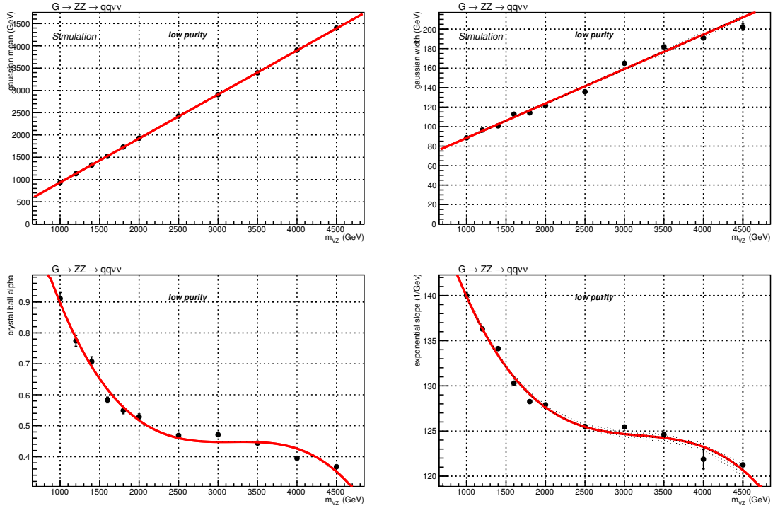
Figure 4.51: Interpolation of the fitted parameters as a function of the resonance mass, for a spin-2 (bulk graviton) signal hypothesis, low-purity category.
