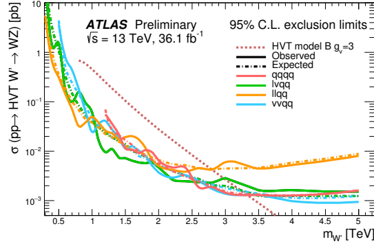
Figure 2.11: The observed and expected limits on the product of the cross-section and branching fraction \sigma \mathcal{B}(W' \rightarrow WZ) for a spin-1 W' , as a function of the reconstructed mass of the diboson resonance. The dark red dotted line shows the theoretical predictions for the HVT model B. [39]
