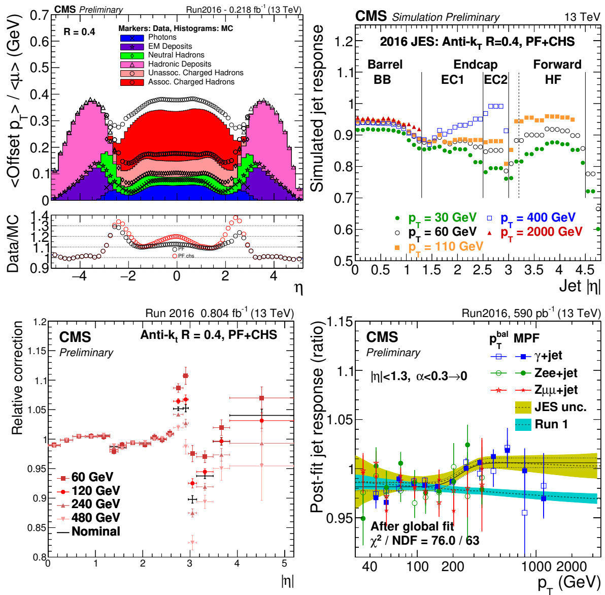
Figure 3.14: Top left: average p_T offset due to additional pile-up events, measured both in data and in MC simulations, as a function of the jet pseudorapidity. Top right: simulated jet response (L2L3 MC-truth corrections), as a function of the jet pseudorapidity. Bottom left: L2L3 residual data-MC corrections, evaluated on di-jet events, as a function of the jet \eta . Bottom right: L2L3 residual data-MC corrections, evaluated on di-jet and Z/\gamma + \text{jet} events, as a function of the jet p_T . [81]
