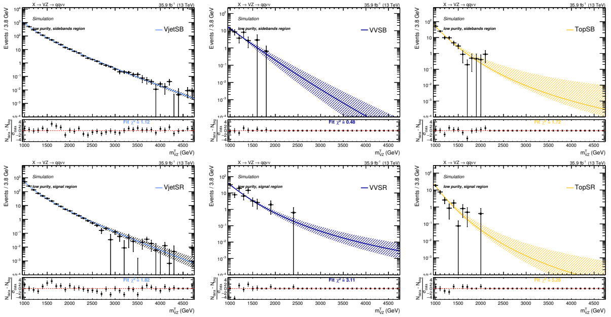
Figure 4.39: Low-purity category. Top: fits to the simulated background components V + \text{jets} (left), VV (center), Top (right) in the sidebands (SB). Bottom: fits to the simulated background components V + \text{jets} (left), VV (center), Top (right) in the signal region (SR).
