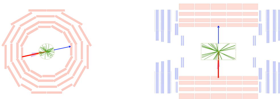
Figure 4.1: Left: representation of the decay of a W' of mass 2.5 TeV, in the transverse plane of the CMS detector. Right: representation of the same event, in the longitudinal plane of the CMS detector.
