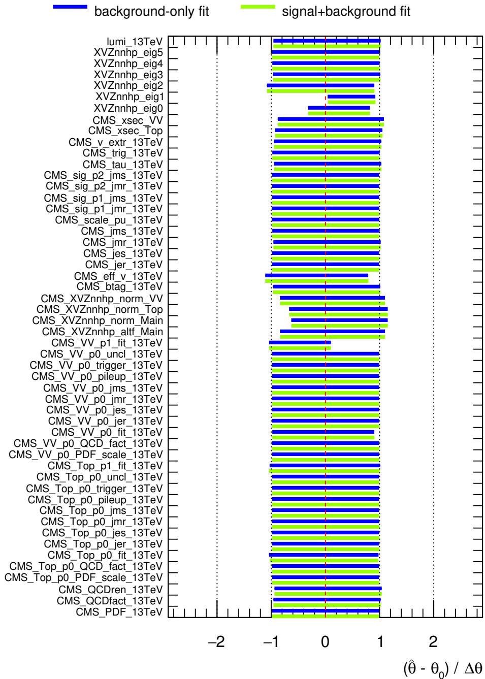
Figure 4.64: Nuisance pulls for the high-purity category, calculated under both the background-only (blue bars) and signal plus background hypotheses (green bars). A signal hypothesis of a spin-2 bulk graviton of mass 3 TeV is considered.
