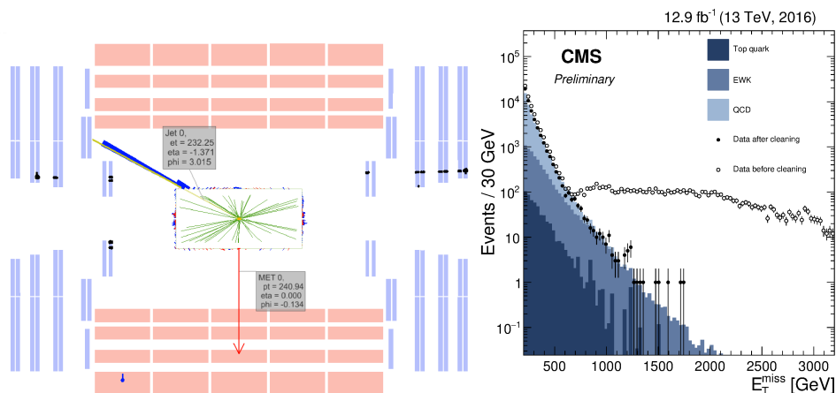
Figure 3.17: Left: event display of beam halo particles hitting the CSC detector. Right: comparison of data and simulations (histograms) when di-jet events are selected, before (open markers) and after (filled markers) anomalous E_T^{\text{miss}} cleaning algorithms have been applied on data. [85]
