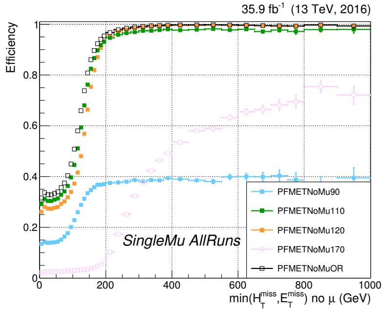
Figure 4.11: \vec{p}_T^{\text{miss}} trigger efficiency for the \vec{p}_T^{\text{miss}} trigger paths used in this analysis, calculated on SingleMuon dataset, as a function of the minimum of the variables E_T^{\text{miss}} (no \mu ) (eq. 4.1) and H_T^{\text{miss}} (eq. 4.2).
