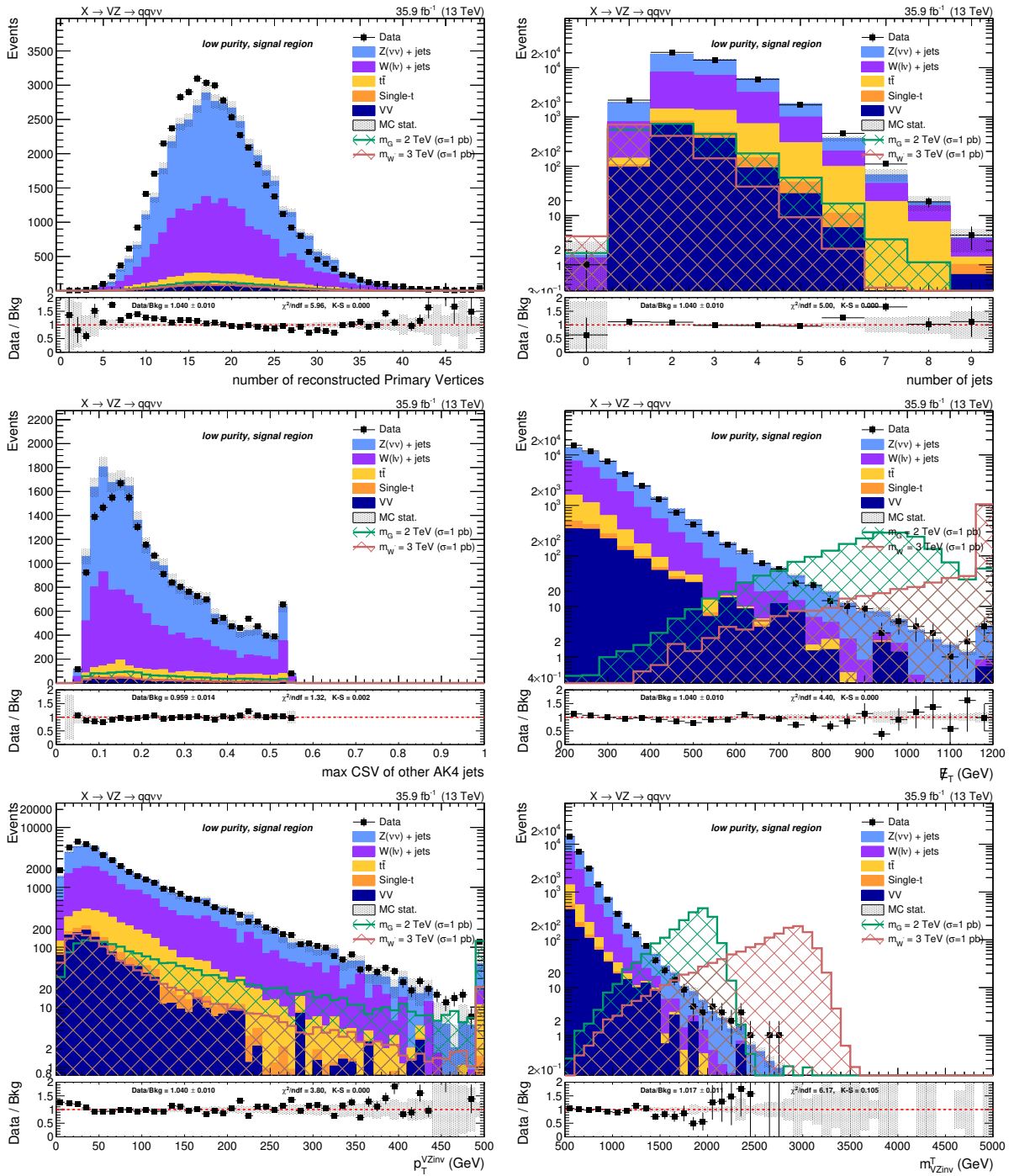
Figure 4.33: Top: number of reconstructed primary vertices (left) and number of AK4 jets in the event (right). Center: distribution of the b-tagging multivariate discriminant for the AK4 jets not included in the V jet cone (left) and E_T^{\text{miss}} distribution (right). Bottom: p_T of the VZ candidate (left) and transverse mass of the VZ candidate (right). Events are selected with the low-purity signal region selection, and simulated backgrounds are normalized to luminosity.
