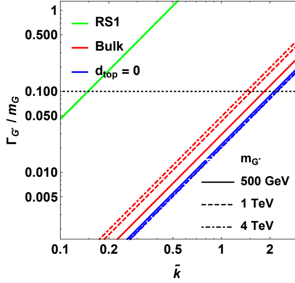
Figure 2.13: Width of the KK gravitons, in units of the mass of the resonance, as a function of the curvature parameter \tilde{k} . The red curves represent the bulk extension of RS1 original model for different mass hypotheses (from 500 GeV up to 4 TeV). [47]
