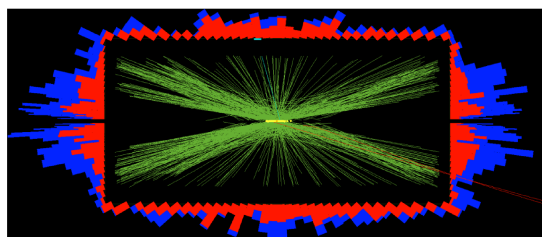
Figure 3.4: CMS collision event, where a record of 78 interactions per single bunch crossing were taking place simultaneously. [54]
