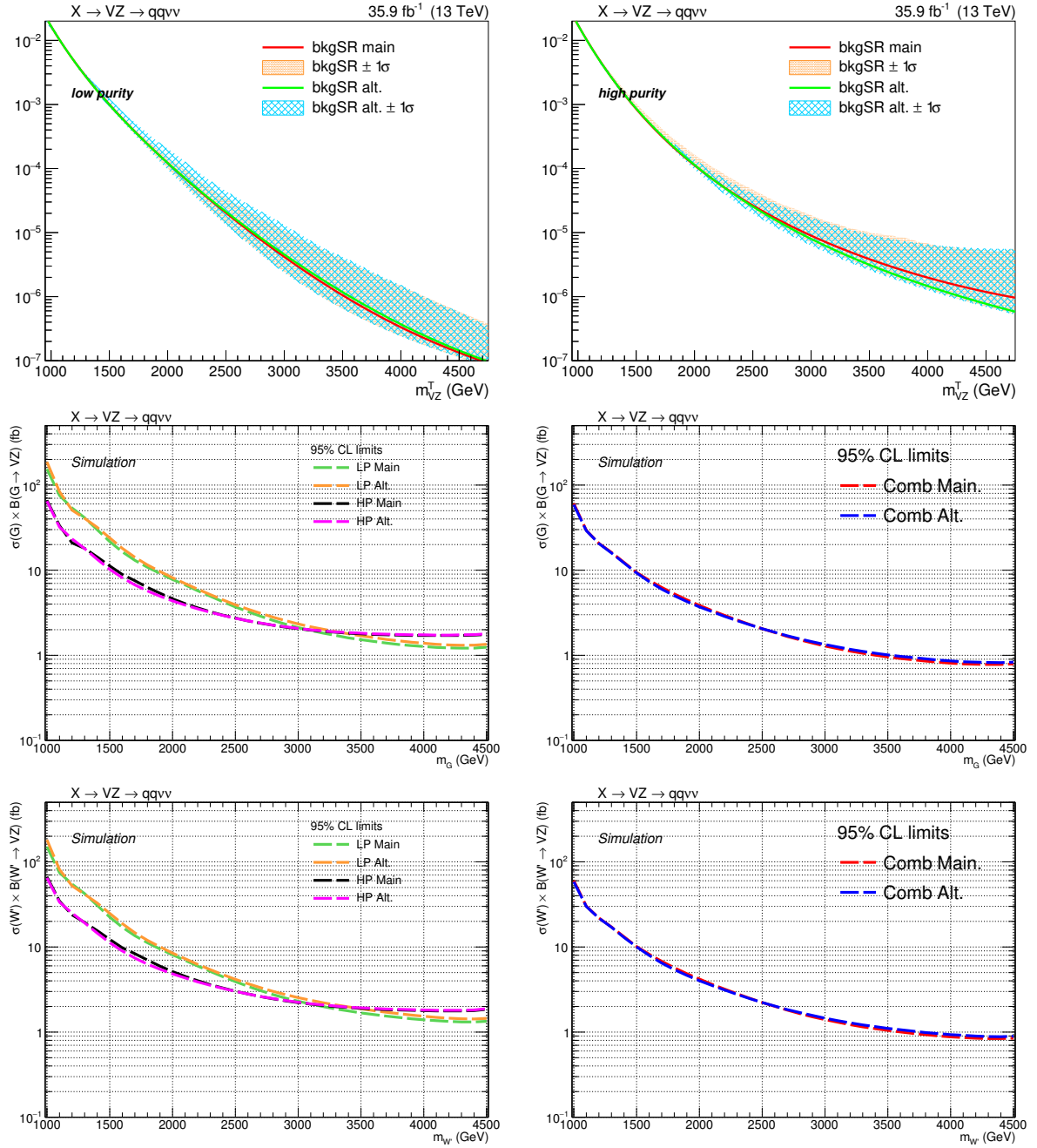
Figure 4.48: Validation of the \alpha method: impact of the choice of the function to describe the dominant V + \text{jets} background. Top: fit results of the background shape prediction in the SR obtained with the main function (red curve) and the alternative function (green curve), for low- (left) and high- (right) purity categories. Center: exclusion limits on cross-section times branching fraction for a spin-2 bulk graviton hypothesis, as a function of the mass of the resonance, calculated by choosing the main function (left plots: green curve for low-purity category alone and black curve for high-purity category alone, right plot: red curve for the combination of the categories) or the alternative function (left plots: orange curve for low-purity category alone and pink curve for high-purity category alone, right plot: blue curve for the combination of the categories). Bottom: exclusion limits on cross-section times branching fraction for a spin-1 W' hypothesis.
