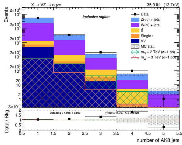
Figure 4.14: Number of reconstructed AK8 jets after inclusive selections.
