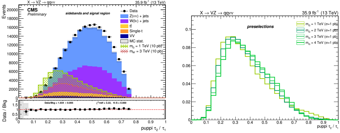
Figure 4.20: Distribution of the \tau_{21} subjettiness of the leading AK8 jet, selected as the hadronically decaying V candidate, for expected SM background and data (left), and for bulk graviton signal (right).
