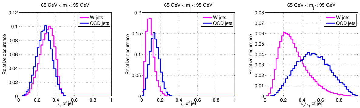
Figure 4.19: Distribution of \tau_1 (left), \tau_2 (center), and \tau_{21} (right) variables, in simulations of a W plus jets process (in pink) and for a multi-jet QCD originated process (in blue). A selection on the leading jet mass is applied: 65 < m_j < 95 GeV; jets are clustered with a parameter R_0 = 0.6 , p_T > 300 GeV, |\eta| < 1.3 [106].
