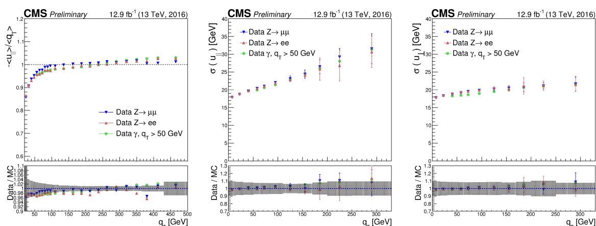
Figure 3.20: Left: E_T^{\text{miss}} response, as a function of the transverse momentum q_T of the vector boson considered in the event ( Z decaying into \mu\mu , Z in ee or a photon), measured on data. Center and right: resolution on the measurement of the parallel and perpendicular hadronic recoil in data, as a function of q_T . [85]
