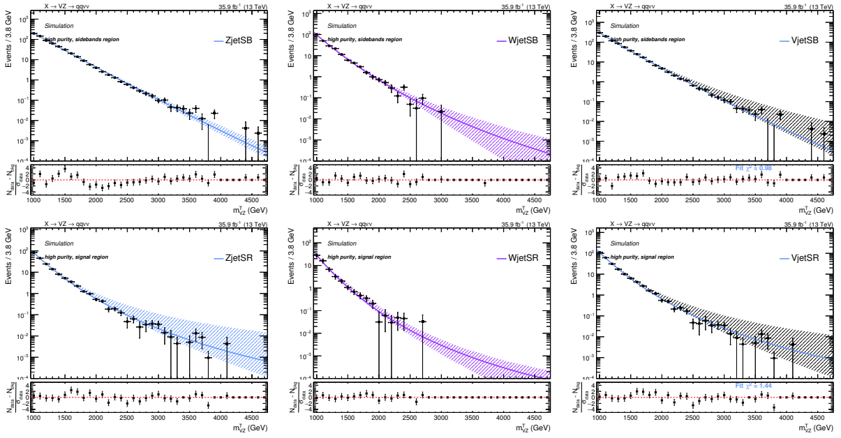
Figure 4.45: Validation of the \alpha method, high-purity category. Top: fits to the simulated background components Z + \text{jets} (left), W + \text{jets} (center), and their combination V + \text{jets} (right), in the sidebands (SB). Bottom: fits to the simulated background components Z + \text{jets} (left), W + \text{jets} (center), and their combination V + \text{jets} (right), in the signal region.
