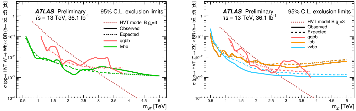
Figure 2.12: The observed and expected limits on the product of the cross-section and branching fraction \sigma \mathcal{B}(W' \rightarrow WH) for a spin-1 W' (left) and \sigma \mathcal{B}(Z' \rightarrow ZH) for a spin-1 Z' (right), as a function of the reconstructed mass of the diboson resonance. The dark red dotted lines show the theoretical predictions for the HVT model B. [39]
