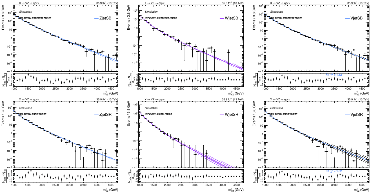
Figure 4.44: Validation of the \alpha method, low-purity category. Top: fits to the simulated background components Z + jets (left), W + jets (center), and their combination V + jets (right), in the sidebands (SB). Bottom: fits to the simulated background components Z + jets (left), W + jets (center), and their combination V + jets (right), in the signal region.
