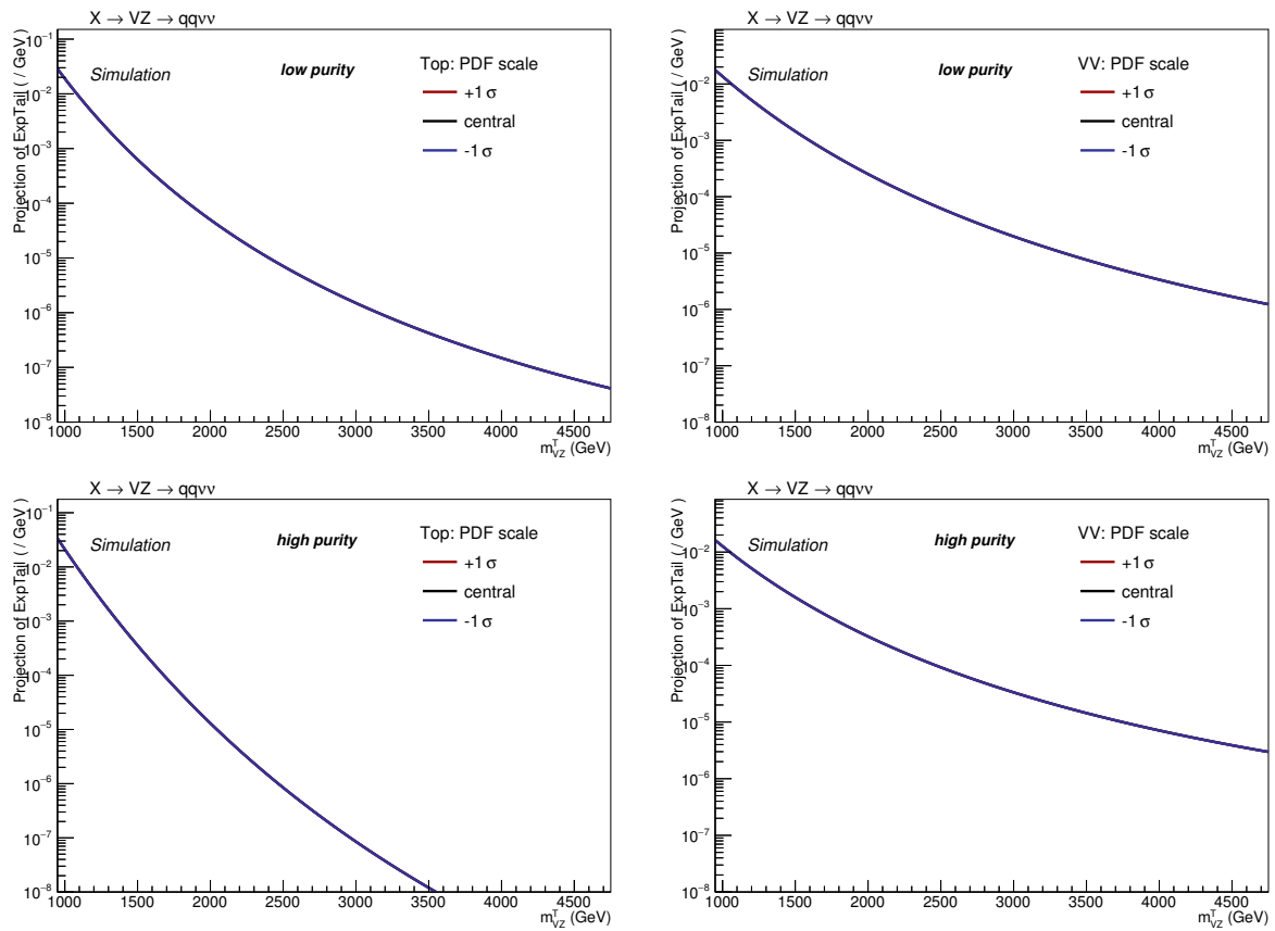
Figure 4.62: Shape variations due to PDF scale in the Top (left) and diboson (right) backgrounds, in the low-purity (top) and high-purity (bottom) category.
