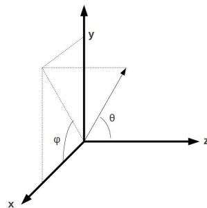
Figure 3.8: The CMS coordinate system. [57]
