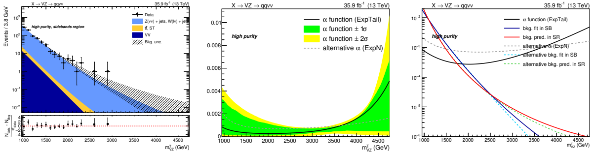
Figure 4.42: High-purity category. Result of the fit to data in the SB (left), \alpha -ratio function (center), and \alpha function compared to the background shape in both SB and SR (right). The black line, with the corresponding 1\sigma (green) and 2\sigma (yellow) uncertainty bands, represents the \alpha function. The gray line is the alternative \alpha function. The pinched region in the uncertainty bands is due to the normalization of the probability density functions entering the numerator and denominator of the \alpha -ratio: given the unitarity constraint, the \alpha function is forced to subtend the same area while varying within the uncertainties of each parameter, hence it is only allowed to oscillate at the extremes of the spectrum. The blue and red solid lines represent the estimated background in the SB and SR, respectively, with both the main (solid line) and alternative (dotted line) parametrizations.
