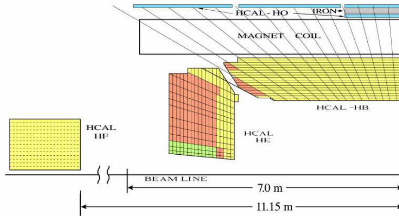
Figure 3.12: The CMS hadronic calorimeter. [56]
