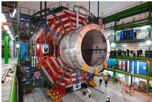
Figure 3.9: Installation of the superconducting solenoid in the CMS cavern. [56]
