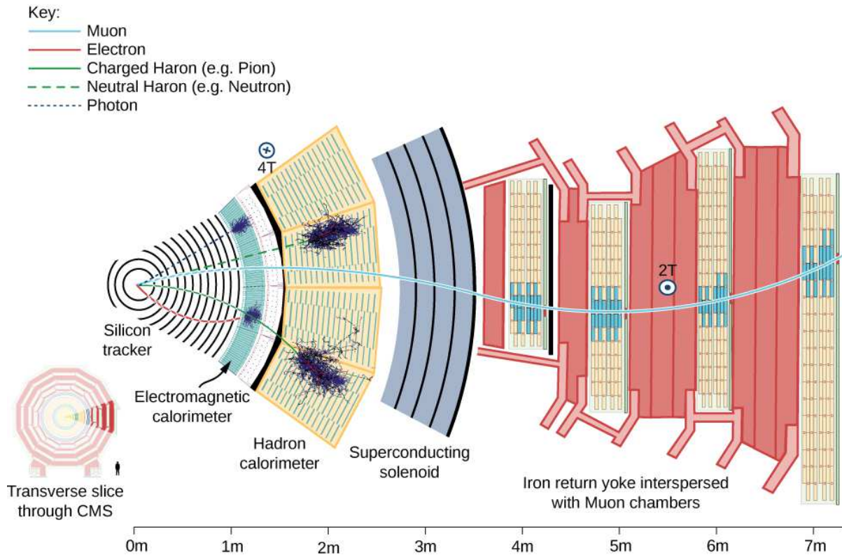
Figure 3.7: Mean path of a particle through the CMS detector. A muon, in light blue, passes through with a bended trajectory, depending on its momentum and charge, triggering signals in all the sub-systems. An electron, in red, leaves a track in the silicon tracker and is absorbed by the electromagnetic calorimeter. A neutral or charged hadron, in green, stops inside the hadronic calorimeter. A photon, dotted blue line, showers in the electromagnetic calorimeter, without leaving any track in the silicon detector. [56]
