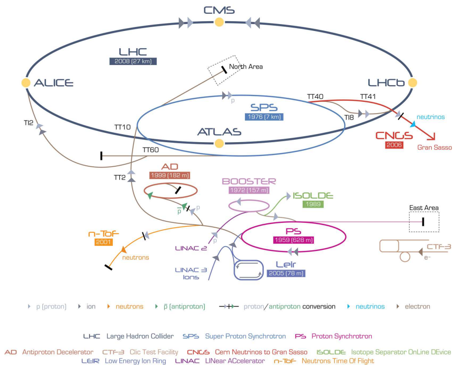
Figure 3.2: The CERN accelerator complex. [52]
