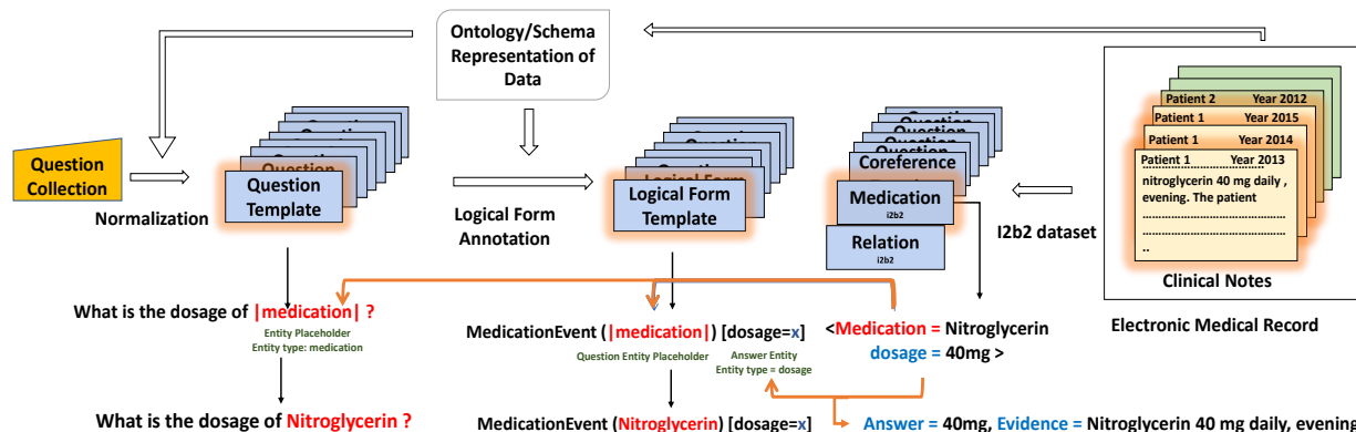
Figure 4.1: Our QA dataset generation framework using existing i2b2 annotations on a given patient’s record to generate a question, its logical form and answer evidence. The highlights in the figure show the annotations being used for this example.
