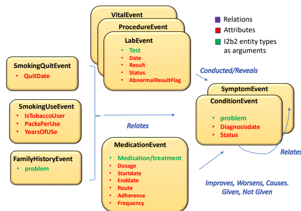
Figure 4.2: Events, attributes & relations in emrQA’s logical forms. Events & attributes accept i2b2 entities as arguments.
