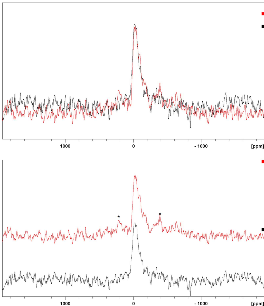
Fig. 7. (a) Overlaid 25 Mg MAS NMR spectra of unleached MW25 (black) and MgEM (red) glasses obtained at 52.05 MHz with 54,200 \pi/18 pulse and 0.1 s pulse delay and 102,400 \pi/18 pulses and 1.5 s pulse delay, respectively. The spinning speed is the same at 14 kHz. Spectra are referenced to 1 M MgCl 2 solution as 0 ppm; (b) the same spectra as shown in (a) stacked so that the spinning sidebands on MgEM spectrum can be seen (denoted by asterisks). (For interpretation of the references to colour in this figure legend, the reader is referred to the web version of this article.)
