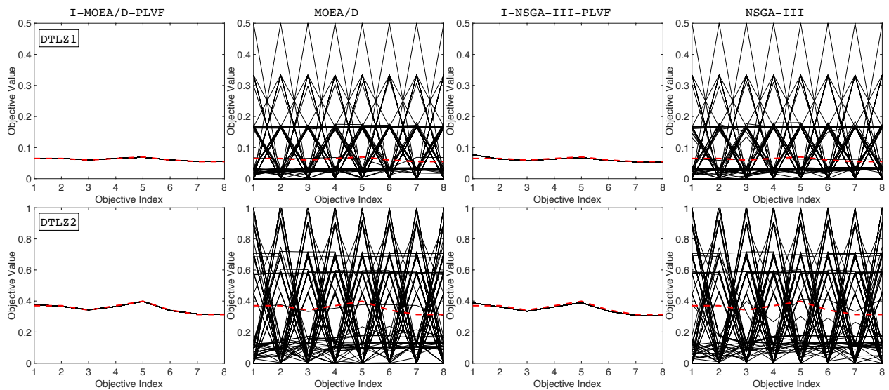
Figure 9: Solutions obtained on 8-objective DTLZ1 and DTLZ2 test problems where \mathbf{z}^r , which prefers the middle region of the PF, is represented as the red dotted line.
