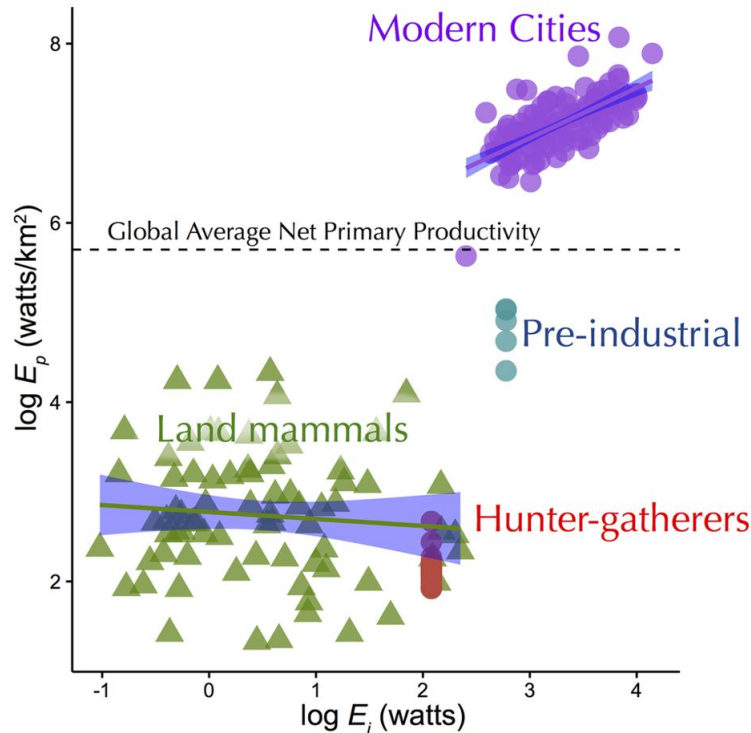
Figure 6: Red circles represent vegetarian hunter-gatherers (n=31), blue circles are pre-industrial societies (n=4), purple circles are modern cities (n=163), and green triangles are other herbivorous land mammal species (n=74). E_p is estimated as the product of density (individuals/km 2 ) and E_i (watts). Note that population energy use for herbivorous land mammals does not vary with individual energy use supporting theoretical expectations (slope=0), whereas urban cities increase (positive slope). The dashed line represents the terrestrial average net primary productivity for the planet from (15). Taken from (4) under http://creativecommons.org/licenses/by/4.0/
