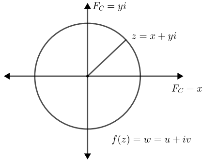
Fig. 8: Complex plane
