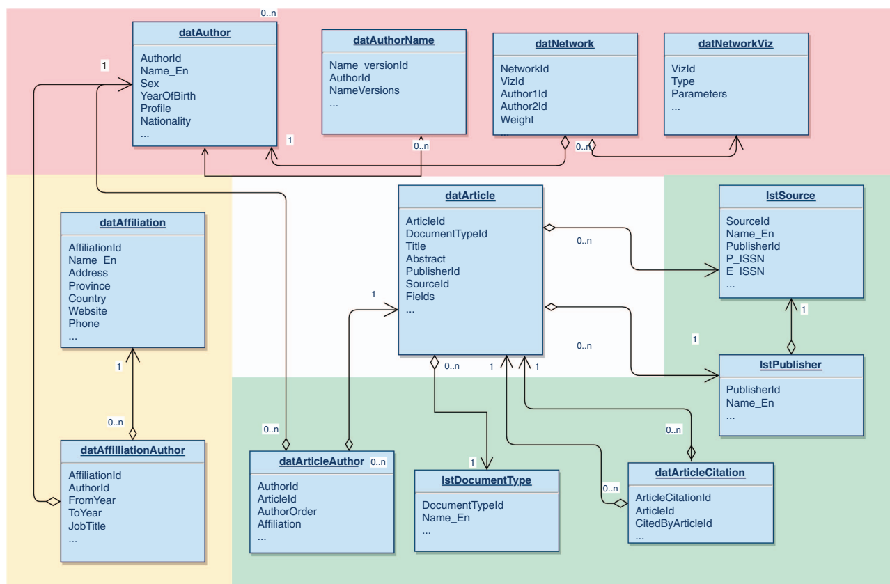
Figure 4. SSHPA's data structure diagram: relationships among authors, articles, affiliations, fields, sources, and publishers. These are four kinds of data in SSHPA system and they are related to each other through one fundamental unit— datArticle . The pink block contains boxes pertaining to the authors and their networks information. The green block contains boxes pertaining to the sources, publishers and articles information. The yellow block contains boxes pertaining to the authors' affiliations.
