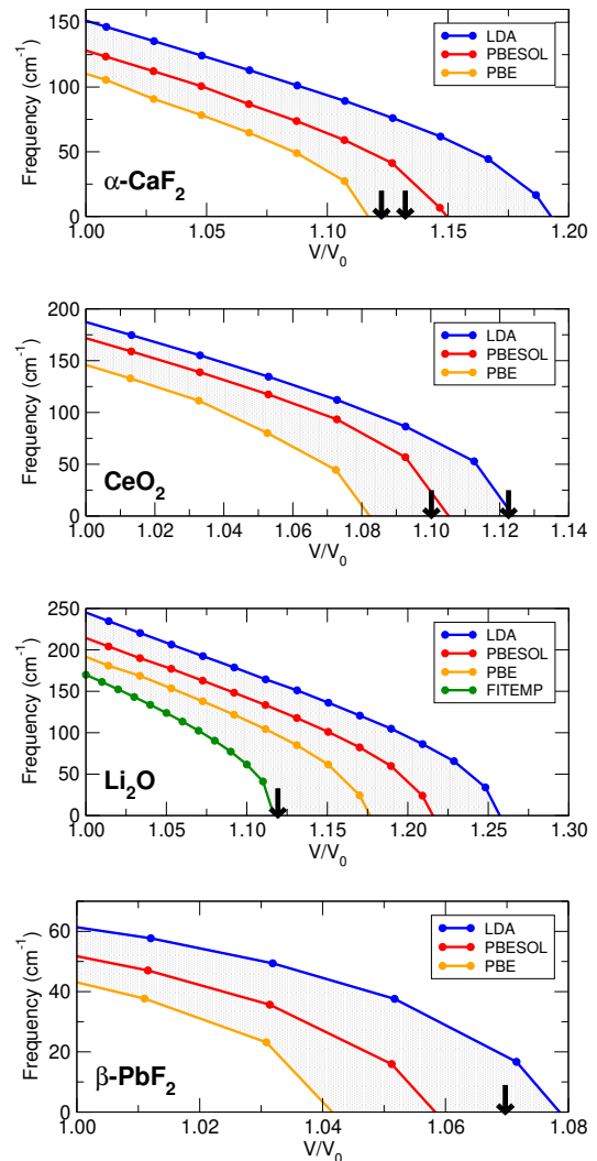
FIG. 8. Softening of the B_{1u} phonon mode in \alpha -CaF 2 , CeO 2 , and Li 2 O, and softening of the E_u phonon mode in \beta -PbF 2 with different exchange-correlation functionals. Frequencies \omega are given as a function of relative volume V/V_0 , where V_0 is the T = 0 K volume. Thick vertical arrows indicate V/V_0 derived from experimental results at the superionic phase transition; see the text for references.
