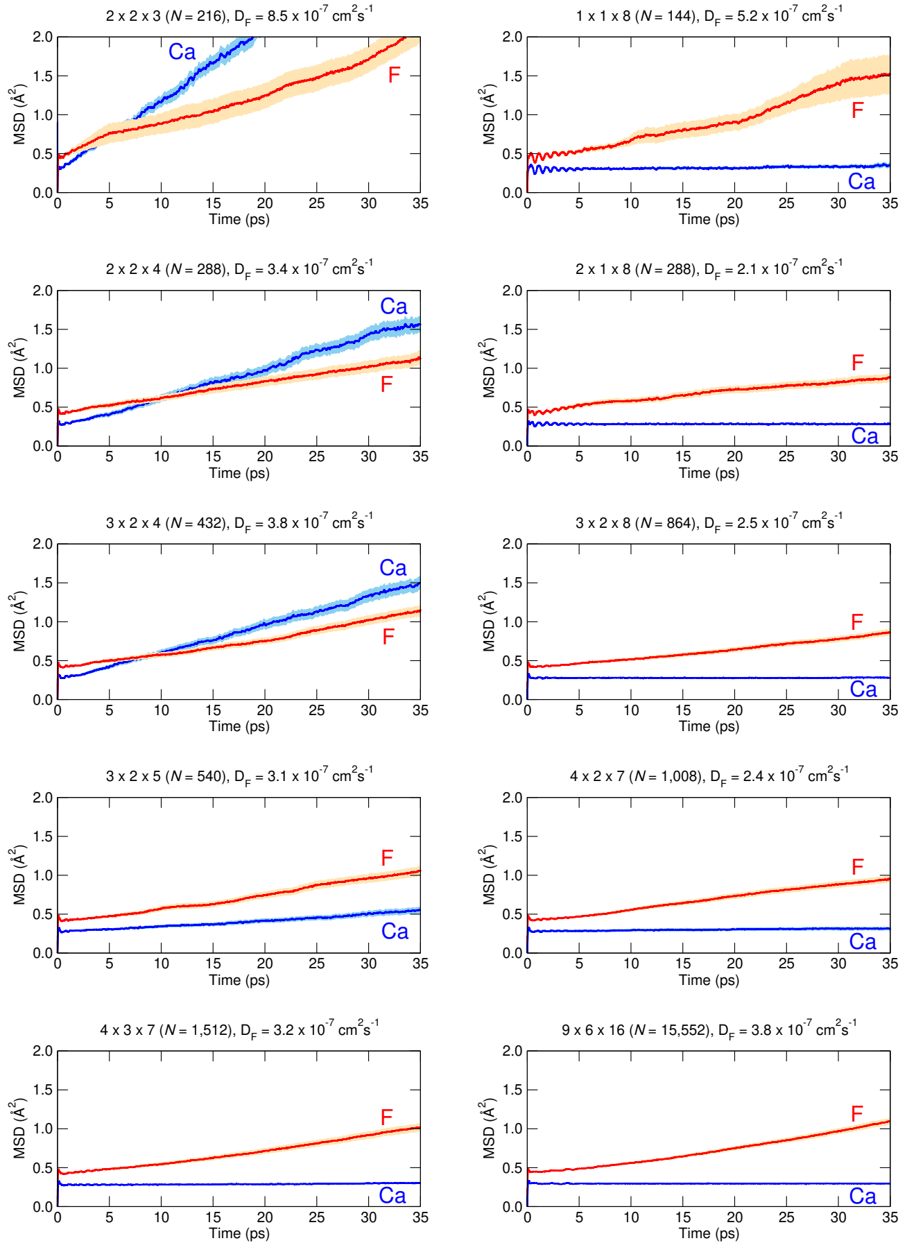
FIG. 9. Mean-squared displacements of Ca and F ions in P\bar{6}2m - \text{CaF}_2 at 2500 K and 20 GPa, for a variety of different simulation cell shapes and sizes.
