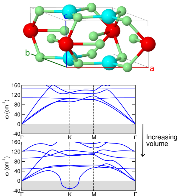
FIG. 1. (Top) The P\bar{6}2m -CaF 2 structure. Calcium atoms on the 1b Wyckoff site are in red, and those on the 2c site are in blue. Fluorine atoms are shown in green. (Bottom) Phonon dispersion relations in P\bar{6}2m -CaF 2 showing the softening of an acoustic mode at K at increasing volume (see Ref. [5]).
