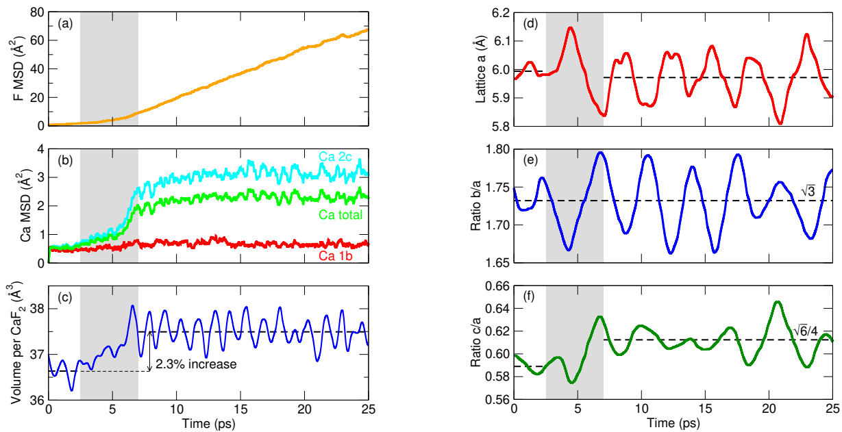
FIG. 4. Results of an 864-atom AIMD- NPT simulation at T = 2650 K and P = 20 GPa. (a) MSD for fluorine. (b) MSD for calcium, split into contributions from calcium ions on the 1b and 2c Wyckoff sites. (c) Evolution of the system volume. (d) Lattice parameter a for the hexagonal P\bar{6}2m cell. (e) Ratio of the b and a lattice lengths in the orthorhombically-set cell. (f) Ratio of the c and a lattice lengths.
