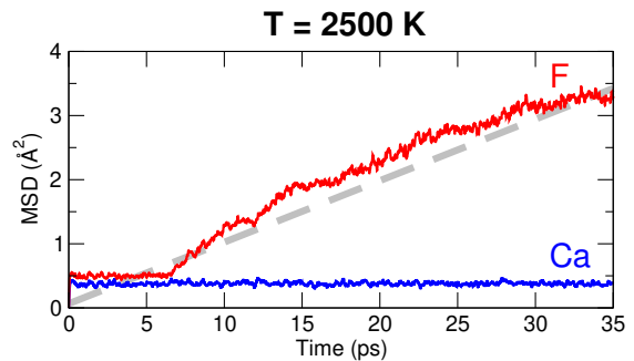
FIG. 3. MSD of F and Ca ions in P\bar{6}2m -CaF 2 in an 864-atom AIMD- NVT simulation at T = 2500 K. The pressure is P = 19.8 \pm 0.4 GPa. A best-fit line to the F MSD curve is shown by the thick dashed line.
