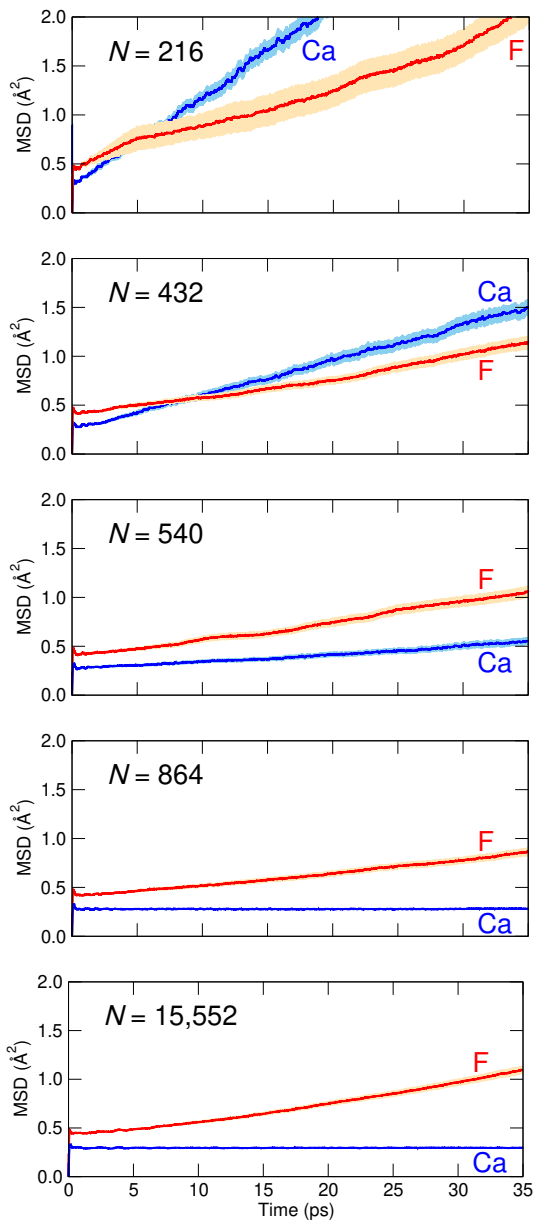
FIG. 2. Behaviour of the mean-square displacement of Ca and F ions in the P\bar{6}2m structure as a function of simulation cell size N at T = 2500 K and P = 20 GPa, from classical MD simulations. Light-blue and orange shaded regions indicate the uncertainty in the MSD for Ca and F respectively, obtained by averaging over multiple trajectories. Note that the uncertainties are small on the scale of the figures for N = 864 and N = 15,552 .
