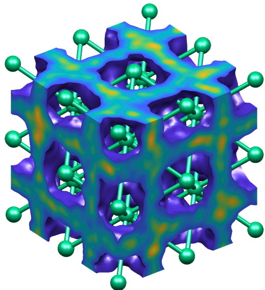
FIG. 7. Fluorine density isosurface for Im\bar{3}m -CaF 2 at 3000 K and 20 GPa, drawn at 1\times the mean fluorine density, which is 0.052 \text{ \AA}^{-3} . Yellow corresponds to high densities, and blue to low densities. Calcium ions are represented by pale blue spheres, and a 2 \times 2 \times 2 supercell of the conventional bcc unit cell is shown. The conventional lattice parameter is 4.24 Å.
