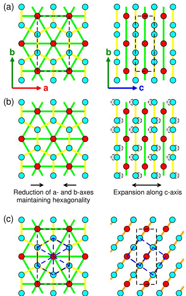
FIG. 5. Changes in the Ca sublattice in P\bar{6}2m -CaF 2 . Ca ions occupying the 1b Wyckoff site are shown in red, and those occupying the 2c site are in blue. Yellow and green lines link coplanar Ca ions, in planes perpendicular to the c -axis. Fluorine ions are not shown. (a). The pristine P\bar{6}2m structure, with black dashed lines showing the orthorhombic cell ( Z = 6 ). The hexagonal symmetry means that b/a = \sqrt{3} . (b). Increasing temperature results in volume expansion, largely along the c -axis, with a slight reduction in the a - and b -axes. Hexagonality is maintained in the a and b axes (i.e. b/a = \sqrt{3} ), and c/a increases to \sqrt{6}/4 . Ca ions on the 2c positions (blue) are displaced away from their sites and onto the sites shown in grey. (c). The resulting Ca sublattice is bcc. The orientation of the conventional bcc unit cell shown by blue dashed lines.
