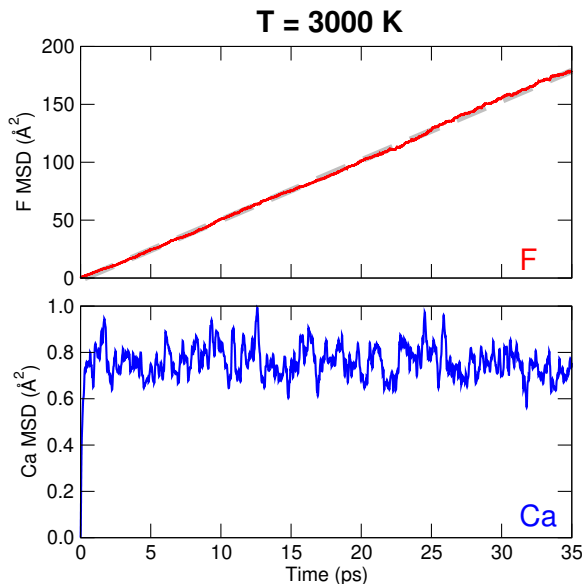
FIG. 6. MSD of F and Ca ions in P\bar{6}2m -CaF 2 in an 864-atom AIMD- NVT simulation at T = 3000 K. The pressure is P = 19.9 \pm 0.4 GPa. A best-fit line to the F MSD curve is shown by the thick dashed line.
