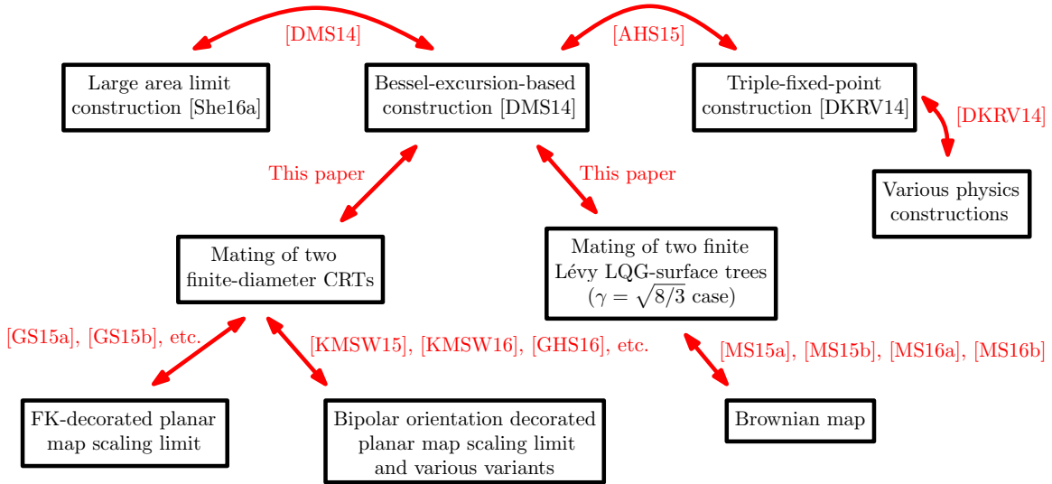
Figure 1.1: Several constructions of the Liouville quantum gravity sphere and their relationships. The boxes represent equivalent LQG-sphere definitions.
