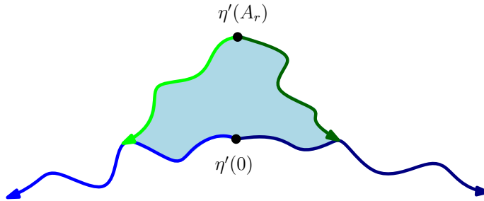
Figure 5.3: Illustration of the setup for the proof of Theorem 1.1 for \gamma \in (0, \sqrt{2}] and \kappa' \geq 8 . Shown is a space-filling \text{SLE}_{\kappa'} process \eta' on an \gamma -quantum cone parameterized by \mathbf{C} normalized so that \eta'(0) = 0 . The blue (resp. dark blue) path represents the left (resp. right) side of \eta' stopped at time 0 and the green (resp. dark green) show the left (resp. right) side of \eta' stopped at the time A_r up until merging with the blue (resp. dark blue) path. The light blue region is \eta'([0, A_r]) . The left/right boundary length process (L, R) is normalized so that L_0 = R_0 = 0 and L_{A_r} (resp. R_{A_r} ) is equal to the length of the green (resp. dark green) path minus the length of blue (resp. dark blue) path up until they merge and L_t, R_t are defined similarly for general t values. In particular, for t \in [0, A_r] , we have that L_t (resp. R_t ) is at least -1 times the length of the blue (resp. dark blue) path up until merging with the green (resp. dark green) path.
