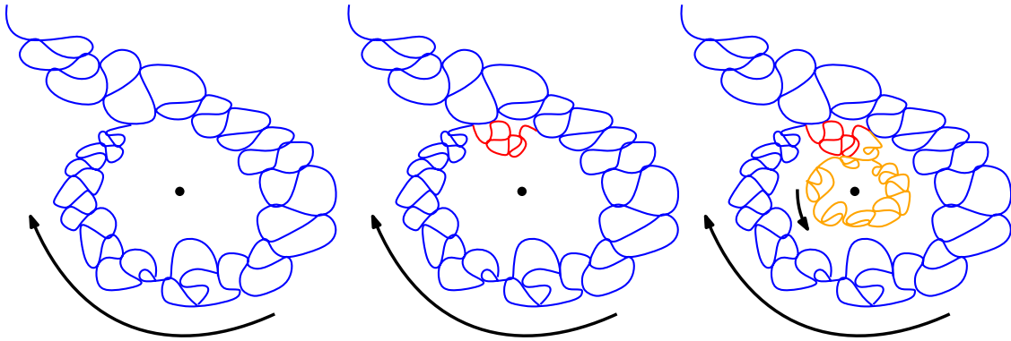
Figure 5.1: Left: A whole-plane \text{SLE}_{\kappa'}(\kappa' - 6) process from \infty to 0 stopped at a time that it has just closed a clockwise bubble around 0. The time-reversal of the associated space-filling \text{SLE}_{\kappa'} will enter this bubble and then fill it up before exiting, which is why it corresponds to a \pi/2 -cone excursion of the corresponding boundary length process. Middle: More of the \text{SLE}_{\kappa'}(\kappa' - 6) process is drawn. The component containing 0 is surrounded by one side of the \text{SLE}_{\kappa'}(\kappa' - 6) so again corresponds to a \pi/2 -cone excursion (which is nested inside the previous one). Right: The \text{SLE}_{\kappa'}(\kappa' - 6) drawn up until finishing the first bubble with a counterclockwise orientation after the time shown in the left panel. This bubble corresponds to an orientation changing \pi/2 -cone excursion.
