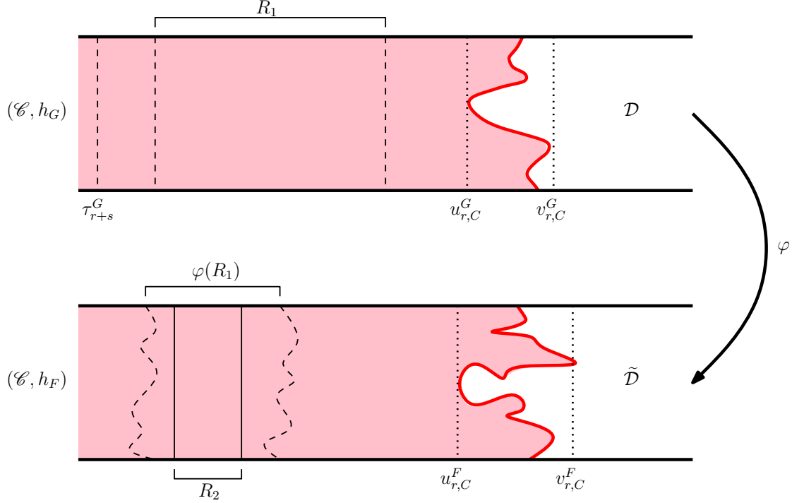
Figure 5.2: Illustration of the setup of the proof of Lemma 5.13. Top: a surface sampled from the law \mathfrak{m}_G . The red region is the part of the surface separated from +\infty up until the first time that the \text{SLE}_{\kappa'}(\kappa' - 6) process \tilde{\eta}' makes a loop with boundary length at most C^{-1}e^{\gamma r/2} . Bottom: the surface sampled from \mathfrak{m}_F after resampling \mathcal{D} to yield \tilde{\mathcal{D}} . The superscripts F and G are used to indicate quantities associated with h_F and h_G , respectively.
