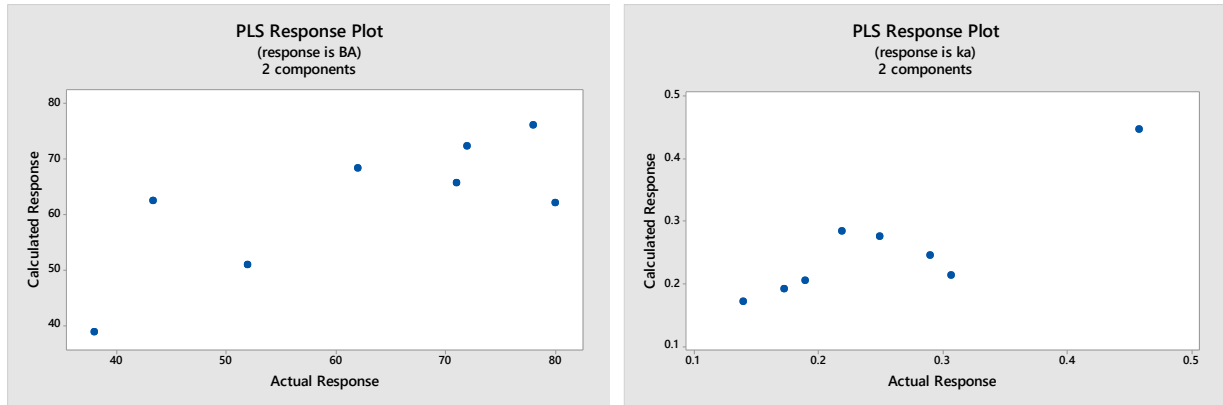
Supplementary Figure 3. PLS prediction of %BA and k_a with a , b and c .
