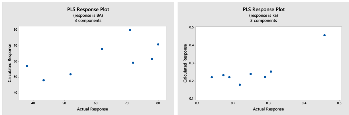
Supplementary Figure 2. PLS prediction of %BA and k_a with molecule and formulation properties.
