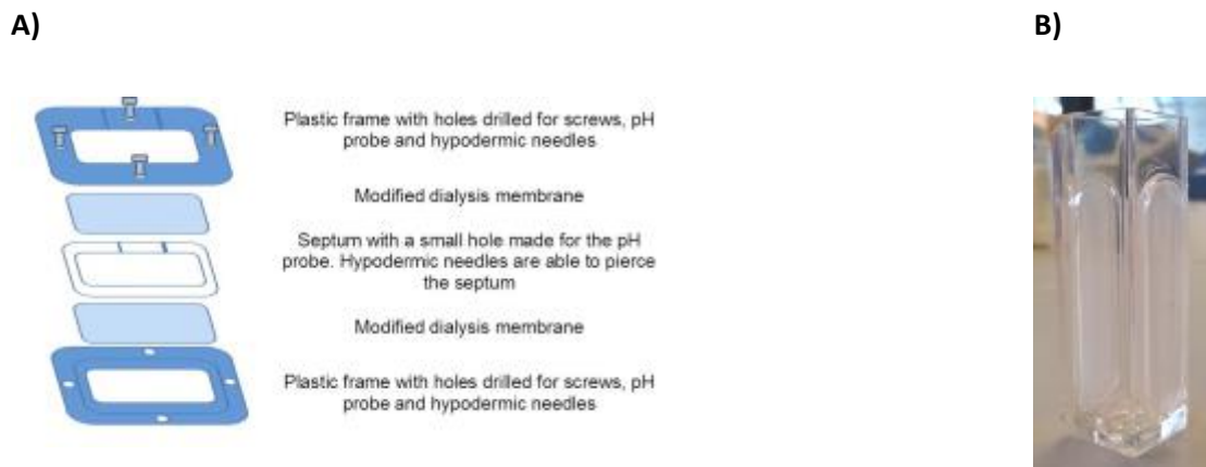
Supplementary Figure 4. Comparison of injection site compartments used in Scissor. A) Organization of the dialysis cassette used in the prototype system. A 3 mL Slide-A-Lyzer dialysis cassette, 0.60 x 6.3 x 2.5 cm, was modified as highlighted by the schematic. B) A 4.5 mL cuvette, 1 x 1 x 5 cm, cartridge used in the commercial system.
