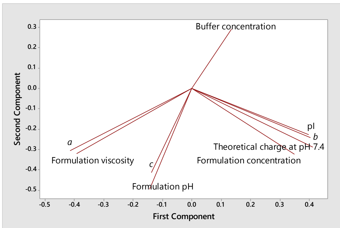
1 2 Figure 3. Loading plot of the two first components describing the relationships between input 3 parameters for the set of monoclonal antibodies tested in the Scissor system.
