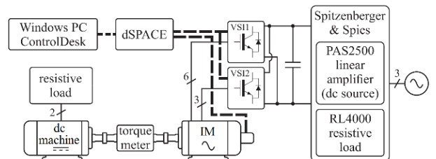
Fig. 14. Experimental rig and its electrical scheme.
