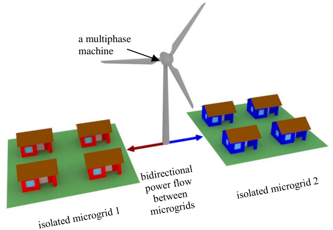
Fig. 1. A single multiphase machine can be used for power transfer from one microgrid to another. The microgrids are mutually isolated.
