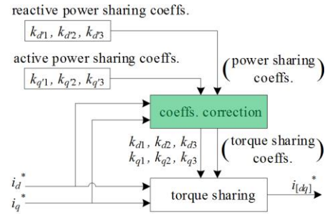
Fig. 11. “Power sharing” block from Fig. 9 (a nine-phase IM is assumed, so that there are three coefficients). The block “coeffs. correction” is the only difference from the standard torque sharing algorithm (e.g. [15]).
