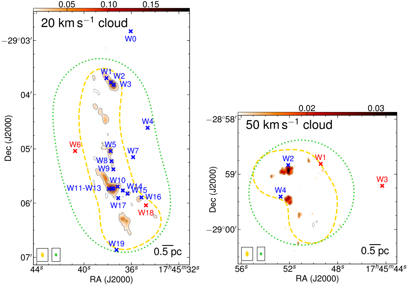
Figure 4. VLA \text{H}_2\text{O} masers in the six clouds. The background images and contours show the SMA 1.3 mm continuum emission, and the dashed and dotted loops show the mosaic field of the SMA and VLA, which are identical to those in Figure 3. \text{H}_2\text{O} masers are marked by crosses, among which red ones are those with AGB star counterparts.
