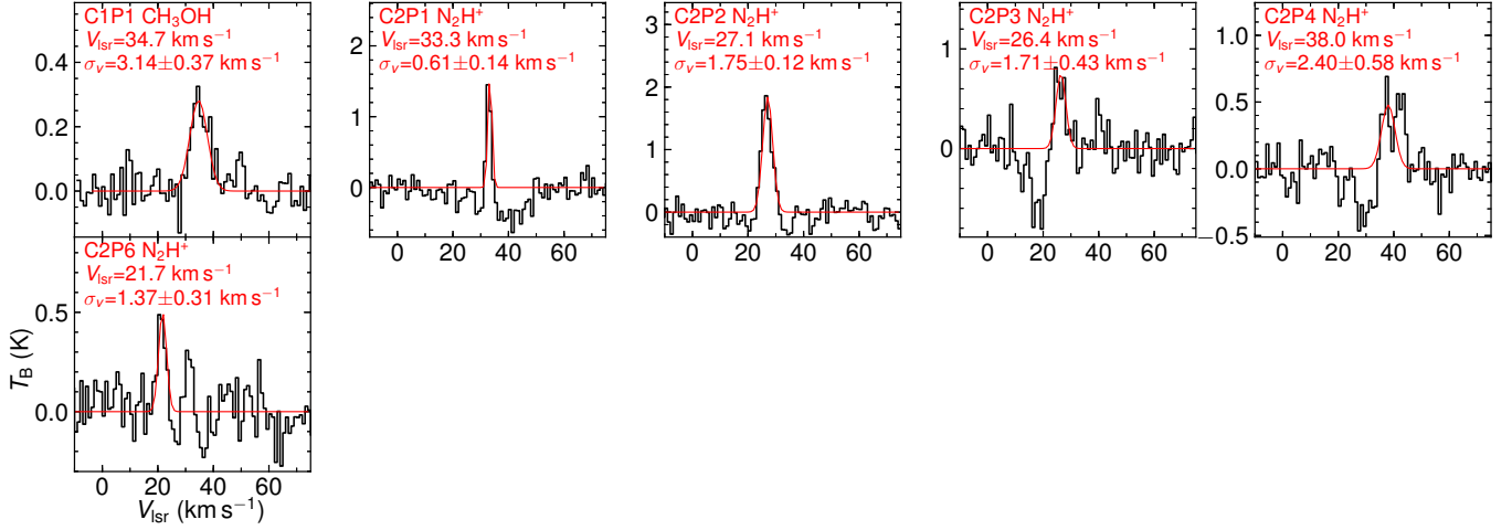
Figure 17. The SMA N 2 H + or CH 3 OH spectra and best-fit models of cores in Sgr B1-off. The best-fit line widths (deconvolved from channel width) are noted in each panel.
