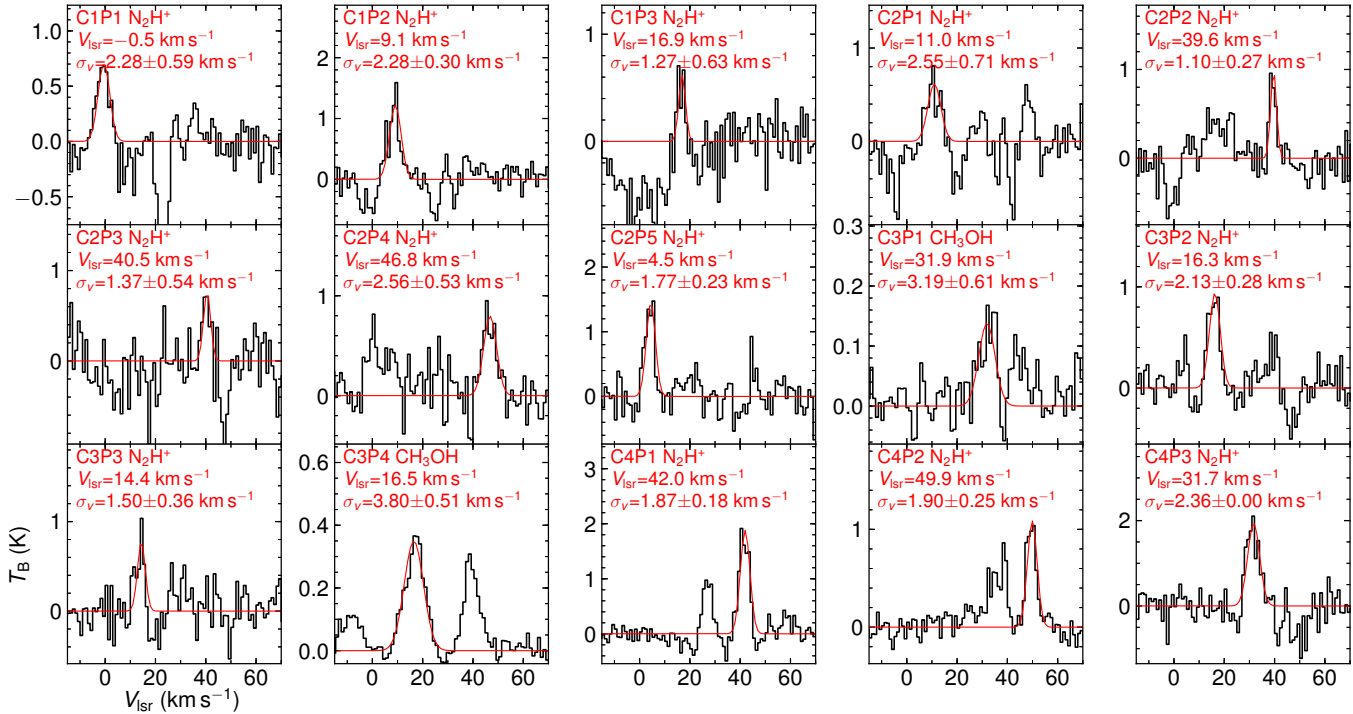
Figure 16. The SMA N 2 H + or CH 3 OH spectra and best-fit models of cores in G0.253+0.016. The best-fit line widths (deconvolved from channel width) are noted in each panel.
