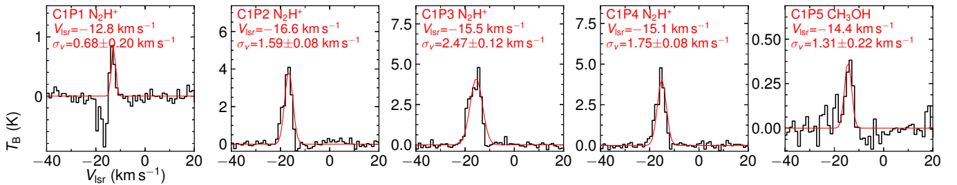
Figure 19. The SMA N 2 H + or CH 3 OH spectra and best-fit models of cores in Sgr D. The best-fit line widths (deconvolved from channel width) are noted in each panel.
