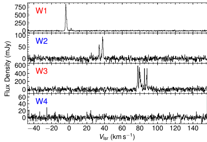
Figure 9. H 2 O maser spectra in the 50 km s -1 cloud detected by the VLA.
