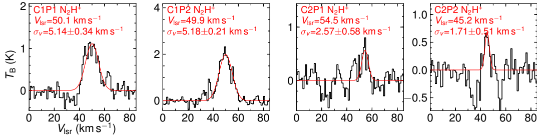
Figure 15. The SMA N 2 H + spectra and best-fit models of cores in the 50 km s -1 cloud. The best-fit line widths (deconvolved from channel width) are noted in each panel.
