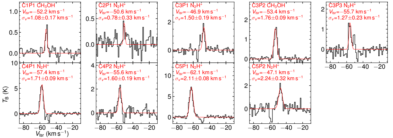
Figure 18. The SMA N 2 H + or CH 3 OH spectra and best-fit models of cores in Sgr C. The best-fit line widths (deconvolved from channel width) are noted in each panel.
