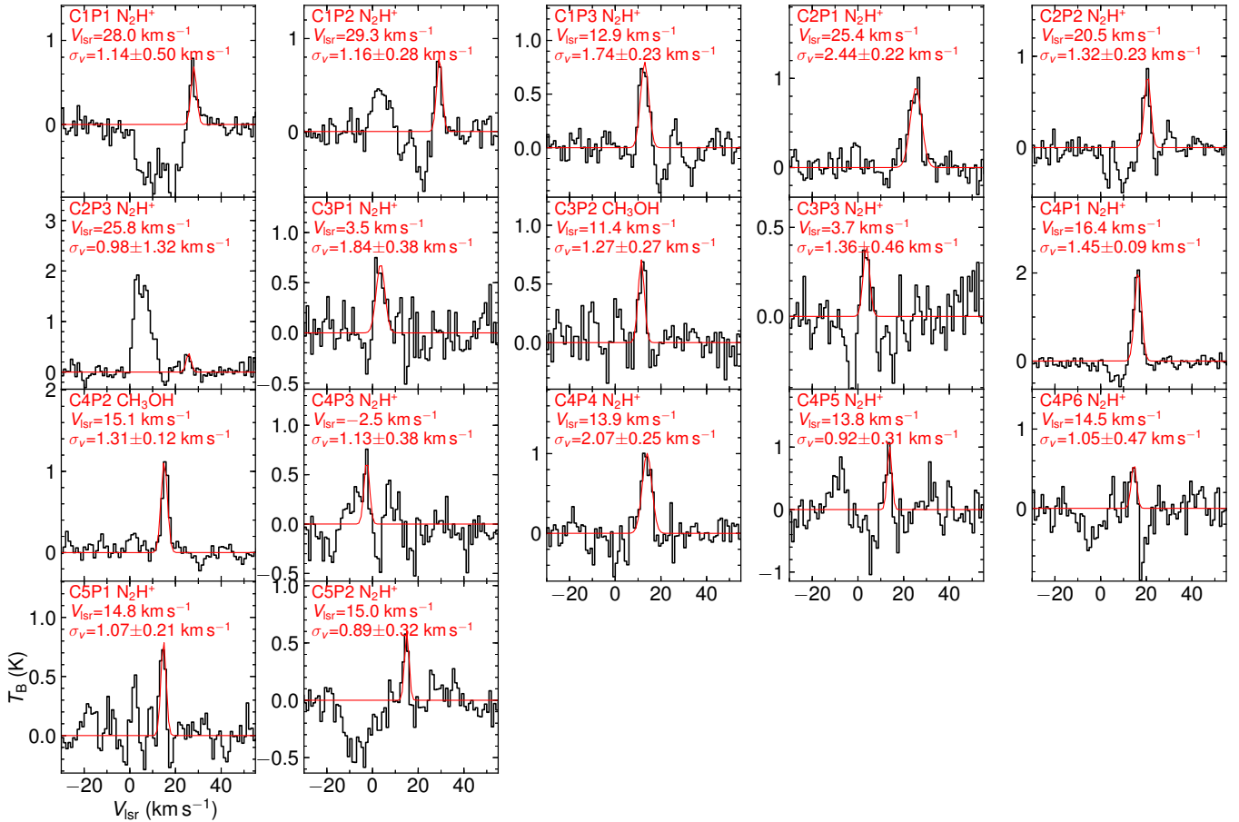
Figure 14. The SMA N 2 H + or CH 3 OH spectra and best-fit models of cores in the 20 km s -1 cloud. The best-fit centroid velocities ( V_{\text{sr}} ) and line widths ( \sigma_v , deconvolved from channel width) are noted in each panel.
