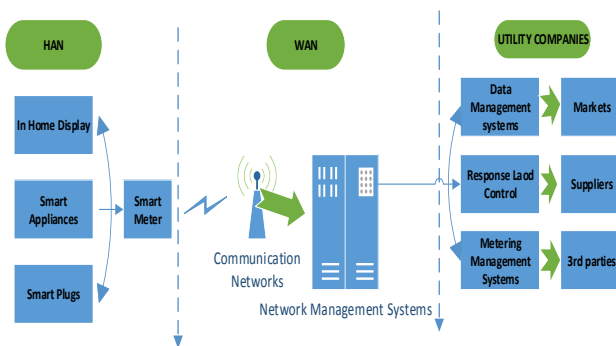
Figure I. Advanced Metering Infrastructure
