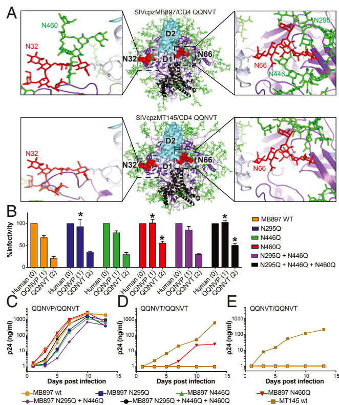
Fig. 5. Steric hindrance between CD4- and SIVcpz Env-encoded glycans. (A) A model of two SIVcpz Envs (Top, MB897; Bottom, MT145) in complex with the chimpanzee CD4 QQNVT variant (containing both N32 and N66 glycans) is shown. Env residues are shown in purple, Env glycans in green, and CD4 glycans in red. (B) Infectivity of WT and mutant MB897 Envs lacking the indicated glycans in cells expressing different CD4 alleles (parentheses indicate the number of D1 domain glycans). Asterisks denote significant enhancement of the mutant Envs relative to the MB897 WT (orange) for that particular allele. (C-E) Replication of wild-type and mutant MB897 viruses in CD4 + T cells from one heterozygous chimpanzee encoding QQNVP and QQNVT alleles (C) and two homozygous chimpanzees encoding the QQNVT allele (D and E).
