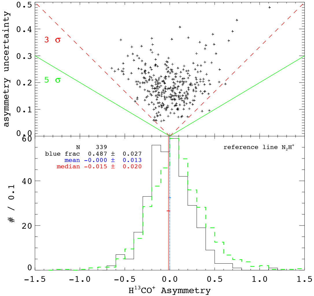
Figure 3. The asymmetry parameter A for H^{13}CO^+ , with N_2H^+ as the reference line. The upper panel shows the asymmetries on the x-axis and the 1\sigma uncertainty in the asymmetry on the y-axis. Points lying below the dashed red and solid green lines have an asymmetry value that is at least three or five times its uncertainty respectively. The lower panel shows a histogram of the asymmetry. The vertical red and blue lines and text denote the median and mean of the distribution; the horizontal red and blue lines indicate the \pm 1\sigma uncertainties in the median and mean. The distribution of A for HCO^+ , normalized to have the same peak, is superposed in green. Note the clear shift to more positive values for HCO^+ . A K-S test gives a probability of 9 \times 10^{-5} that these two distributions were drawn from the same parent population.
