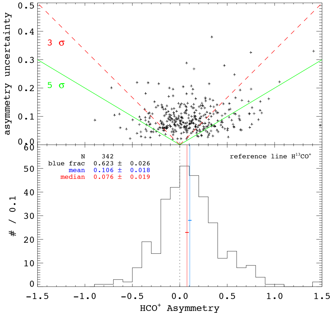
Figure 4. The asymmetry parameter A for HCO + , with H 13 CO + as the reference line. The upper panel shows the asymmetries on the x-axis and the 1\sigma uncertainty in the asymmetry on the y-axis. Points lying below the dashed red and solid green lines have an asymmetry value that is at least three or five times its uncertainty respectively. The lower panel shows a histogram of the asymmetry. The vertical red and blue lines and text denote the median and mean of the distribution; the horizontal red and blue lines indicate the \pm 1\sigma uncertainties in the median and mean.
