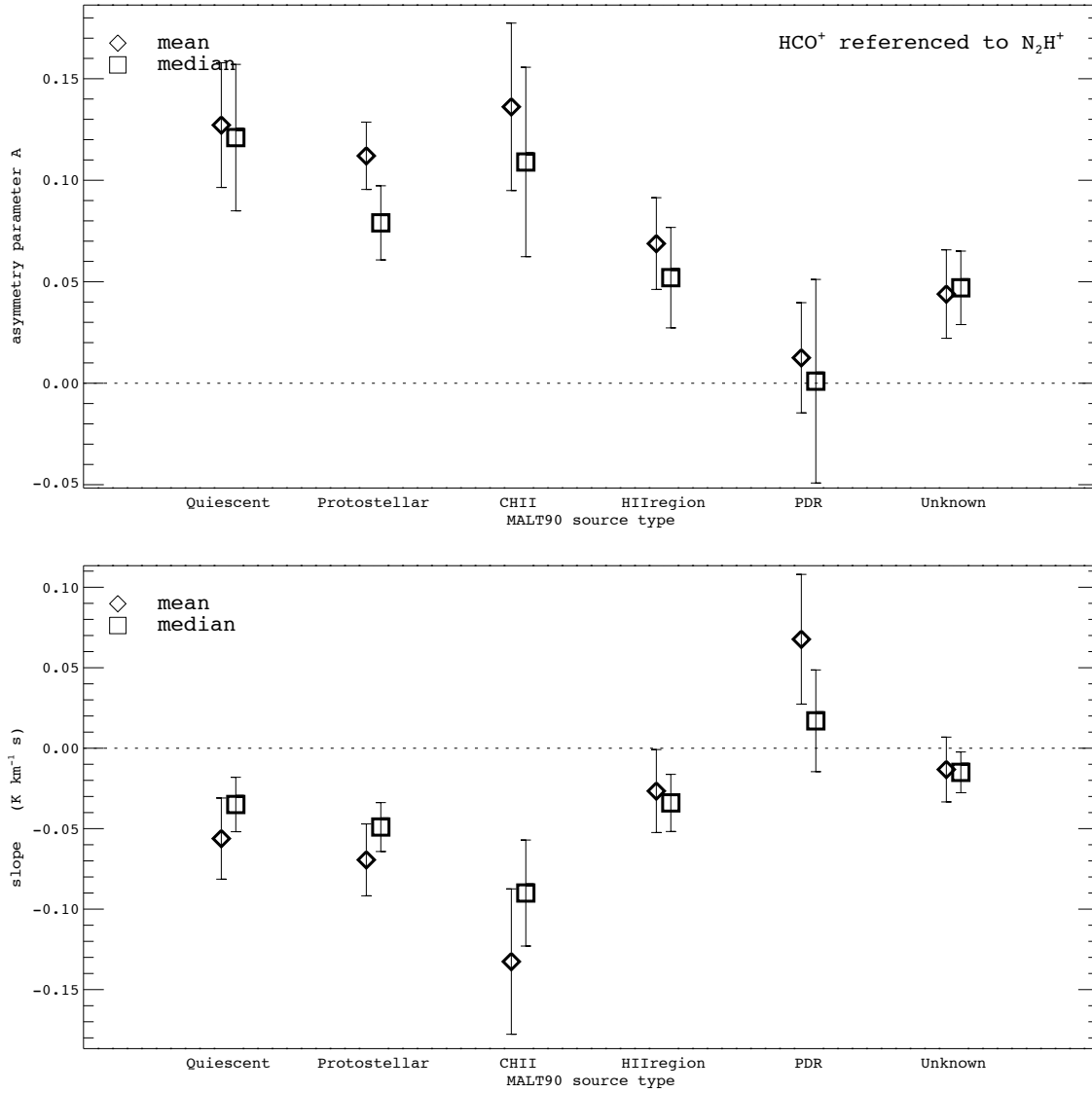
Figure 11. The mean and median \text{HCO}^+ asymmetries and line slopes plotted versus the IR classification.
