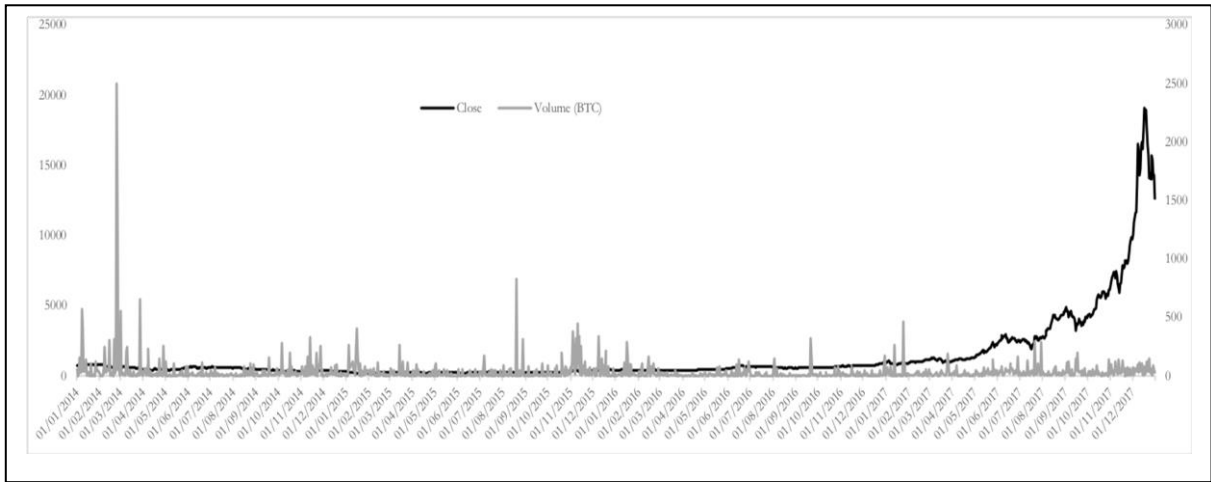
Figure 1: Time-series graph of the price of Bitstamp on the primary y-axis and volume on the secondary y-axis.
