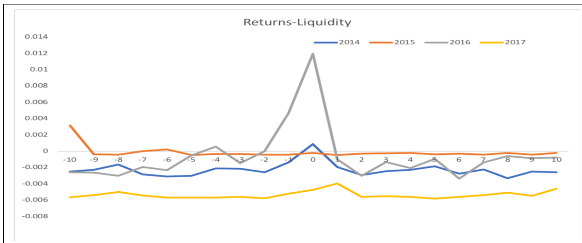
Figure 8: The cross-correlation between Bitcoin volume and liquidity over four subsample periods for different lead and lag intervals.
