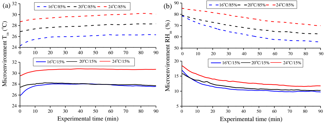
Figure 3 Changes in mean T_{in} and RH_{in} in inner clothing environment over time
