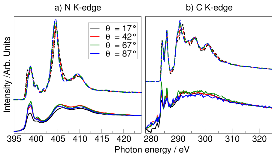
Figure 8: Comparison of experimental and computational spectra for the a) N K-edge and b) C K-edge for high coverage BTA adsorption at 300 K. Experimental data are shown as solid lines. The computational spectra (dashed lines) are those for a mixture of 30% low coverage chains (Fig. 2b) and 70% dimers (Fig. 2c). The angle \theta refers to the angle between the X-ray polarization vector and the surface normal (see Fig. 1).
