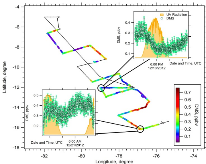
Fig. 5.16 M91 ship track for a portion of the cruise colored by atmospheric DMS measurements. The inset figure shows DMS measurements during one 24-hour station, the location of which is indicated by the large black circle.
