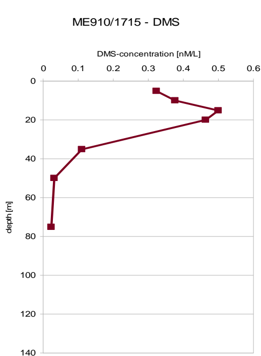
Fig. 5.8-1: DMS depth profile at M910/1715
