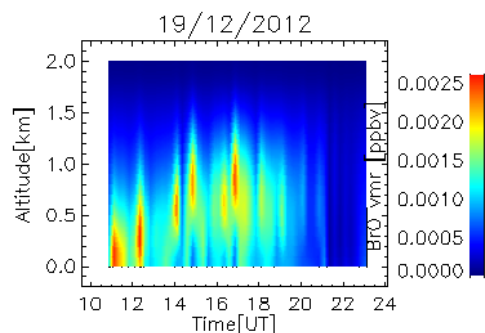
Fig. 5.17-3 Preliminary BrO profiles from MAX-DOAS measurements on 19 Dec 2012.
