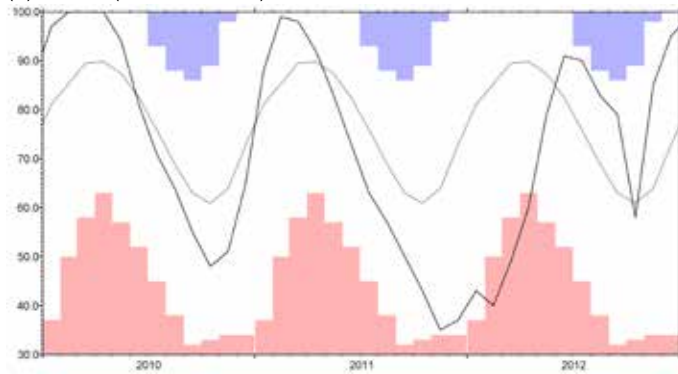
Figure 15 Reservoir stocks (% of capacity)
