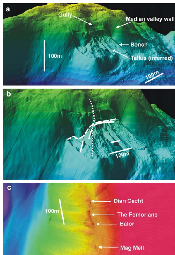
Figure 5. (a) Multibeam echosounder bathymetry of the Moytirra vent field setting. Moytirra is imaged in higher resolution and sits on a bench at the base of a steep median valley wall fault scarp with ridges of assumed tallus extending down-slope. (b) Close up of the vent field showing major lineations. Chimneys are aligned (solid line) parallel to the boundary fault (dashed line). They occur at the intersection of an other fault marking a gully in the headwall (dotted line) (c) Plan view showing the named chimney clusters in close alignment.
