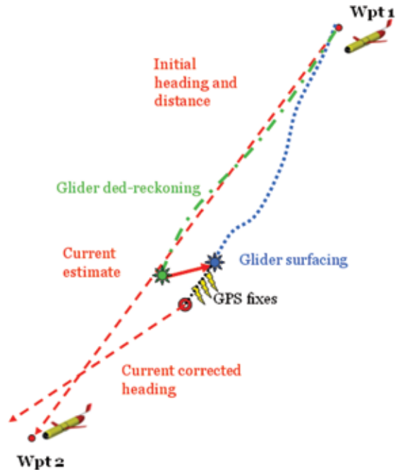
Figure 3: The glider navigates using ded-reckoning. The green line represents the ded-reckoned path while the blue line depicts the actual path. When the glider surfaces, it uses an estimate of the depth-averaged currents over the past yo, combined with surface drift, estimated from the GPS, to determine its next heading.
