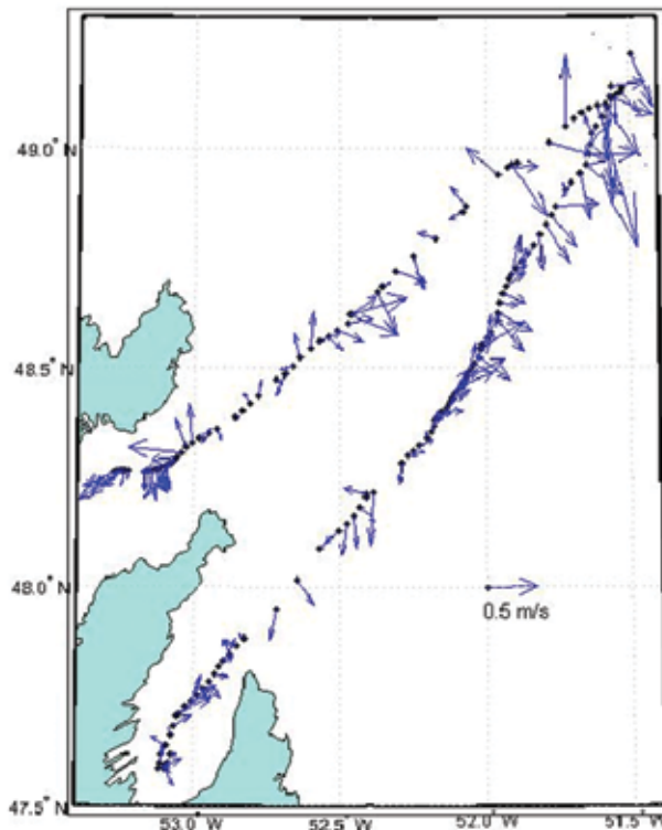
Figure 4: Examples of surface currents computed from GPS fixes while the Slocum is transmitting data. The largest velocities correspond to where the glider crossed the inner branch of the Labrador current.
