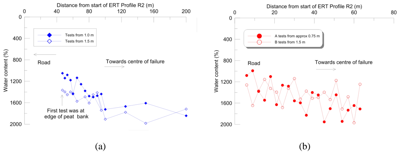
Figure 13. Longitudinal profiles of water content (a) Carn Park and (b) Roosky
