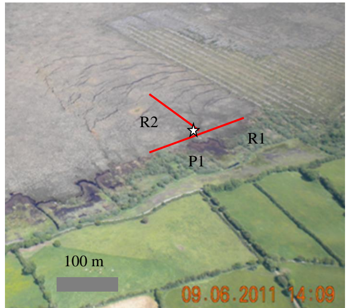
Figure 3. Southern failed area at Carn Park bog (a) from 2005 aerial photograph (courtesy Charise Mc Keown - Geological Survey of Ireland) and (b) Section of 2011 ortho rectified photograph of Carn Park bog (courtesy Andrea Webb, National Parks and Wildlife Services). R1 and R2 represent the ERT profiles and P1 the deep peat probe
