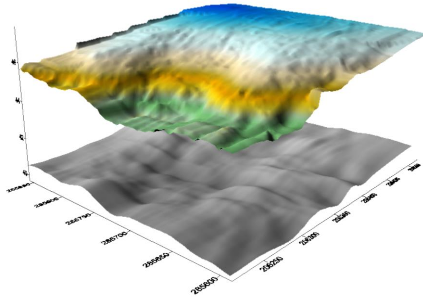
Figure 9. (a) peat thickness and (b) 3D plot of surface and peat base topography for Aghnamona bog, Roosky. (East and north co-ordinates and elevation are given in m).
