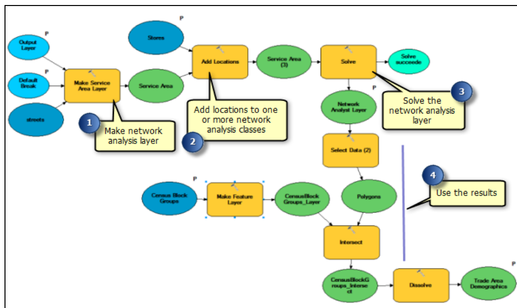
Figure 7: Model Builder for automating iterative processes
