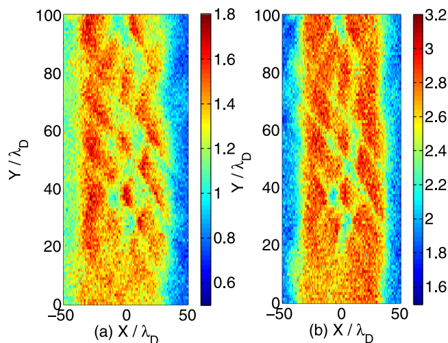
FIG. 14. The ion density distributions in a section of the 2D simulation box at the time t\omega_{pi} = 72 . Panel (a) shows the distribution of the ion beam that moves to increasing values of x . Panel (b) shows the total ion density (enhanced online) [URL: http://dx.doi.org/10.1063/1.4825339.3 ].
