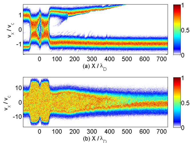
FIG. 4. The phase space distributions f_{i.e}(x, v_x) from the 1D simulation at the time t\omega_{pi} = 86 : Panel (a) shows the ion distribution and panel (b) shows the electron distribution. Space and velocity are expressed in units of the Debye length \lambda_D and of the initial cloud speed v_c . The density is normalized to its peak value and displayed on a linear color scale (enhanced online) [URL: http://dx.doi.org/10.1063/1.4825339.1 ].
