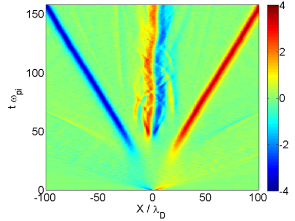
FIG. 2. The spatio-temporal electric field distribution in the 1D simulation: The color corresponds to 10^3 E_x , space is given in units of the electron Debye length \lambda_D and time is normalized to the ion plasma frequency \omega_{pi} .
